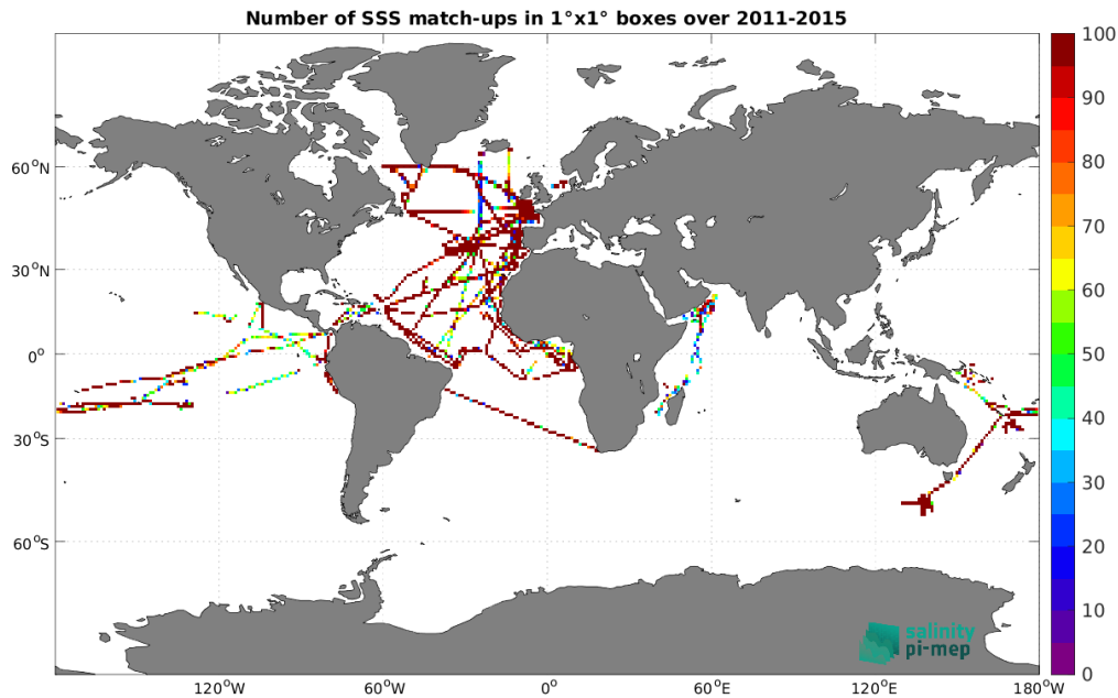
Figure 5: Number of SSS match-ups between TSG (GOSUD-Research-vessel) SSS and the Aquarius SSS L3 CAP v5 - 7-Day running (JPL) SSS product for the Global Ocean Pi-MEP region over 1^\circ \times 1^\circ boxes and for the full satellite product period.
