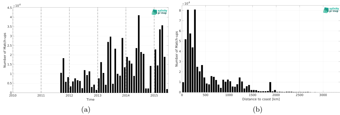
Figure 2: Number of match-ups between TSG (GOSUD-Research-vessel) and Aquarius SSS L3 CAP v5 - 7-Day running (JPL) SSS as a function of time (a) and as function of the distance to coast (b) over the Global Ocean Pi-MEP region and for the full satellite product period.
