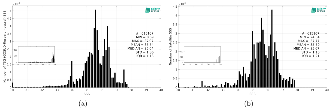
Figure 3: Histograms of SSS from TSG (GOSUD-Research-vessel) (a) and Aquarius SSS L3 CAP v5 - 7-Day running (JPL) (b) considering all match-up pairs per bins of 0.1 over the Global Ocean Pi-MEP region and for the full satellite product period.
