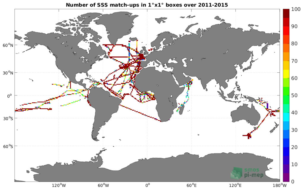
Figure 4: Number of SSS match-ups between TSG (GOSUD-Research-vessel) SSS and the Aquarius SSS L3 CAP v5 - 7-Day running (JPL) SSS product for the Global Ocean Pi-MEP region over 1^\circ \times 1^\circ boxes and for the full satellite product period.
