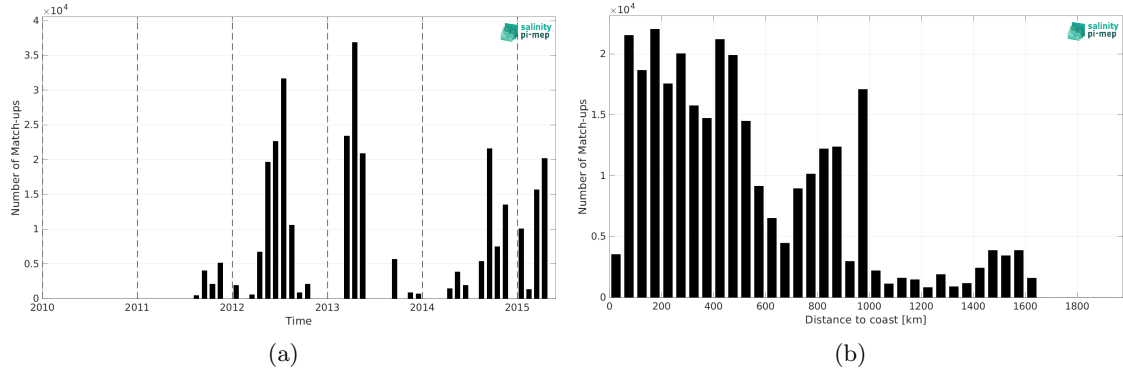
Figure 2: Number of match-ups between TSG (CSIC-UTM) and Aquarius SSS L3 CAP v5 - 7-Day running (JPL) SSS as a function of time (a) and as function of the distance to coast (b) over the Global Ocean Pi-MEP region and for the full satellite product period.
