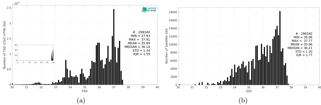
Figure 3: Histograms of SSS from TSG (CSIC-UTM) (a) and Aquarius SSS L3 CAP v5 - 7-Day running (JPL) (b) considering all match-up pairs per bins of 0.1 over the Global Ocean Pi-MEP region and for the full satellite product period.
