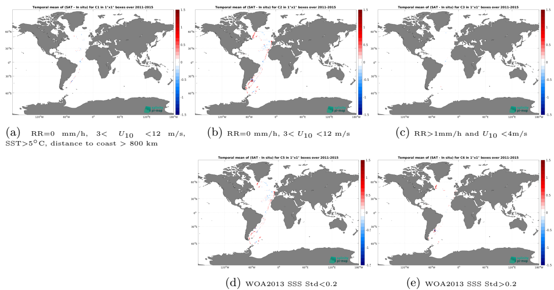
Figure 14: Temporal mean gridded over spatial boxes of size 1^\circ \times 1^\circ of \Delta SSS (Aquarius SSS L3 CAP v5 - 7-Day running (JPL) - TSG (CSIC-UTM)) for 5 different subdatasets corresponding to: RR=0 mm/h, 3 < U_{10} < 12 m/s, SST > 5^\circ\text{C} , distance to coast > 800 km (a), RR=0 mm/h, 3 < U_{10} < 12 m/s (b), RR > 1 mm/h and U_{10} < 4 m/s (c), WOA2013 SSS Std < 0.2 (d), WOA2013 SSS Std > 0.2 (e).
