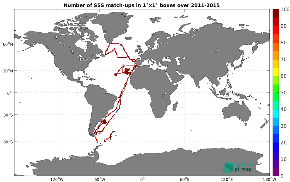
Figure 5: Number of SSS match-ups between TSG (CSIC-UTM) SSS and the Aquarius SSS L3 CAP v5 - 7-Day running (JPL) SSS product for the Global Ocean Pi-MEP region over 1^\circ \times 1^\circ boxes and for the full satellite product period.
