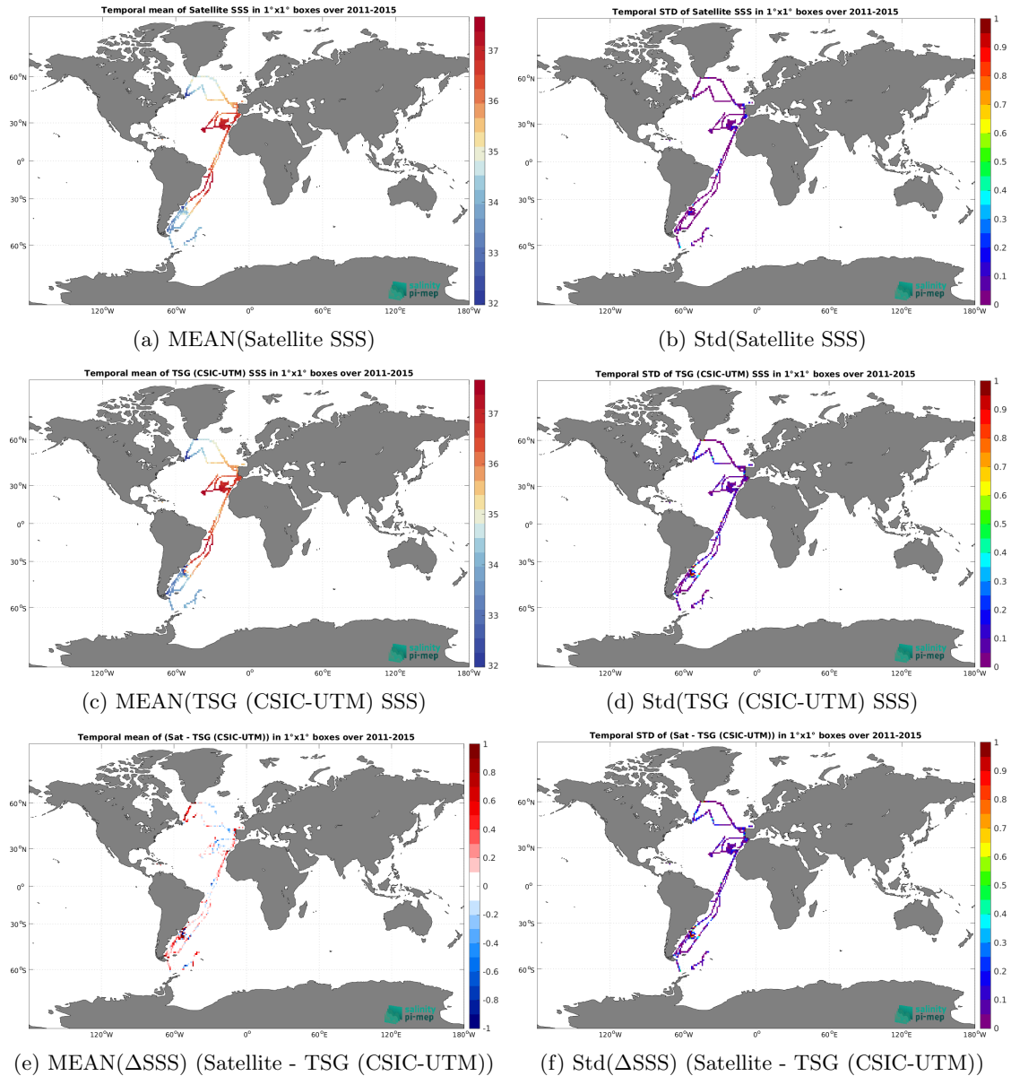
Figure 6: Temporal mean (left) and Std (right) of SSS from Aquarius SSS L3 CAP v5 - 7-Day running (JPL) (top), TSG (CSIC-UTM) (middle), and of \Delta SSS (Satellite - TSG (CSIC-UTM)). Only match-up pairs are used to generate these maps.
