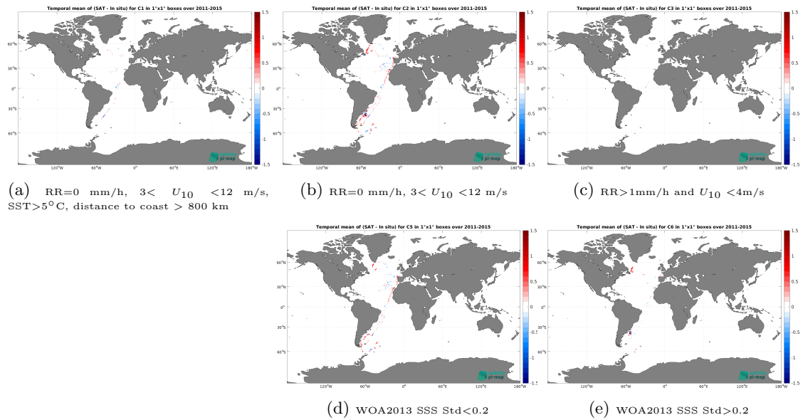
Figure 12: Temporal mean gridded over spatial boxes of size 1^\circ \times 1^\circ of \Delta SSS (Aquarius SSS L3 CAP v5 - 7-Day running (JPL) - TSG (CSIC-UTM)) for 5 different subdatasets corresponding to:RR=0 mm/h, 3 < U_{10} < 12 m/s, SST >5^\circ C, distance to coast > 800 km (a), RR=0 mm/h, 3 < U_{10} < 12 m/s (b), RR >1 mm/h and U_{10} < 4 m/s (c), WOA2013 SSS Std <0.2 (d), WOA2013 SSS Std >0.2 (e).
