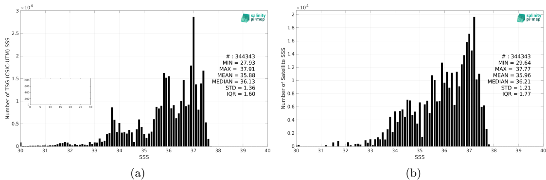
Figure 2: Histograms of SSS from TSG (CSIC-UTM) (a) and Aquarius SSS L3 CAP v5 - 7-Day running (JPL) (b) considering all match-up pairs per bins of 0.1 over the Global Ocean Pi-MEP region and for the full satellite product period.
