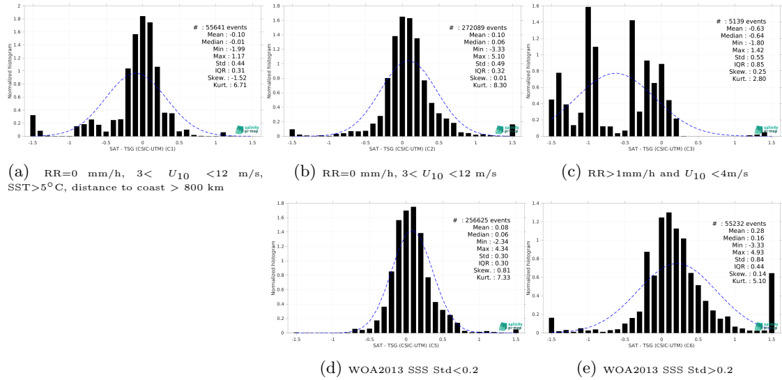
Figure 13: Normalized histogram of \Delta SSS (Aquarius SSS L3 CAP v5 - 7-Day running (JPL) - TSG (CSIC-UTM)) for 5 different subdatasets corresponding to: RR=0 mm/h, 3 < U_{10} < 12 m/s, SST>5°C, distance to coast > 800 km (a), RR=0 mm/h, 3 < U_{10} < 12 m/s (b), RR>1mm/h and U_{10} < 4 m/s (c), WOA2013 SSS Std<0.2 (d), WOA2013 SSS Std>0.2 (e).
