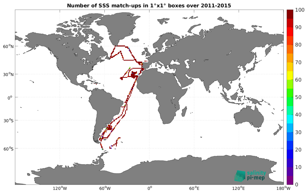
Figure 4: Number of SSS match-ups between TSG (CSIC-UTM) SSS and the Aquarius SSS L3 CAP v5 - 7-Day running (JPL) SSS product for the Global Ocean Pi-MEP region over 1^\circ \times 1^\circ boxes and for the full satellite product period.
