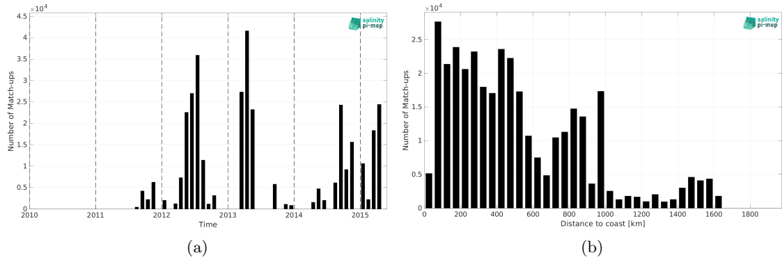
Figure 1: Number of match-ups between TSG (CSIC-UTM) and Aquarius SSS L3 CAP v5 - 7-Day running (JPL) SSS as a function of time (a) and as function of the distance to coast (b) over the Global Ocean Pi-MEP region and for the full satellite product period.
