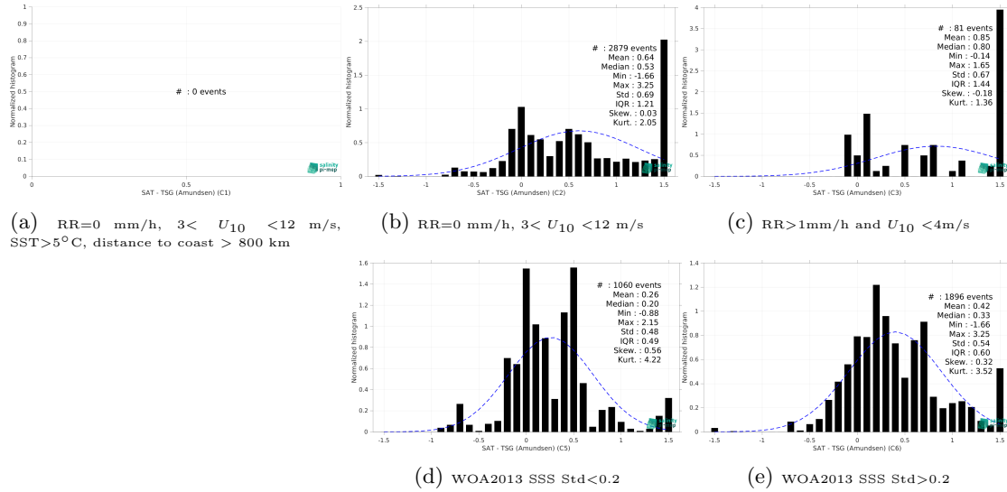
Figure 15: Normalized histogram of \Delta SSS (Aquarius SSS L3 CAP v5 - 7-Day running (JPL) - TSG (Amundsen)) for 5 different subdatasets corresponding to: RR=0 mm/h, 3 < U_{10} < 12 m/s, SST > 5°C, distance to coast > 800 km (a), RR=0 mm/h, 3 < U_{10} < 12 m/s (b), RR > 1mm/h and U_{10} < 4 m/s (c), WOA2013 SSS Std < 0.2 (d), WOA2013 SSS Std > 0.2 (e).
