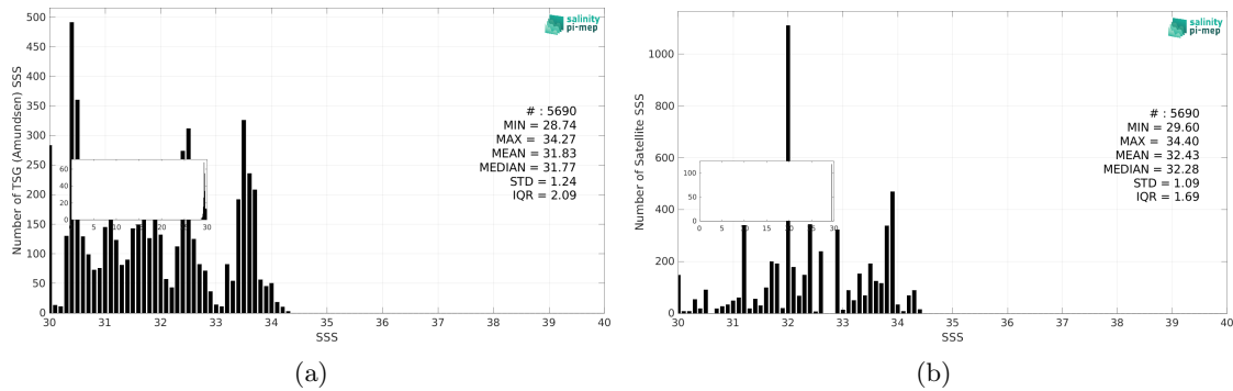
Figure 3: Histograms of SSS from TSG (Amundsen) (a) and Aquarius SSS L3 CAP v5 - 7-Day running (JPL) (b) considering all match-up pairs per bins of 0.1 over the Global Ocean Pi-MEP region and for the full satellite product period.
