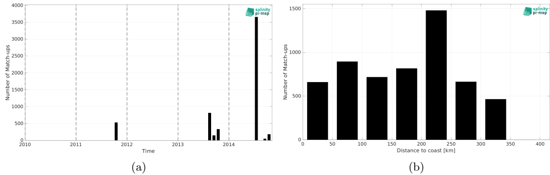
Figure 2: Number of match-ups between TSG (Amundsen) and Aquarius SSS L3 CAP v5 - 7-Day running (JPL) SSS as a function of time (a) and as function of the distance to coast (b) over the Global Ocean Pi-MEP region and for the full satellite product period.
