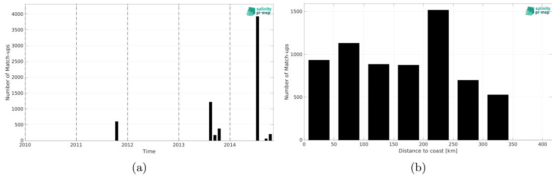
Figure 1: Number of match-ups between TSG (Amundsen) and Aquarius SSS L3 CAP v5 - 7-Day running (JPL) SSS as a function of time (a) and as function of the distance to coast (b) over the Global Ocean Pi-MEP region and for the full satellite product period.
