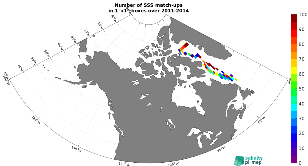
Figure 4: Number of SSS match-ups between TSG (Amundsen) SSS and the Aquarius SSS L3 CAP v5 - 7-Day running (JPL) SSS product for the Global Ocean Pi-MEP region over 1^\circ \times 1^\circ boxes and for the full satellite product period.
