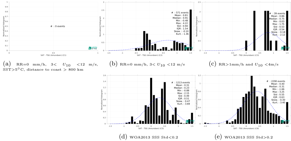
Figure 13: Normalized histogram of \Delta SSS (Aquarius SSS L3 CAP v5 - 7-Day running (JPL) - TSG (Amundsen)) for 5 different subdatasets corresponding to: RR=0 mm/h, 3 < U_{10} < 12 m/s, SST > 5°C, distance to coast > 800 km (a), RR=0 mm/h, 3 < U_{10} < 12 m/s (b), RR > 1mm/h and U_{10} < 4 m/s (c), WOA2013 SSS Std < 0.2 (d), WOA2013 SSS Std > 0.2 (e).
