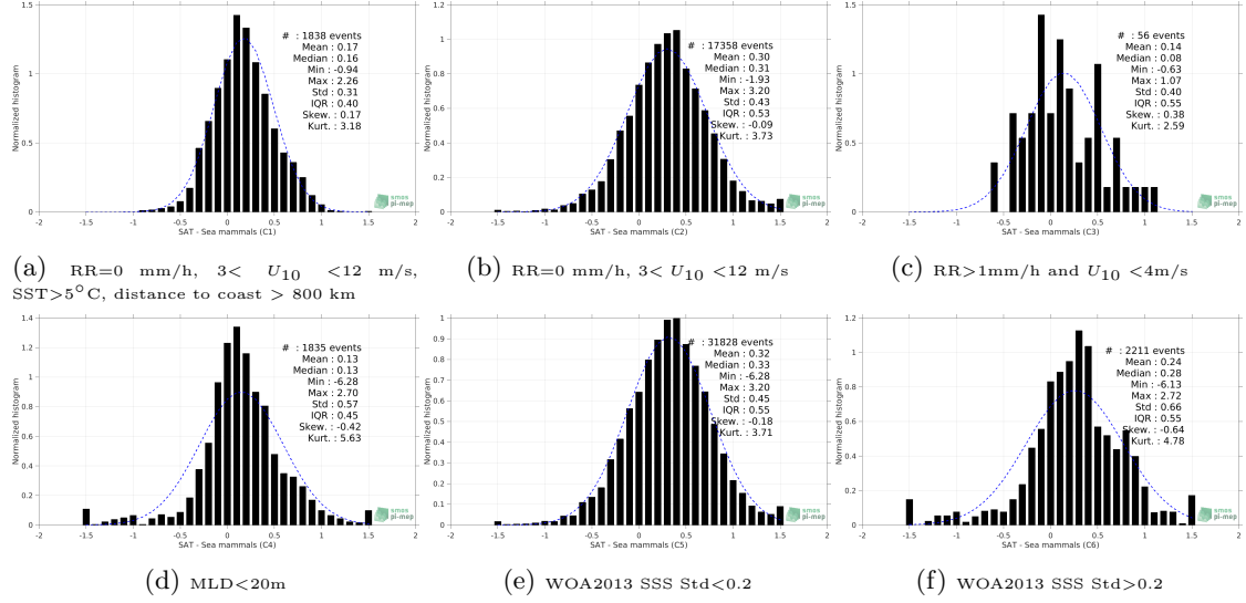
Figure 13: Normalized histogram of \Delta SSS (Aquarius SSS L3 CAP v5 - 7-Day running (JPL) - Sea mammals) for 6 different subdatasets corresponding to: RR=0 mm/h, 3 < U_{10} < 12 m/s, SST>5°C, distance to coast > 800 km (a), RR=0 mm/h, 3 < U_{10} < 12 m/s (b), RR>1mm/h and U_{10} < 4 m/s (c), MLD<20m (d), WOA2013 SSS Std<0.2 (e), WOA2013 SSS Std>0.2 (f).
