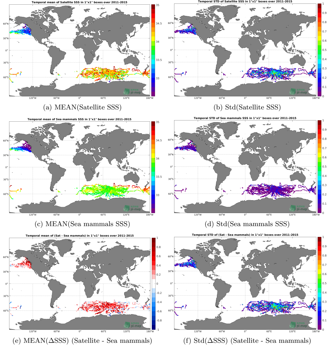
Figure 6: Temporal mean (left) and Std (right) of SSS from Aquarius SSS L3 CAP v5 - 7-Day running (JPL) (top), Sea mammals (middle), and of \Delta SSS (Satellite - Sea mammals). Only match-up pairs are used to generate these maps.
