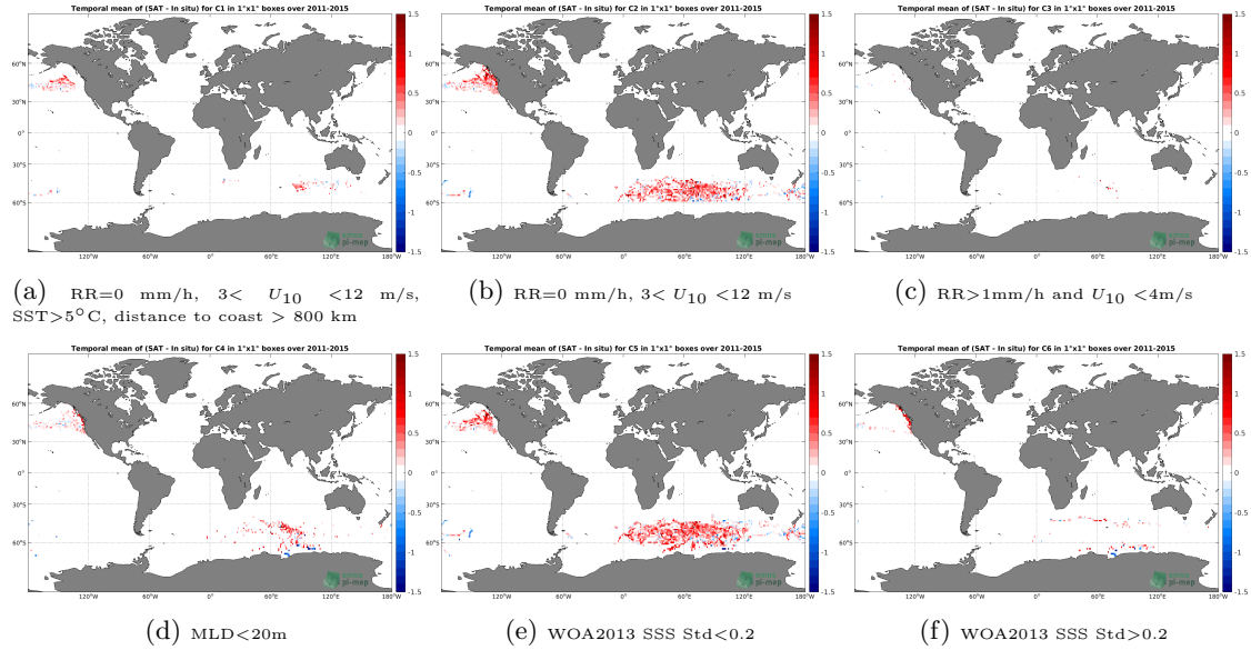
Figure 12: Temporal mean gridded over spatial boxes of size 1^\circ \times 1^\circ of \Delta SSS (Aquarius SSS L3 CAP v5 - 7-Day running (JPL) - Sea mammals) for 6 different subdatasets corresponding to: RR=0 mm/h, 3 < U_{10} < 12 m/s, SST > 5^\circ C , distance to coast > 800 km (a), RR=0 mm/h, 3 < U_{10} < 12 m/s (b), RR > 1 mm/h and U_{10} < 4 m/s (c), MLD < 20 m (d), WOA2013 SSS Std < 0.2 (e), WOA2013 SSS Std > 0.2 (f).
