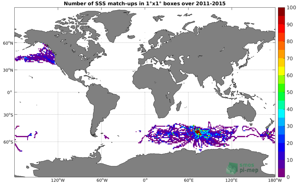
Figure 4: Number of SSS match-ups between Sea mammals SSS and the Aquarius SSS L3 CAP v5 - 7-Day running (JPL) SSS product for the Global Ocean Pi-MEP region over 1^\circ \times 1^\circ boxes and for the full satellite product period.
