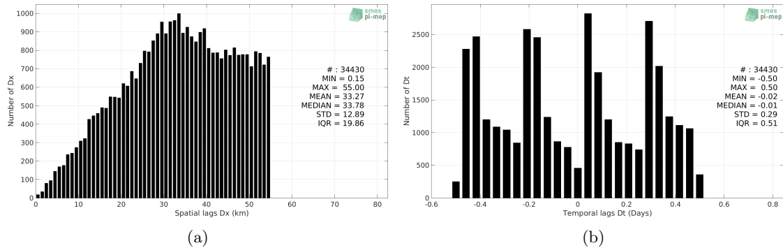
Figure 5: Histograms of the spatial (a) and temporal (b) lags between the time of the Sea mammals measurements and the date of the corresponding Aquarius SSS L3 CAP v5 - 7-Day running (JPL) SSS product.
