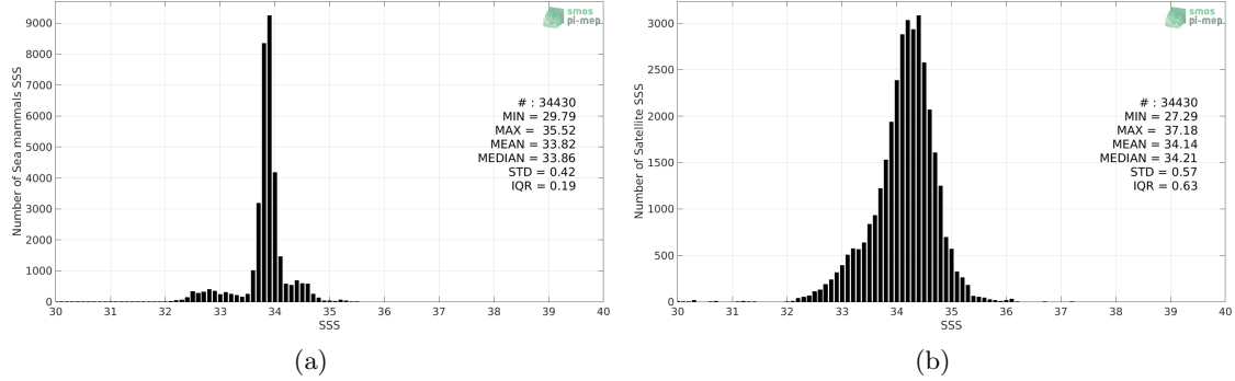
Figure 2: Histograms of SSS from Sea mammals (a) and Aquarius SSS L3 CAP v5 - 7-Day running (JPL) (b) considering all match-up pairs per bins of 0.1 over the Global Ocean Pi-MEP region and for the full satellite product period.
