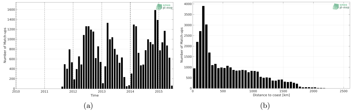
Figure 1: Number of match-ups between Sea mammals and Aquarius SSS L3 CAP v5 - 7-Day running (JPL) SSS as a function of time (a) and as function of the distance to coast (b) over the Global Ocean Pi-MEP region and for the full satellite product period.
