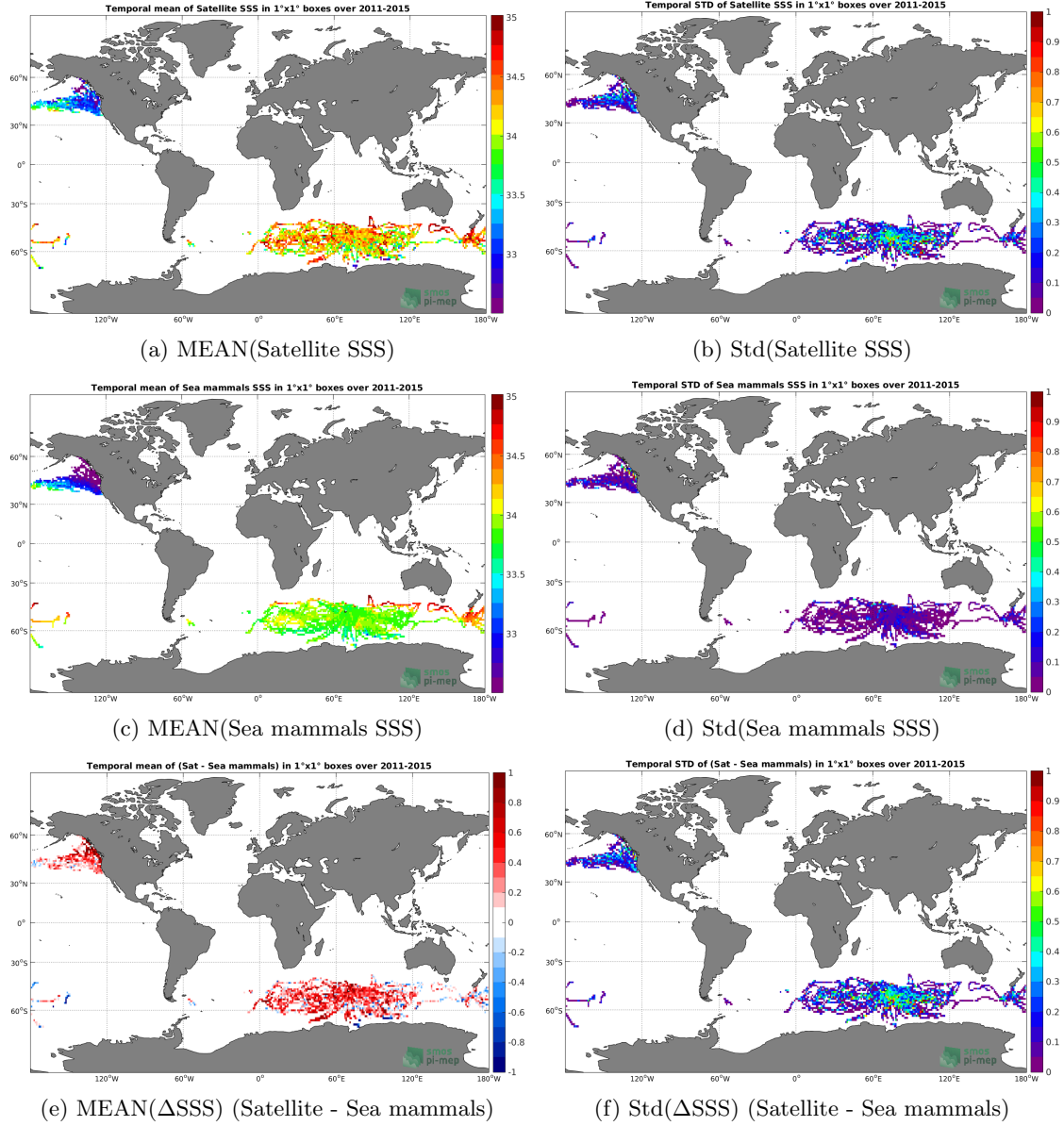
Figure 6: Temporal mean (left) and Std (right) of SSS from Aquarius-L3-JPL-V5-7DAY-RUNNING (top), Sea mammals (middle), and of \Delta SSS (Satellite - Sea mammals). Only match-up pairs are used to generate these maps.
