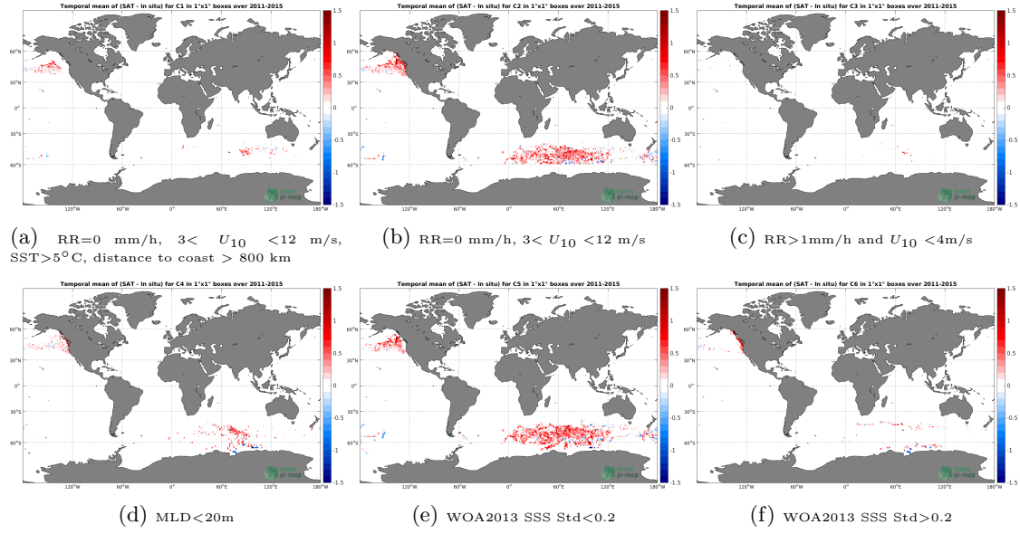
Figure 12: Temporal mean gridded over spatial boxes of size 1^\circ \times 1^\circ of \Delta SSS (Aquarius-L3-JPL-V5-7DAY-RUNNING - Sea mammals) for 6 different subdatasets corresponding to: RR=0 mm/h, 3 < U_{10} < 12 m/s, SST > 5^\circ C , distance to coast > 800 km (a), RR=0 mm/h, 3 < U_{10} < 12 m/s (b), RR > 1 mm/h and U_{10} < 4 m/s (c), MLD < 20 m (d), WOA2013 SSS Std < 0.2 (e), WOA2013 SSS Std > 0.2 (f).
