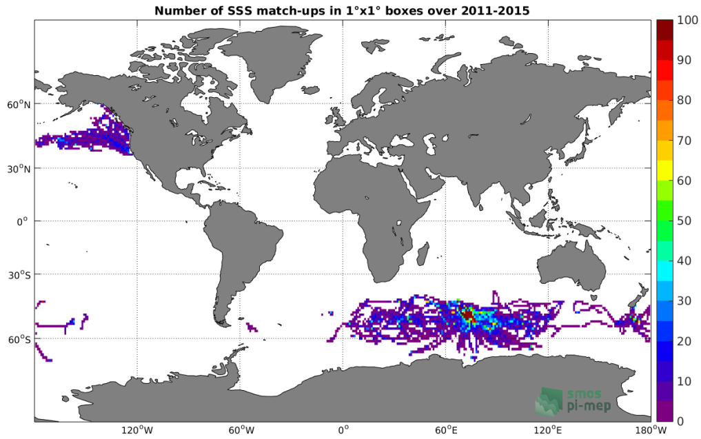
Figure 4: Number of SSS match-ups between Sea mammals SSS and the Aquarius-L3-JPL-V5-7DAY-RUNNING SSS product for the Global Ocean Pi-MEP region over 1^\circ \times 1^\circ boxes and for the full satellite product period.
