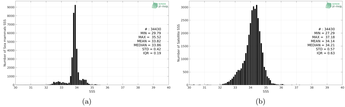
Figure 2: Histograms of SSS from Sea mammals (a) and Aquarius-L3-JPL-V5-7DAY-RUNNING (b) considering all match-up pairs per bins of 0.1 over the Global Ocean Pi-MEP region and for the full satellite product period.
