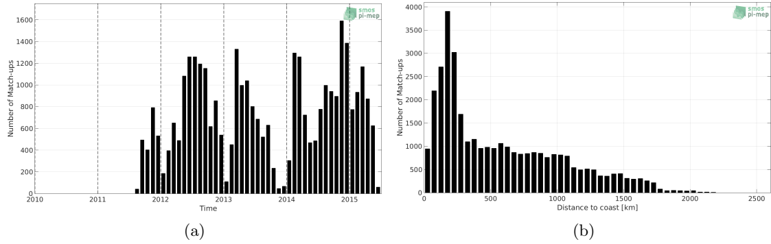
Figure 1: Number of match-ups between Sea mammals and Aquarius-L3-JPL-V5-7DAY-RUNNING SSS as a function of time (a) and as function of the distance to coast (b) over the Global Ocean Pi-MEP region and for the full satellite product period.
