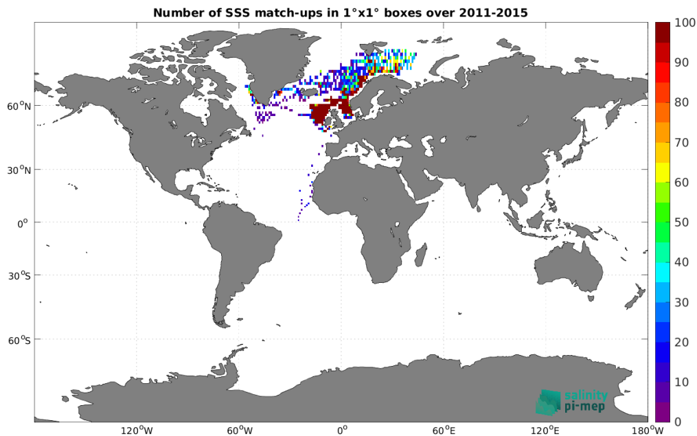
Figure 4: Number of SSS match-ups between ICES SSS and the Aquarius SSS L3 CAP v5 - 7-Day running (JPL) SSS product for the Global Ocean Pi-MEP region over 1^\circ \times 1^\circ boxes and for the full satellite product period.
