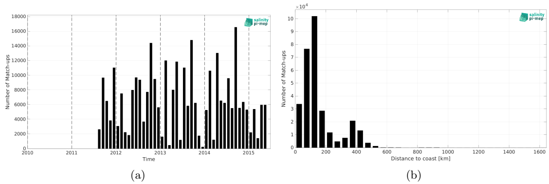
Figure 1: Number of match-ups between ICES and Aquarius SSS L3 CAP v5 - 7-Day running (JPL) SSS as a function of time (a) and as function of the distance to coast (b) over the Global Ocean Pi-MEP region and for the full satellite product period.
