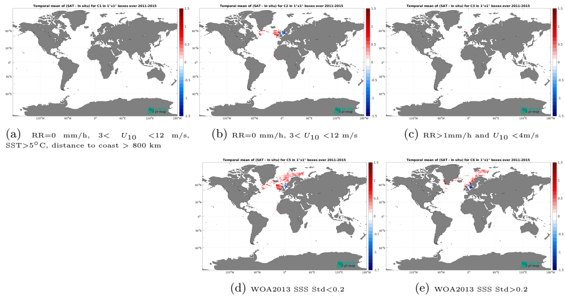
Figure 12: Temporal mean gridded over spatial boxes of size 1^\circ \times 1^\circ of \Delta SSS (Aquarius SSS L3 CAP v5 - 7-Day running (JPL) - ICES) for 5 different subdatasets corresponding to:RR=0 mm/h, 3 < U_{10} < 12 m/s, SST >5^\circ C, distance to coast > 800 km (a), RR=0 mm/h, 3 < U_{10} < 12 m/s (b), RR >1 mm/h and U_{10} < 4 m/s (c), WOA2013 SSS Std <0.2 (d), WOA2013 SSS Std >0.2 (e).
