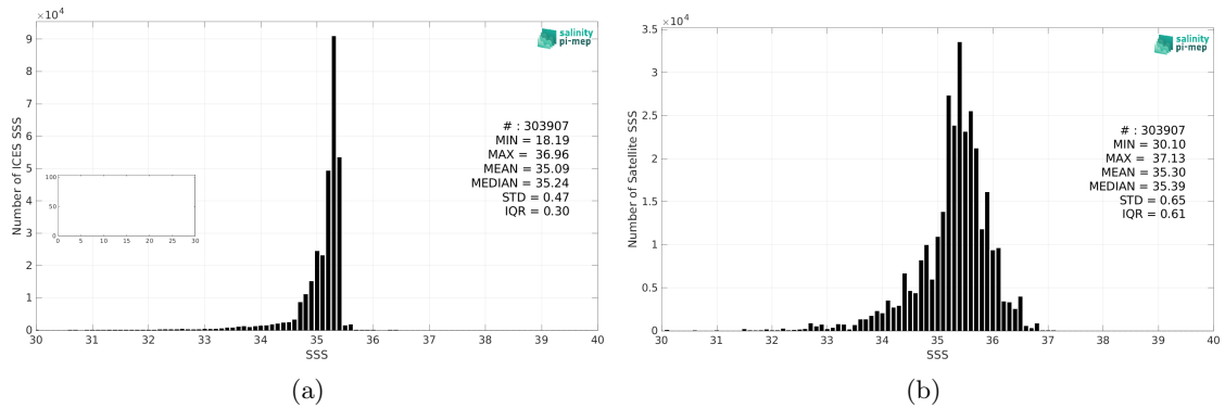
Figure 2: Histograms of SSS from ICES (a) and Aquarius SSS L3 CAP v5 - 7-Day running (JPL) (b) considering all match-up pairs per bins of 0.1 over the Global Ocean Pi-MEP region and for the full satellite product period.
