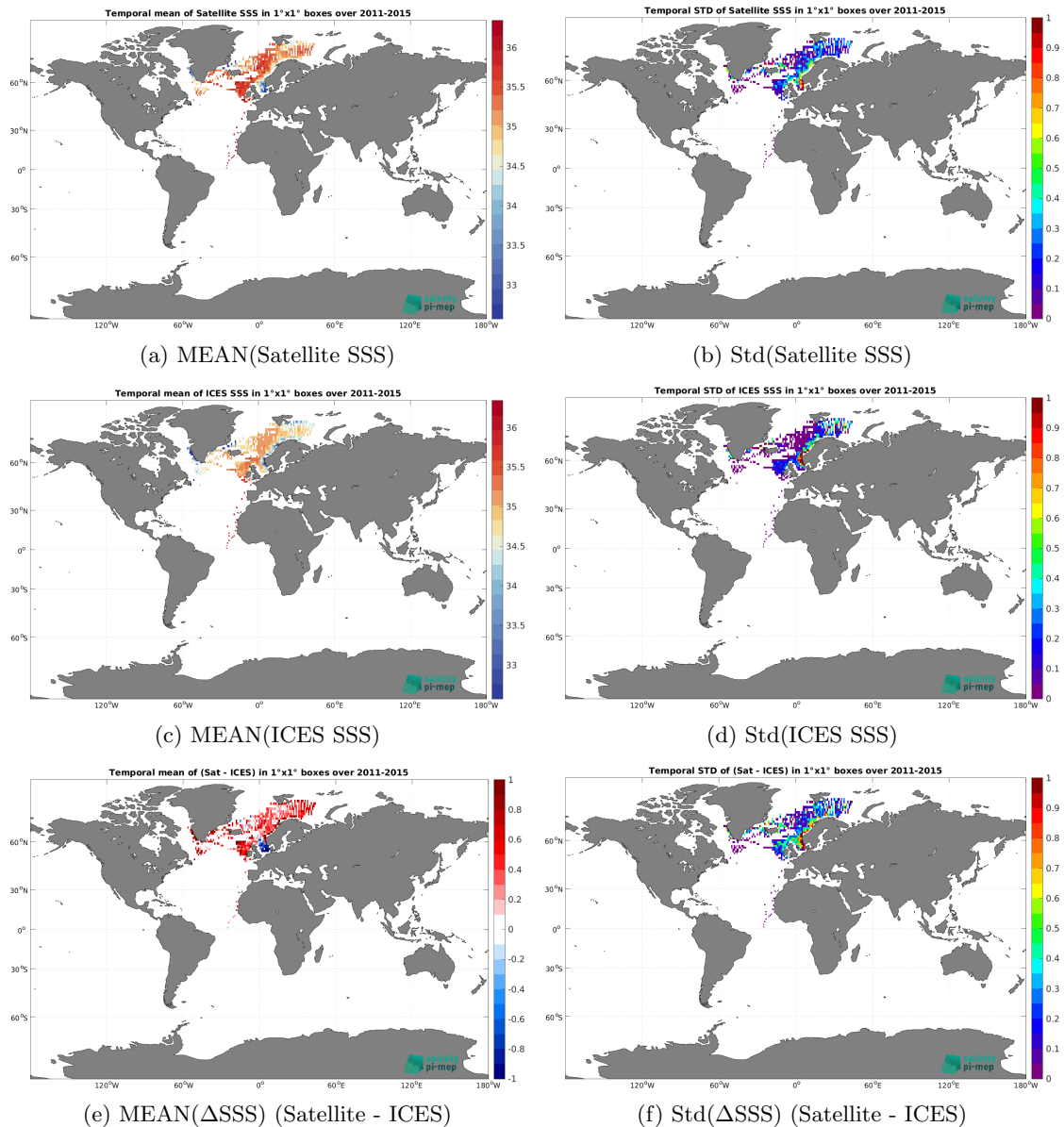
Figure 6: Temporal mean (left) and Std (right) of SSS from Aquarius SSS L3 CAP v5 - 7-Day running (JPL) (top), ICES (middle), and of \Delta SSS (Satellite - ICES). Only match-up pairs are used to generate these maps.
