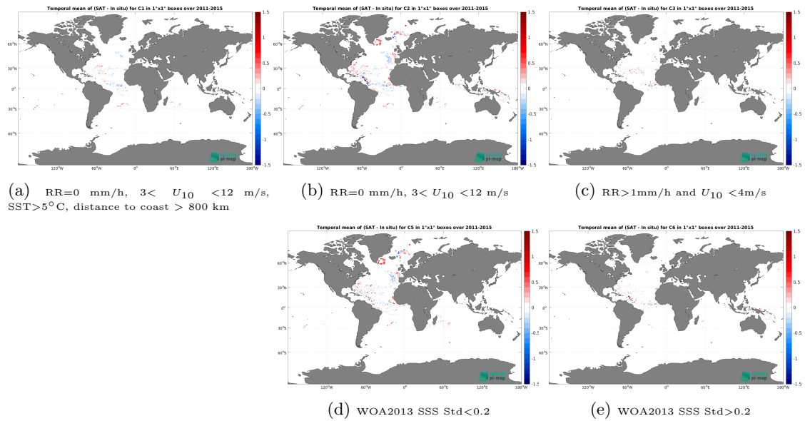
Figure 13: Temporal mean gridded over spatial boxes of size 1^\circ \times 1^\circ of \Delta SSS (Aquarius SSS L3 CAP v5 - 7-Day running (JPL) - Surface drifters) for 5 different subdatasets corresponding to:RR=0 mm/h, 3 < U_{10} < 12 m/s, SST >5^\circ C, distance to coast > 800 km (a), RR=0 mm/h, 3 < U_{10} < 12 m/s (b), RR >1 mm/h and U_{10} < 4 m/s (c), WOA2013 SSS Std <0.2 (d), WOA2013 SSS Std >0.2 (e).
