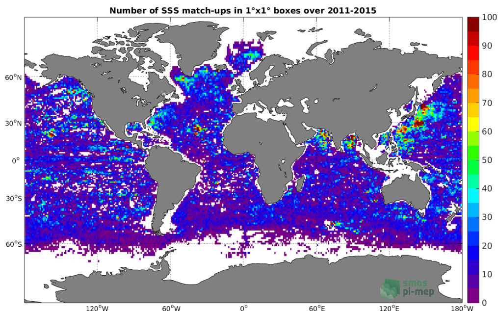
Figure 4: Number of SSS match-ups between Argo SSS and the Aquarius-L3-JPL-V5-7DAY-RUNNING SSS product for the Global Ocean Pi-MEP region over 1°x1° boxes and for the full satellite product period.
