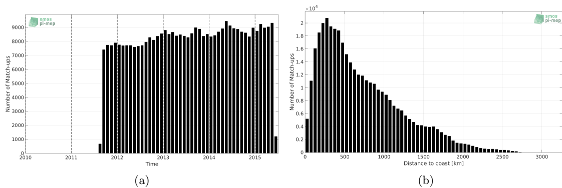
Figure 1: Number of match-ups between Argo and Aquarius-L3-JPL-V5-7DAY-RUNNING SSS as a function of time (a) and as function of the distance to coast (b) over the Global Ocean Pi-MEP region and for the full satellite product period.
