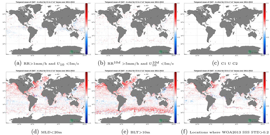
Figure 12: Temporal mean gridded over spatial boxes of size 1°x1° of \Delta SSS (Aquarius-L3-JPL-V5-7DAY-RUNNING - Argo) for 6 different subdatasets corresponding to: RR > 1\text{mm/h} and U_{10} < 5\text{m/s} (a), RR^{10d} > 5\text{mm/h} and U_{10}^{10d} < 5\text{m/s} (b), C1 U C2 (c), MLD < 20\text{m} (d), BLT > 10\text{m} (e), Locations where WOA2013 SSS STD > 0.2 (f).
