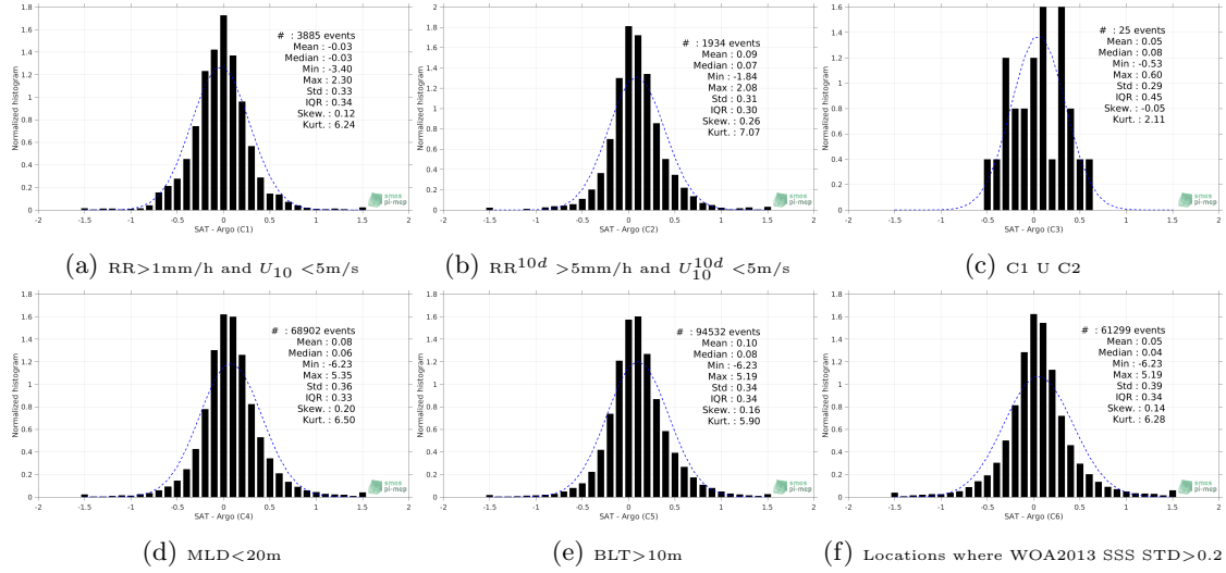
Figure 13: Normalized histogram of \Delta SSS (Aquarius-L3-JPL-V5-7DAY-RUNNING - Argo) for 6 different subdatasets corresponding to: RR > 1mm/h and U_{10} < 5 m/s (a), RR^{10d} > 5 mm/h and U_{10}^{10d} < 5 m/s (b), C1 U C2 (c), MLD < 20m (d), BLT > 10m (e), Locations where WOA2013 SSS STD > 0.2 (f).
