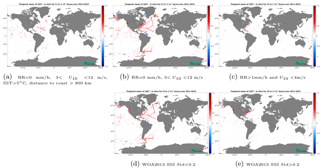
Figure 14: Temporal mean gridded over spatial boxes of size 1^\circ \times 1^\circ of \Delta\text{SSS} (Aquarius SSS L3 CAP v5 - Monthly (JPL) - TSG (SAMOS)) for 5 different subdatasets corresponding to:RR=0 mm/h, 3 < U_{10} < 12 m/s, SST > 5^\circ\text{C} , distance to coast > 800 km (a), RR=0 mm/h, 3 < U_{10} < 12 m/s (b), RR > 1 mm/h and U_{10} < 4 m/s (c), WOA2013 SSS Std < 0.2 (d), WOA2013 SSS Std > 0.2 (e).
