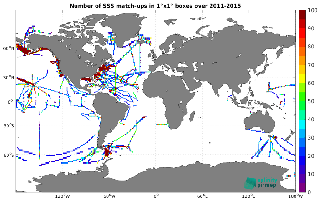
Figure 5: Number of SSS match-ups between TSG (SAMOS) SSS and the Aquarius SSS L3 CAP v5 - Monthly (JPL) SSS product for the Global Ocean Pi-MEP region over 1^\circ \times 1^\circ boxes and for the full satellite product period.
