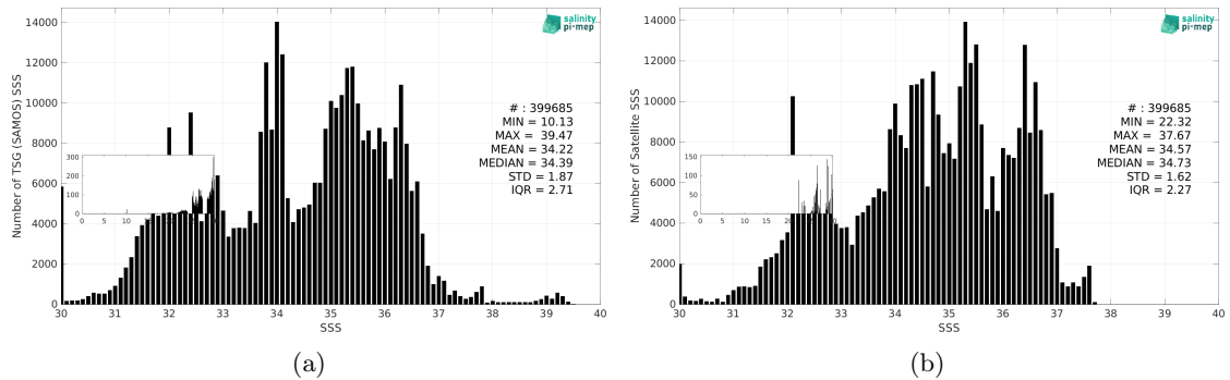
Figure 3: Histograms of SSS from TSG (SAMOS) (a) and Aquarius SSS L3 CAP v5 - Monthly (JPL) (b) considering all match-up pairs per bins of 0.1 over the Global Ocean Pi-MEP region and for the full satellite product period.
