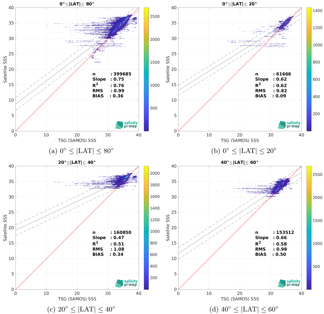
Figure 10: Contour maps of the concentration of Aquarius SSS L3 CAP v5 - Monthly (JPL) SSS (y-axis) versus TSG (SAMOS) SSS (x-axis) at match-up pairs for different latitude bands. For each plot, the red line shows x=y . The black thin and dashed lines indicate a linear fit through the data cloud and the \pm 95\% confidence levels, respectively. The number match-up pairs n , the slope and R^2 coefficient of the linear fit, the root mean square (RMS) and the mean bias between satellite and in situ data are indicated for each latitude band in each plots.
