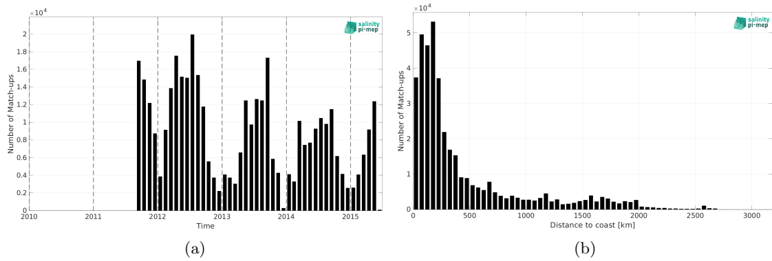
Figure 2: Number of match-ups between TSG (SAMOS) and Aquarius SSS L3 CAP v5 - Monthly (JPL) SSS as a function of time (a) and as function of the distance to coast (b) over the Global Ocean Pi-MEP region and for the full satellite product period.
