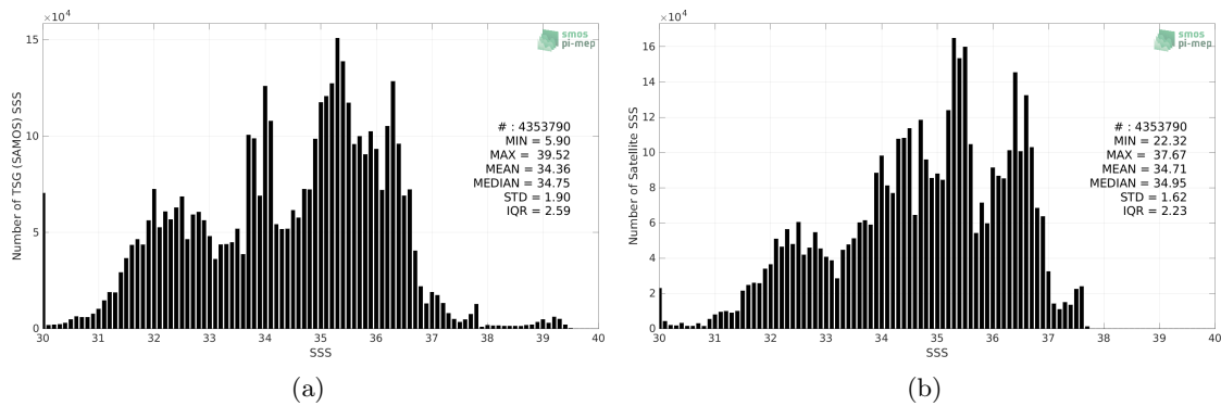
Figure 2: Histograms of SSS from TSG (SAMOS) (a) and Aquarius SSS L3 CAP v5 - Monthly (JPL) (b) considering all match-up pairs per bins of 0.1 over the Global Ocean Pi-MEP region and for the full satellite product period.
