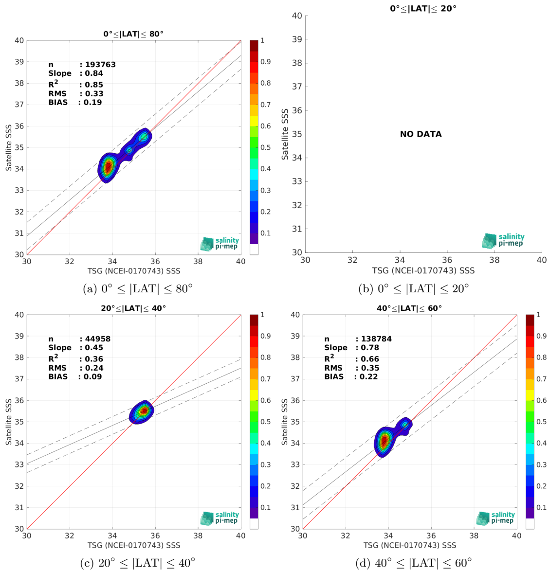
Figure 10: Contour maps of the concentration of Aquarius SSS L3 CAP v5 - Monthly (JPL) SSS (y-axis) versus TSG (NCEI-0170743) SSS (x-axis) at match-up pairs for different latitude bands. For each plot, the red line shows x=y . The black thin and dashed lines indicate a linear fit through the data cloud and the \pm 95\% confidence levels, respectively. The number match-up pairs n , the slope and R^2 coefficient of the linear fit, the root mean square (RMS) and the mean bias between satellite and in situ data are indicated for each latitude band in each plots.
