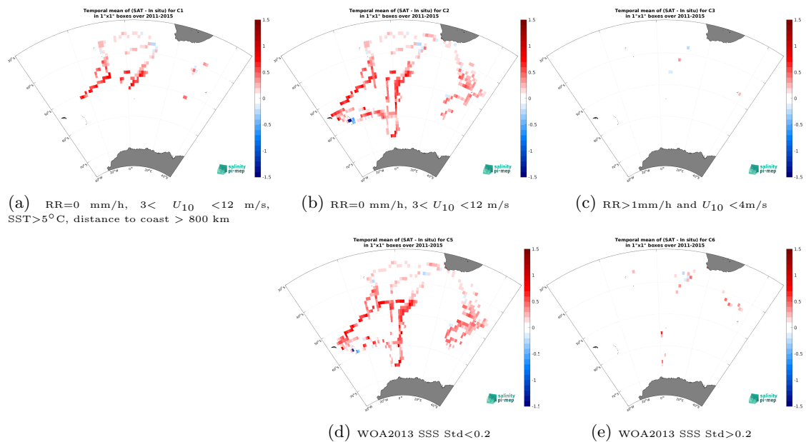
Figure 14: Temporal mean gridded over spatial boxes of size 1^\circ \times 1^\circ of \Delta SSS (Aquarius SSS L3 CAP v5 - Monthly (JPL) - TSG (NCEI-0170743)) for 5 different subdatasets corresponding to: RR=0 mm/h, 3 < U_{10} < 12 m/s, SST > 5^\circ\text{C} , distance to coast > 800 km (a), RR=0 mm/h, 3 < U_{10} < 12 m/s (b), RR > 1 mm/h and U_{10} < 4 m/s (c), WOA2013 SSS Std < 0.2 (d), WOA2013 SSS Std > 0.2 (e).
