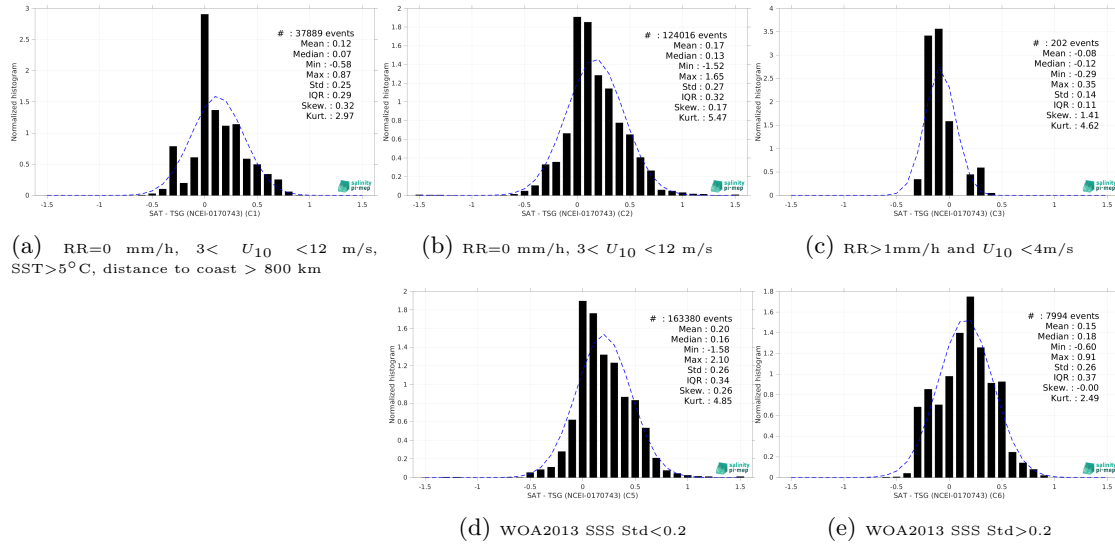
Figure 15: Normalized histogram of \Delta SSS (Aquarius SSS L3 CAP v5 - Monthly (JPL) - TSG (NCEI-0170743)) for 5 different subdatasets corresponding to: RR=0 mm/h, 3 < U_{10} < 12 m/s, SST > 5°C, distance to coast > 800 km (a), RR=0 mm/h, 3 < U_{10} < 12 m/s (b), RR > 1mm/h and U_{10} < 4 m/s (c), WOA2013 SSS Std < 0.2 (d), WOA2013 SSS Std > 0.2 (e).
