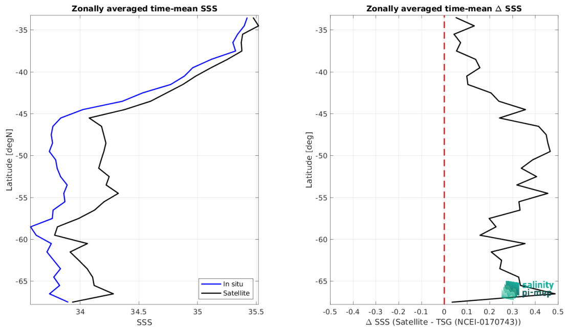
Figure 9: Left panel: Zonal mean SSS from Aquarius SSS L3 CAP v5 - Monthly (JPL) satellite product (black) and from TSG (NCEI-0170743) (blue). Right panel: Zonal mean of \Delta SSS (Satellite - TSG (NCEI-0170743)) for all the collected Pi-MEP match-up pairs estimated over the full satellite product period.
