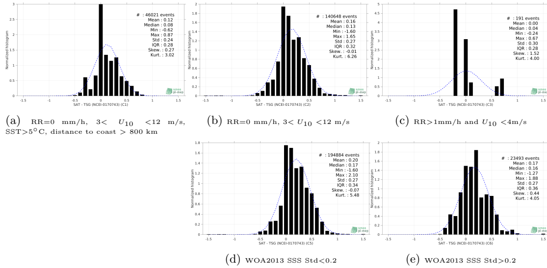
Figure 13: Normalized histogram of \Delta SSS (Aquarius SSS L3 CAP v5 - Monthly (JPL) - TSG (NCEI-0170743)) for 5 different subdatasets corresponding to: RR=0 mm/h, 3 < U_{10} < 12 m/s, SST > 5°C, distance to coast > 800 km (a), RR=0 mm/h, 3 < U_{10} < 12 m/s (b), RR > 1mm/h and U_{10} < 4 m/s (c), WOA2013 SSS Std < 0.2 (d), WOA2013 SSS Std > 0.2 (e).
