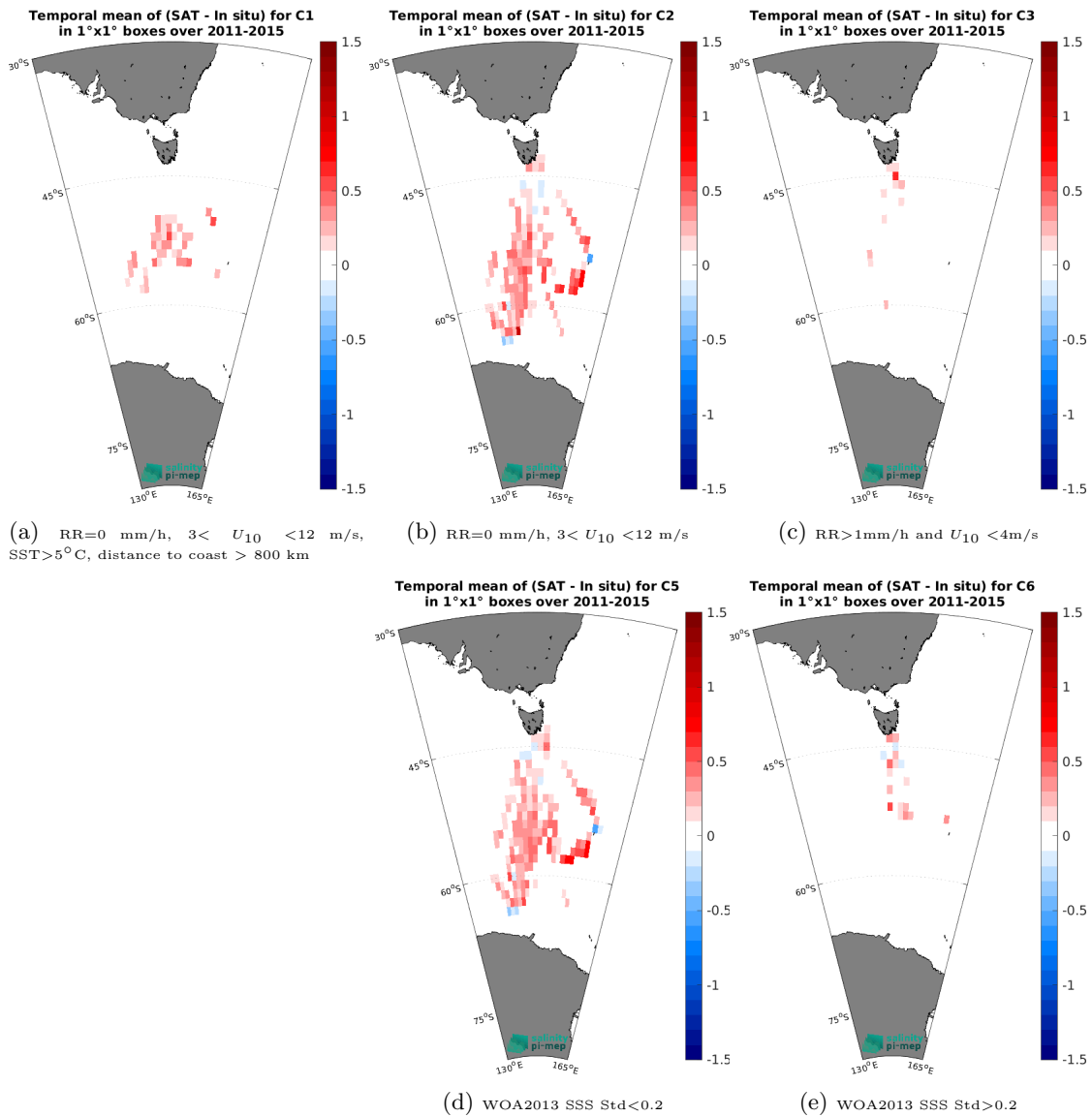
Figure 14: Temporal mean gridded over spatial boxes of size 1^\circ \times 1^\circ of \Delta SSS (Aquarius SSS L3 CAP v5 - Monthly (JPL) - TSG (LEGOS-Survostral)) for 5 different subdatasets corresponding to:RR=0 mm/h, 3 < U_{10} < 12 m/s, SST>5°C, distance to coast > 800 km (a), RR=0 mm/h, 3 < U_{10} < 12 m/s (b), RR>1mm/h and U_{10} < 4 m/s (c), WOA2013 SSS Std<0.2 (d), WOA2013 SSS Std>0.2 (e).
