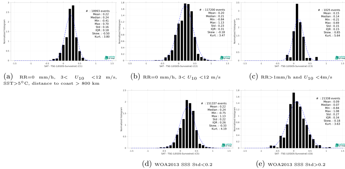
Figure 15: Normalized histogram of \Delta SSS (Aquarius SSS L3 CAP v5 - Monthly (JPL) - TSG (LEGOS-Survostral)) for 5 different subdatasets corresponding to: RR=0 mm/h, 3 < U_{10} < 12 m/s, SST>5°C, distance to coast > 800 km (a), RR=0 mm/h, 3 < U_{10} < 12 m/s (b), RR>1mm/h and U_{10} < 4 m/s (c), WOA2013 SSS Std<0.2 (d), WOA2013 SSS Std>0.2 (e).
