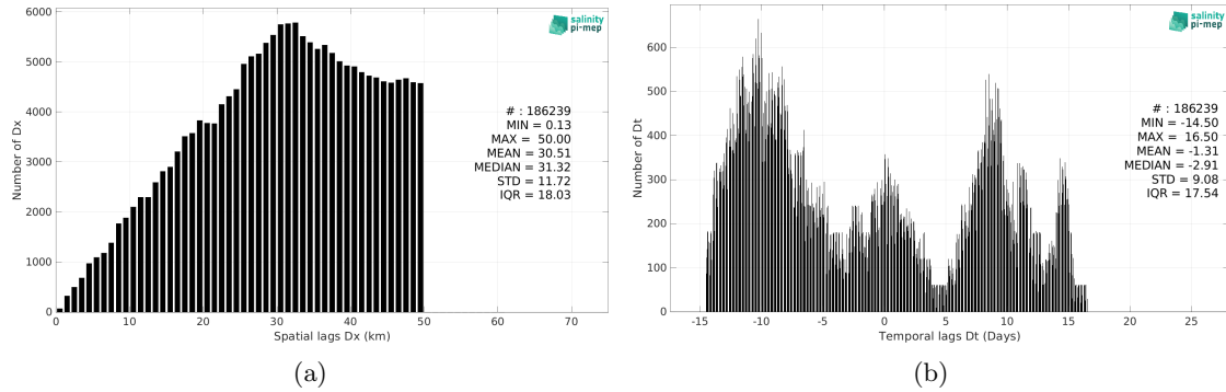
Figure 6: Histograms of the spatial (a) and temporal (b) lags between the location/time of the TSG (LEGOS-Survostral) measurement and the date of the corresponding Aquarius SSS L3 CAP v5 - Monthly (JPL) SSS pixel.
