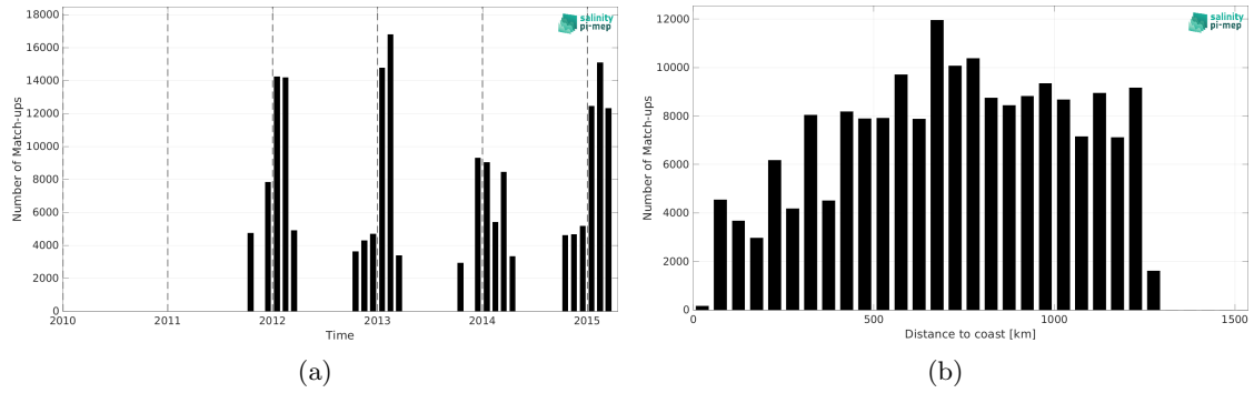
Figure 2: Number of match-ups between TSG (LEGOS-Survostral) and Aquarius SSS L3 CAP v5 - Monthly (JPL) SSS as a function of time (a) and as function of the distance to coast (b) over the Global Ocean Pi-MEP region and for the full satellite product period.
