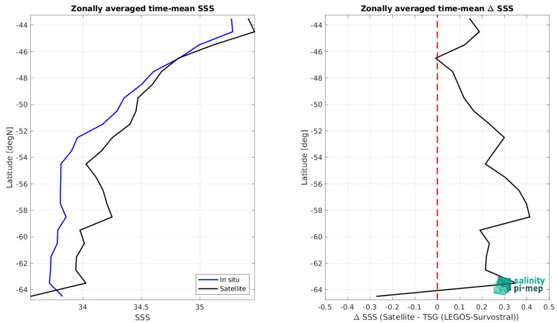
Figure 9: Left panel: Zonal mean SSS from Aquarius SSS L3 CAP v5 - Monthly (JPL) satellite product (black) and from TSG (LEGOS-Survostral) (blue). Right panel: Zonal mean of \Delta SSS (Satellite - TSG (LEGOS-Survostral)) for all the collected Pi-MEP match-up pairs estimated over the full satellite product period.
