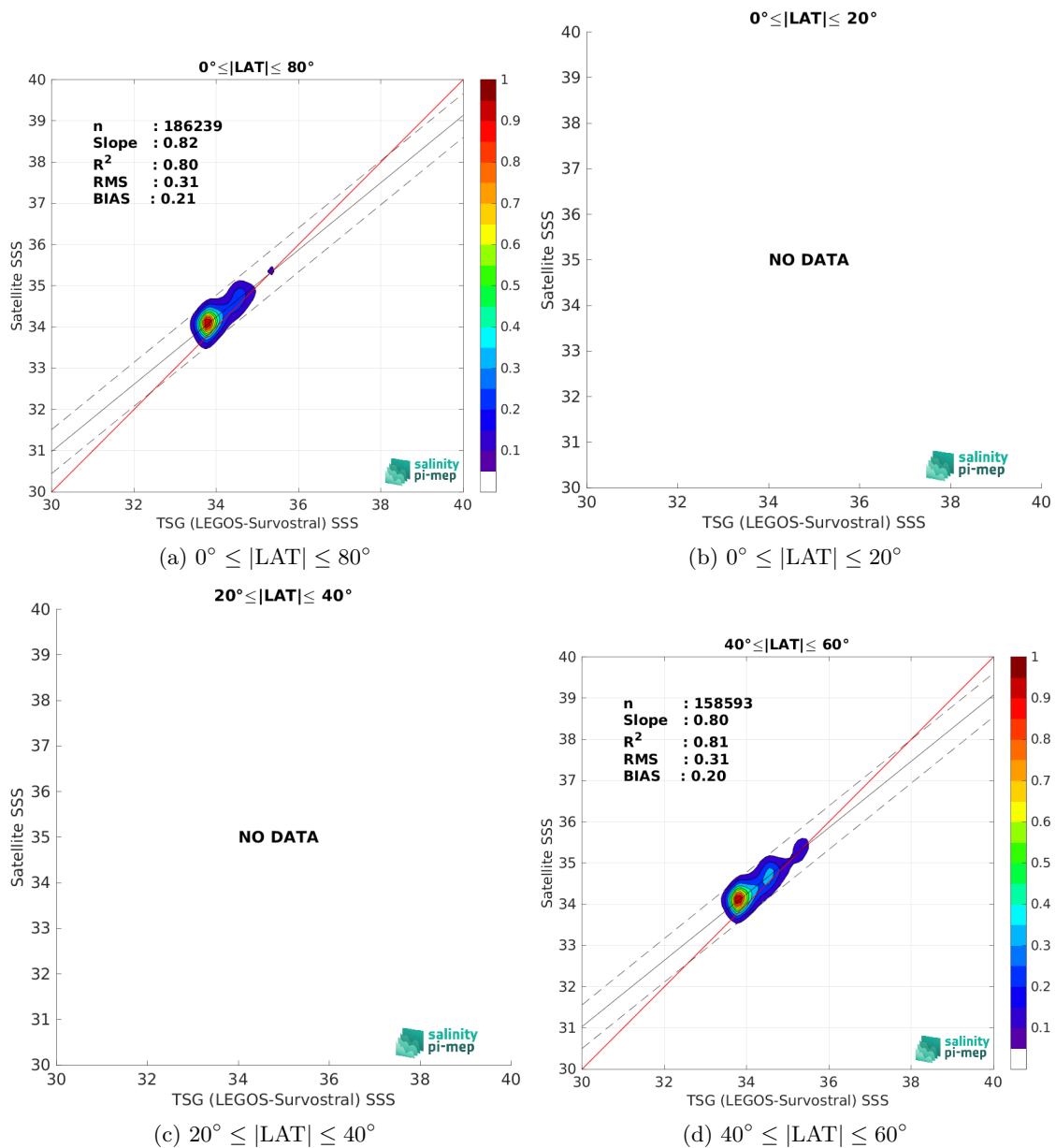
Figure 10: Contour maps of the concentration of Aquarius SSS L3 CAP v5 - Monthly (JPL) SSS (y-axis) versus TSG (LEGOS-Survostral) SSS (x-axis) at match-up pairs for different latitude bands. For each plot, the red line shows x=y . The black thin and dashed lines indicate a linear fit through the data cloud and the \pm 95\% confidence levels, respectively. The number match-up pairs n , the slope and R^2 coefficient of the linear fit, the root mean square (RMS) and the mean bias between satellite and in situ data are indicated for each latitude band in each plots.
