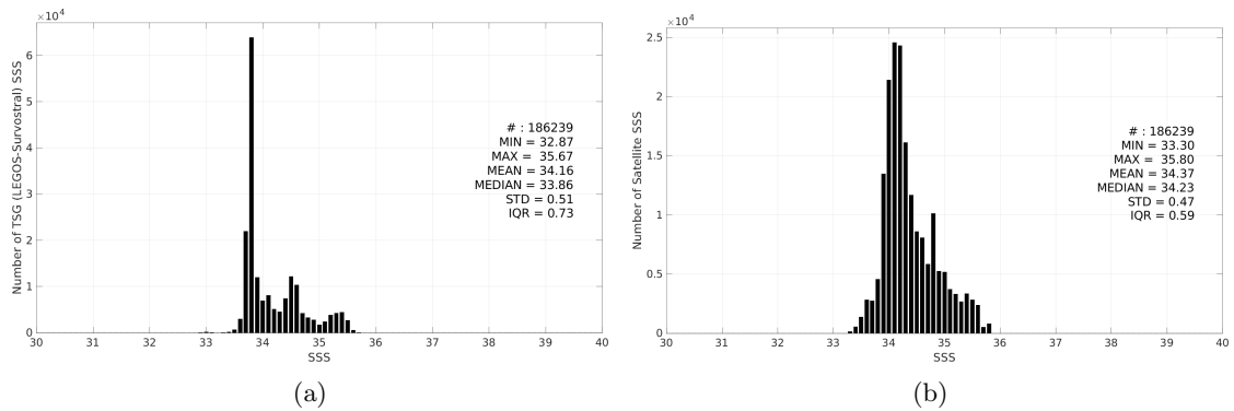
Figure 3: Histograms of SSS from TSG (LEGOS-Survostral) (a) and Aquarius SSS L3 CAP v5 - Monthly (JPL) (b) considering all match-up pairs per bins of 0.1 over the Global Ocean Pi-MEP region and for the full satellite product period.
