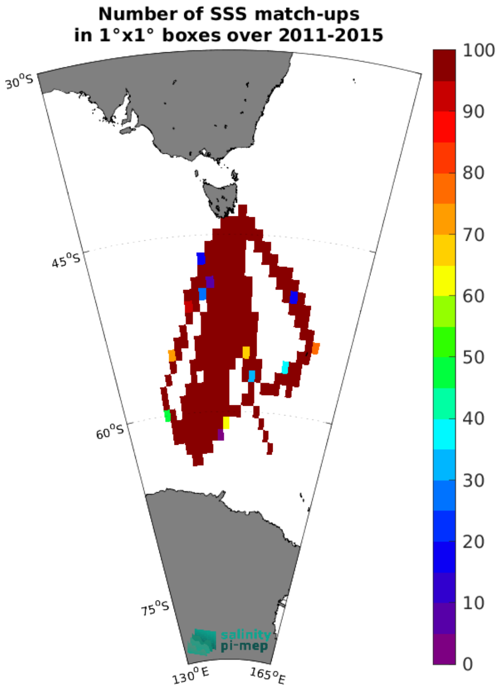
Figure 5: Number of SSS match-ups between TSG (LEGOS-Survostral) SSS and the Aquarius SSS L3 CAP v5 - Monthly (JPL) SSS product for the Global Ocean Pi-MEP region over 1°x1° boxes and for the full satellite product period.
