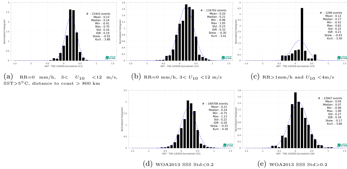
Figure 13: Normalized histogram of \Delta SSS (Aquarius SSS L3 CAP v5 - Monthly (JPL) - TSG (LEGOS-Survostral)) for 5 different subdatasets corresponding to: RR=0 mm/h, 3 < U_{10} < 12 m/s, SST > 5°C, distance to coast > 800 km (a), RR=0 mm/h, 3 < U_{10} < 12 m/s (b), RR > 1mm/h and U_{10} < 4 m/s (c), WOA2013 SSS Std < 0.2 (d), WOA2013 SSS Std > 0.2 (e).
