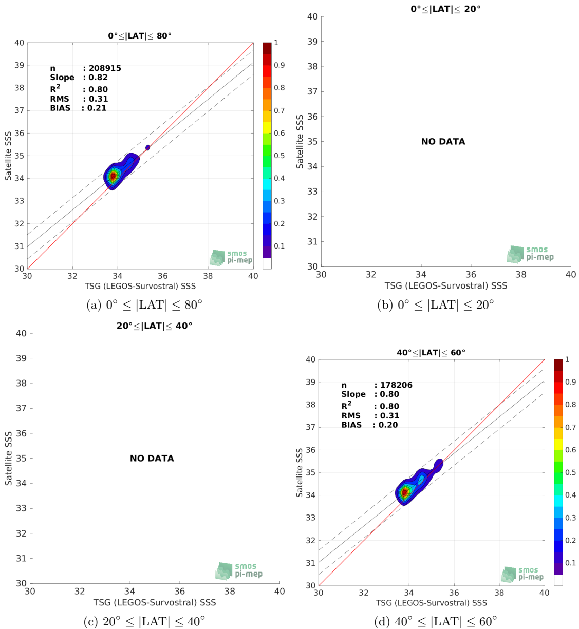
Figure 9: Contour maps of the concentration of Aquarius SSS L3 CAP v5 - Monthly (JPL) SSS (y-axis) versus TSG (LEGOS-Survostral) SSS (x-axis) at match-up pairs for different latitude bands. For each plot, the red line shows x=y . The black thin and dashed lines indicate a linear fit through the data cloud and the \pm 95\% confidence levels, respectively. The number match-up pairs n , the slope and R^2 coefficient of the linear fit, the root mean square (RMS) and the mean bias between satellite and in situ data are indicated for each latitude band in each plots.
