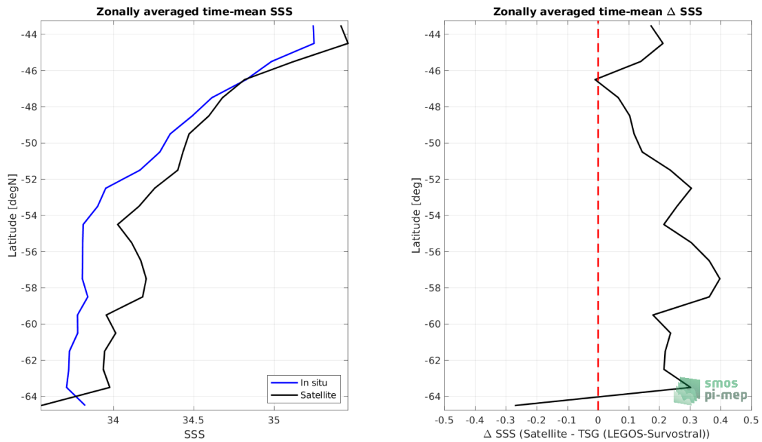
Figure 8: Left panel: Zonal mean SSS from Aquarius SSS L3 CAP v5 - Monthly (JPL) satellite product (black) and from TSG (LEGOS-Survostral) (blue). Right panel: Zonal mean of \Delta SSS (Satellite - TSG (LEGOS-Survostral)) for all the collected Pi-MEP match-up pairs estimated over the full satellite product period.
