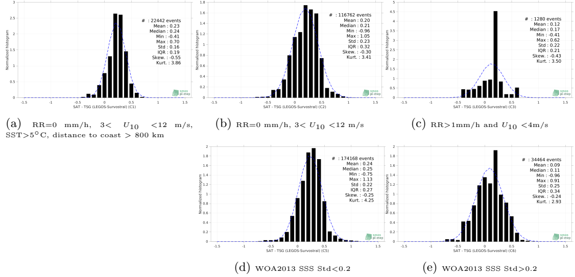
Figure 13: Normalized histogram of \Delta SSS (Aquarius SSS L3 CAP v5 - Monthly (JPL) - TSG (LEGOS-Survostral)) for 5 different subdatasets corresponding to: RR=0 mm/h, 3 < U_{10} < 12 m/s, SST > 5°C, distance to coast > 800 km (a), RR=0 mm/h, 3 < U_{10} < 12 m/s (b), RR > 1mm/h and U_{10} < 4 m/s (c), WOA2013 SSS Std < 0.2 (d), WOA2013 SSS Std > 0.2 (e).
