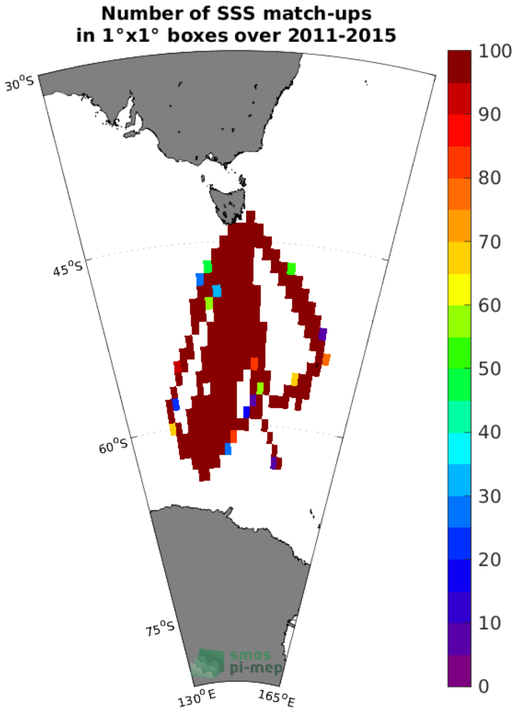
Figure 4: Number of SSS match-ups between TSG (LEGOS-Survostral) SSS and the Aquarius SSS L3 CAP v5 - Monthly (JPL) SSS product for the Global Ocean Pi-MEP region over 1°x1° boxes and for the full satellite product period.
