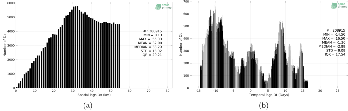
Figure 5: Histograms of the spatial (a) and temporal (b) lags between the location/time of the TSG (LEGOS-Survostral) measurement and the date of the corresponding Aquarius SSS L3 CAP v5 - Monthly (JPL) SSS pixel.
