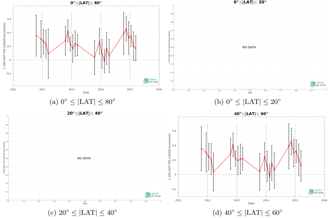
Figure 10: Monthly median (red curves) of \Delta SSS (Satellite - in situ TSG (LEGOS-Survostral)) and \pm 1 Std (black vertical thick bars) as function of time for all the collected Pi-MEP match-up pairs estimated over the Global Ocean Pi-MEP region and for the full satellite product period are shown for different latitude bands: (a) 80^\circ\text{S}-80^\circ\text{N} , (b) 20^\circ\text{S}-20^\circ\text{N} , (c) 40^\circ\text{S}-20^\circ\text{S} and 20^\circ\text{N}-40^\circ\text{N} and (d) 60^\circ\text{S}-40^\circ\text{S} and 40^\circ\text{N}-60^\circ\text{N} .
