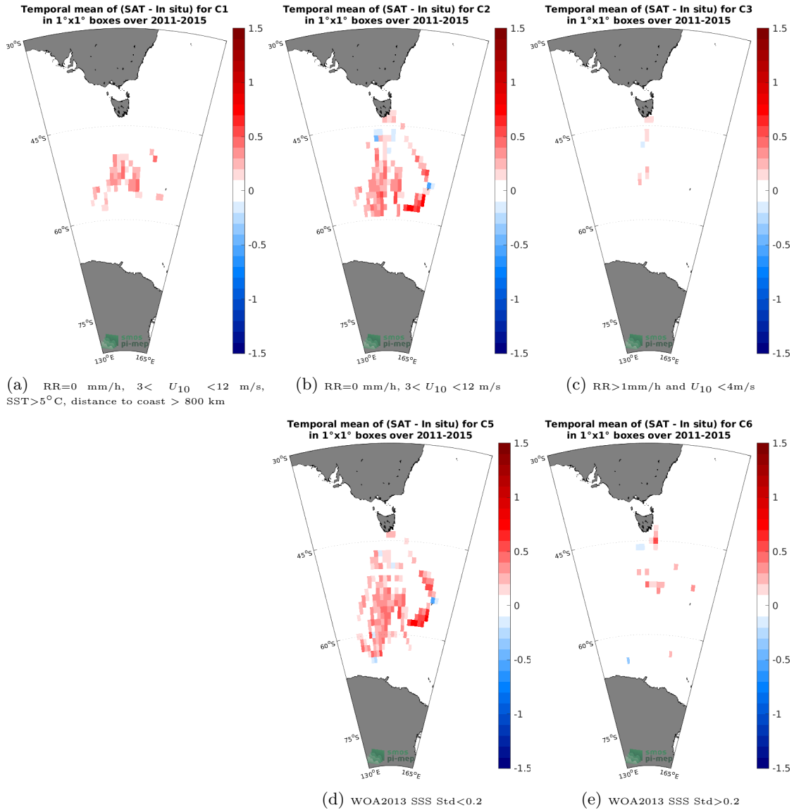
Figure 12: Temporal mean gridded over spatial boxes of size 1^\circ \times 1^\circ of \Delta SSS (Aquarius SSS L3 CAP v5 - Monthly (JPL) - TSG (LEGOS-Survostral)) for 5 different subdatasets corresponding to: RR=0 mm/h, 3 < U_{10} < 12 m/s, SST>5°C, distance to coast > 800 km (a), RR=0 mm/h, 3 < U_{10} < 12 m/s (b), RR>1mm/h and U_{10} < 4 m/s (c), WOA2013 SSS Std<0.2 (d), WOA2013 SSS Std>0.2 (e).
