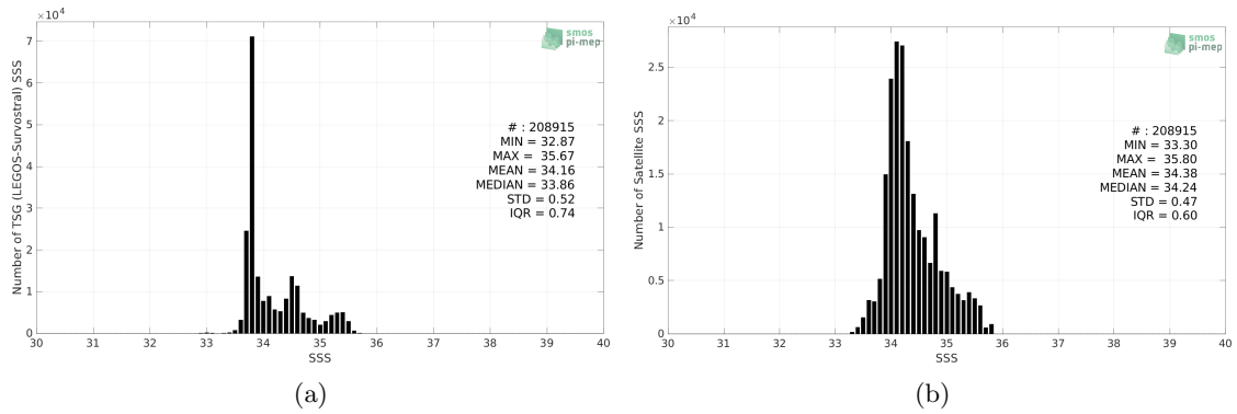
Figure 2: Histograms of SSS from TSG (LEGOS-Survostral) (a) and Aquarius SSS L3 CAP v5 - Monthly (JPL) (b) considering all match-up pairs per bins of 0.1 over the Global Ocean Pi-MEP region and for the full satellite product period.
