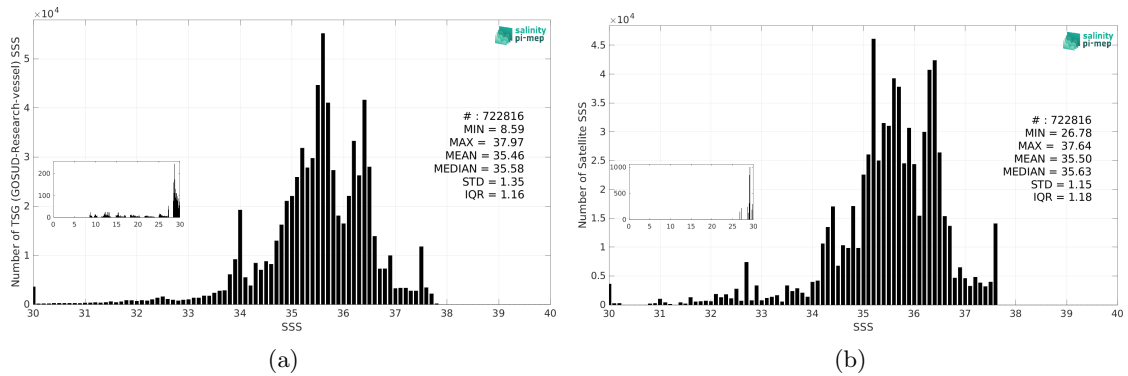
Figure 3: Histograms of SSS from TSG (GOSUD-Research-vessel) (a) and Aquarius SSS L3 CAP v5 - Monthly (JPL) (b) considering all match-up pairs per bins of 0.1 over the Global Ocean Pi-MEP region and for the full satellite product period.
