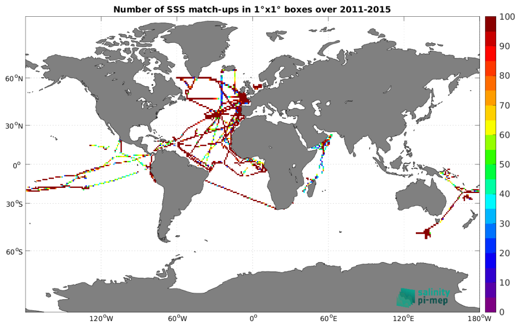
Figure 5: Number of SSS match-ups between TSG (GOSUD-Research-vessel) SSS and the Aquarius SSS L3 CAP v5 - Monthly (JPL) SSS product for the Global Ocean Pi-MEP region over 1^\circ \times 1^\circ boxes and for the full satellite product period.
