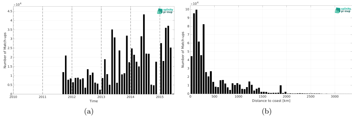
Figure 2: Number of match-ups between TSG (GOSUD-Research-vessel) and Aquarius SSS L3 CAP v5 - Monthly (JPL) SSS as a function of time (a) and as function of the distance to coast (b) over the Global Ocean Pi-MEP region and for the full satellite product period.
