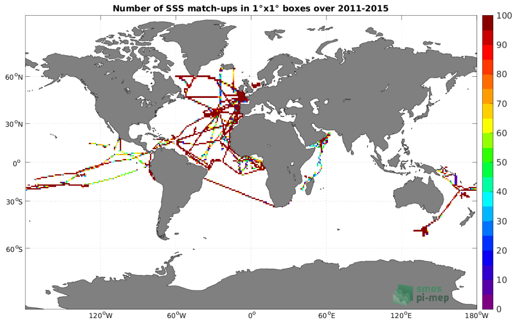
Figure 4: Number of SSS match-ups between TSG (GOSUD-Research-vessel) SSS and the Aquarius SSS L3 CAP v5 - Monthly (JPL) SSS product for the Global Ocean Pi-MEP region over 1^\circ \times 1^\circ boxes and for the full satellite product period.
