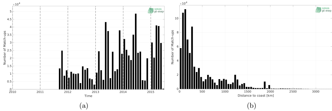
Figure 1: Number of match-ups between TSG (GOSUD-Research-vessel) and Aquarius SSS L3 CAP v5 - Monthly (JPL) SSS as a function of time (a) and as function of the distance to coast (b) over the Global Ocean Pi-MEP region and for the full satellite product period.
