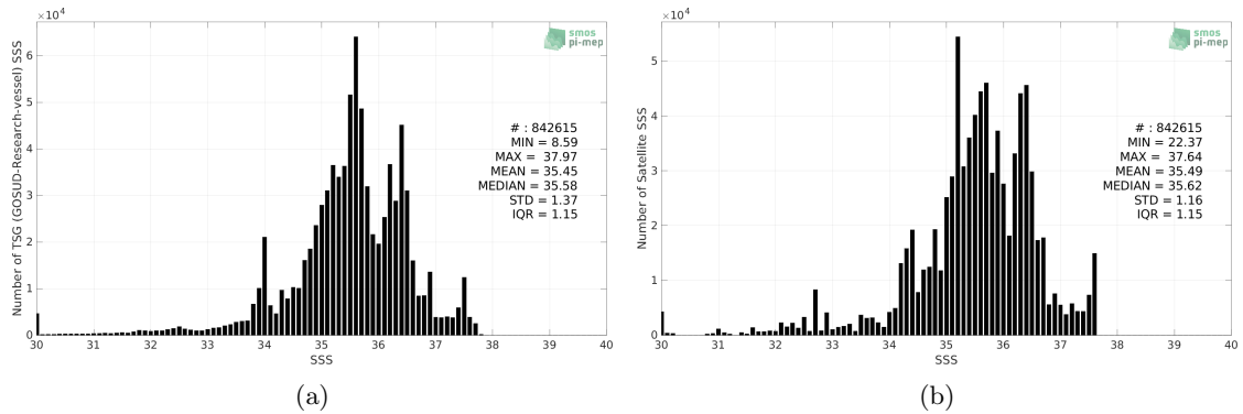
Figure 2: Histograms of SSS from TSG (GOSUD-Research-vessel) (a) and Aquarius SSS L3 CAP v5 - Monthly (JPL) (b) considering all match-up pairs per bins of 0.1 over the Global Ocean Pi-MEP region and for the full satellite product period.
