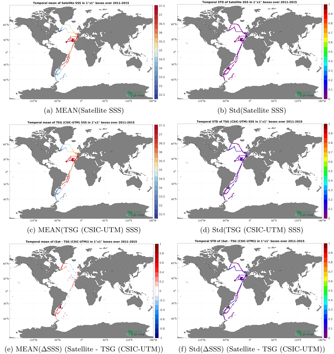
Figure 6: Temporal mean (left) and Std (right) of SSS from Aquarius SSS L3 CAP v5 - Monthly (JPL) (top), TSG (CSIC-UTM) (middle), and of \Delta SSS (Satellite - TSG (CSIC-UTM)). Only match-up pairs are used to generate these maps.
