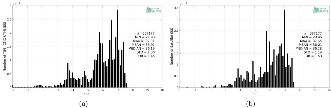
Figure 2: Histograms of SSS from TSG (CSIC-UTM) (a) and Aquarius SSS L3 CAP v5 - Monthly (JPL) (b) considering all match-up pairs per bins of 0.1 over the Global Ocean Pi-MEP region and for the full satellite product period.
