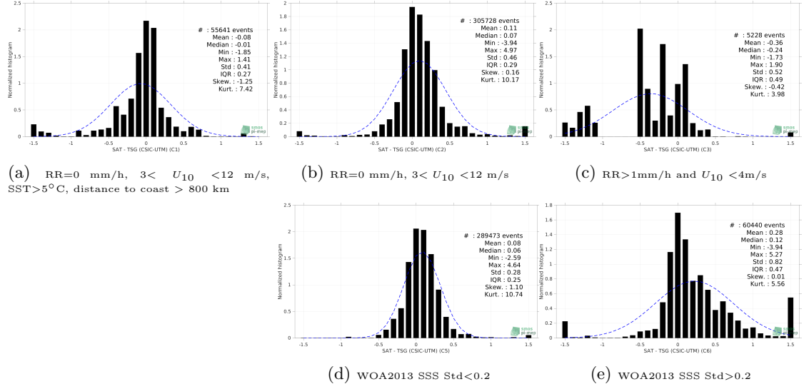
Figure 13: Normalized histogram of \Delta SSS (Aquarius SSS L3 CAP v5 - Monthly (JPL) - TSG (CSIC-UTM)) for 5 different subdatasets corresponding to: RR=0 mm/h, 3 < U_{10} < 12 m/s, SST>5°C, distance to coast > 800 km (a), RR=0 mm/h, 3 < U_{10} < 12 m/s (b), RR>1mm/h and U_{10} < 4 m/s (c), WOA2013 SSS Std<0.2 (d), WOA2013 SSS Std>0.2 (e).
