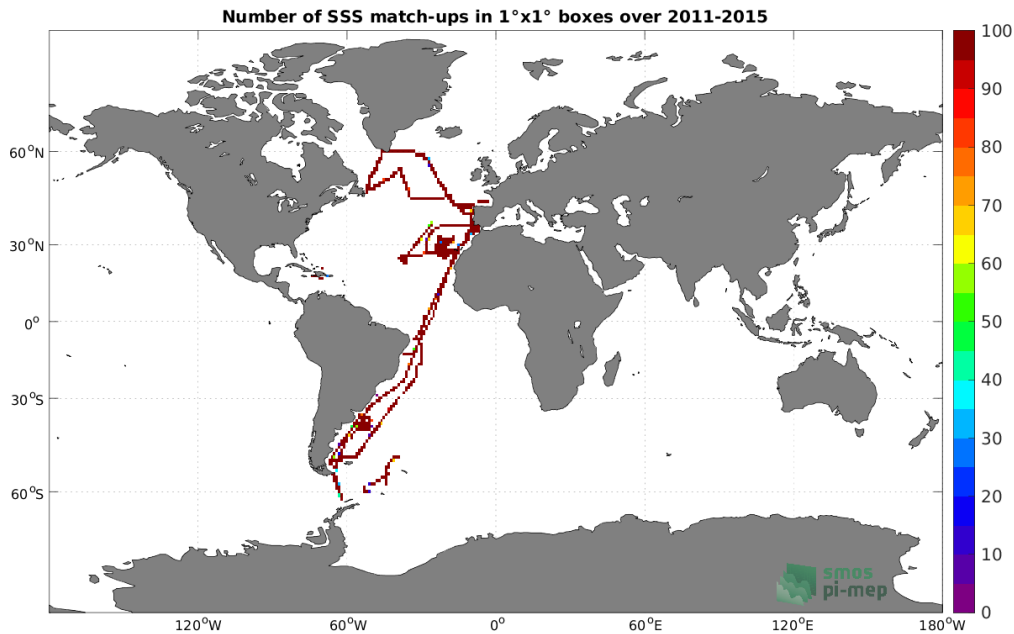
Figure 4: Number of SSS match-ups between TSG (CSIC-UTM) SSS and the Aquarius SSS L3 CAP v5 - Monthly (JPL) SSS product for the Global Ocean Pi-MEP region over 1^\circ \times 1^\circ boxes and for the full satellite product period.
