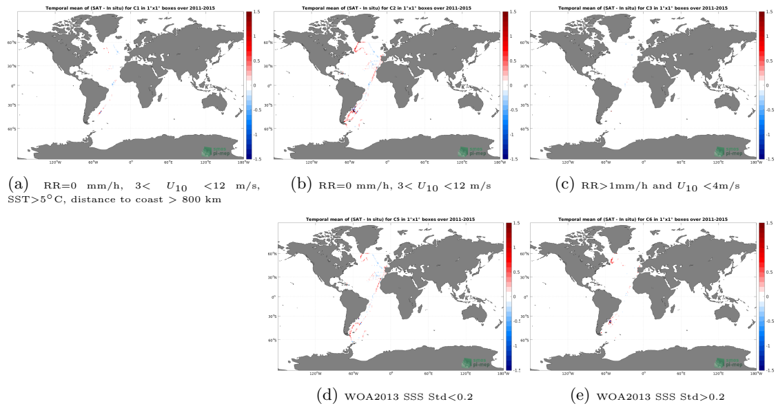
Figure 12: Temporal mean gridded over spatial boxes of size 1^\circ \times 1^\circ of \Delta SSS (Aquarius SSS L3 CAP v5 - Monthly (JPL) - TSG (CSIC-UTM)) for 5 different subdatasets corresponding to:RR=0 mm/h, 3 < U_{10} < 12 m/s, SST > 5^\circ\text{C} , distance to coast > 800 km (a), RR=0 mm/h, 3 < U_{10} < 12 m/s (b), RR > 1 mm/h and U_{10} < 4 m/s (c), WOA2013 SSS Std < 0.2 (d), WOA2013 SSS Std > 0.2 (e).
