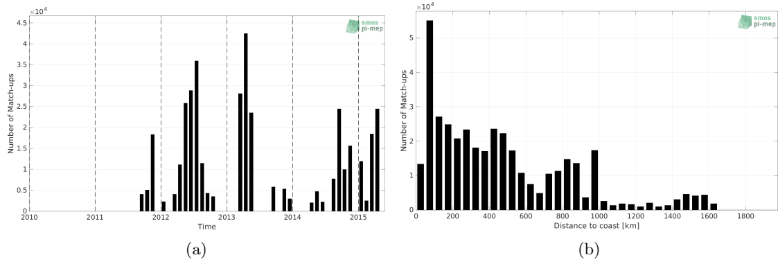
Figure 1: Number of match-ups between TSG (CSIC-UTM) and Aquarius SSS L3 CAP v5 - Monthly (JPL) SSS as a function of time (a) and as function of the distance to coast (b) over the Global Ocean Pi-MEP region and for the full satellite product period.
