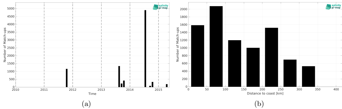
Figure 1: Number of match-ups between TSG (Amundsen) and Aquarius SSS L3 CAP v5 - Monthly (JPL) SSS as a function of time (a) and as function of the distance to coast (b) over the Global Ocean Pi-MEP region and for the full satellite product period.
