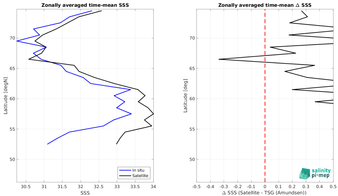
Figure 8: Left panel: Zonal mean SSS from Aquarius SSS L3 CAP v5 - Monthly (JPL) satellite product (black) and from TSG (Amundsen) (blue). Right panel: Zonal mean of \Delta SSS (Satellite - TSG (Amundsen)) for all the collected Pi-MEP match-up pairs estimated over the full satellite product period.
