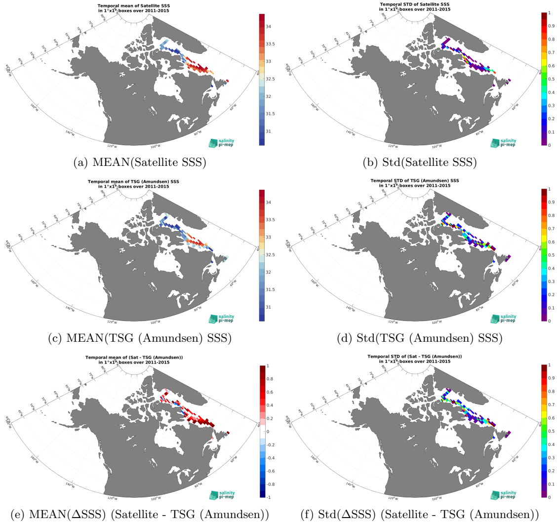
Figure 6: Temporal mean (left) and Std (right) of SSS from Aquarius SSS L3 CAP v5 - Monthly (JPL) (top), TSG (Amundsen) (middle), and of \Delta SSS (Satellite - TSG (Amundsen)). Only match-up pairs are used to generate these maps.
