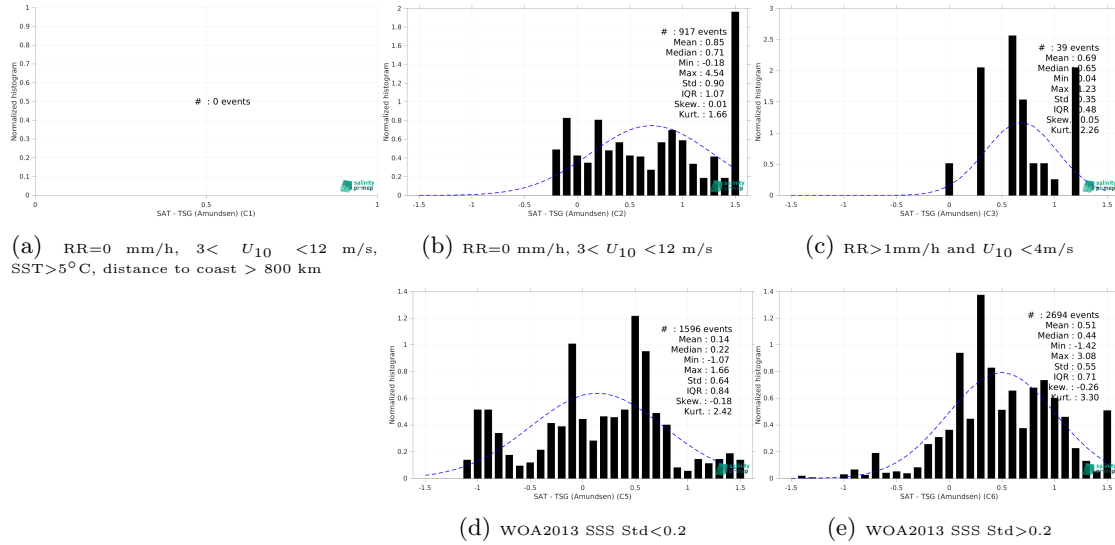
Figure 13: Normalized histogram of \Delta SSS (Aquarius SSS L3 CAP v5 - Monthly (JPL) - TSG (Amundsen)) for 5 different subdatasets corresponding to: RR=0 mm/h, 3 < U_{10} < 12 m/s, SST > 5°C, distance to coast > 800 km (a), RR=0 mm/h, 3 < U_{10} < 12 m/s (b), RR > 1mm/h and U_{10} < 4 m/s (c), WOA2013 SSS Std < 0.2 (d), WOA2013 SSS Std > 0.2 (e).
