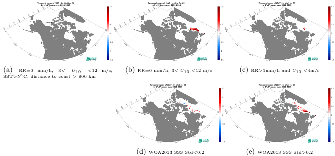
Figure 12: Temporal mean gridded over spatial boxes of size 1^{\circ}\times 1^{\circ} of \Delta\text{SSS} (Aquarius SSS L3 CAP v5 - Monthly (JPL) - TSG (Amundsen)) for 5 different subdatasets corresponding to:RR=0 mm/h, 3 < U_{10} < 12 m/s, SST >5^{\circ}\text{C} , distance to coast > 800 km (a), RR=0 mm/h, 3 < U_{10} < 12 m/s (b), RR >1 mm/h and U_{10} < 4 m/s (c), WOA2013 SSS Std <0.2 (d), WOA2013 SSS Std >0.2 (e).
