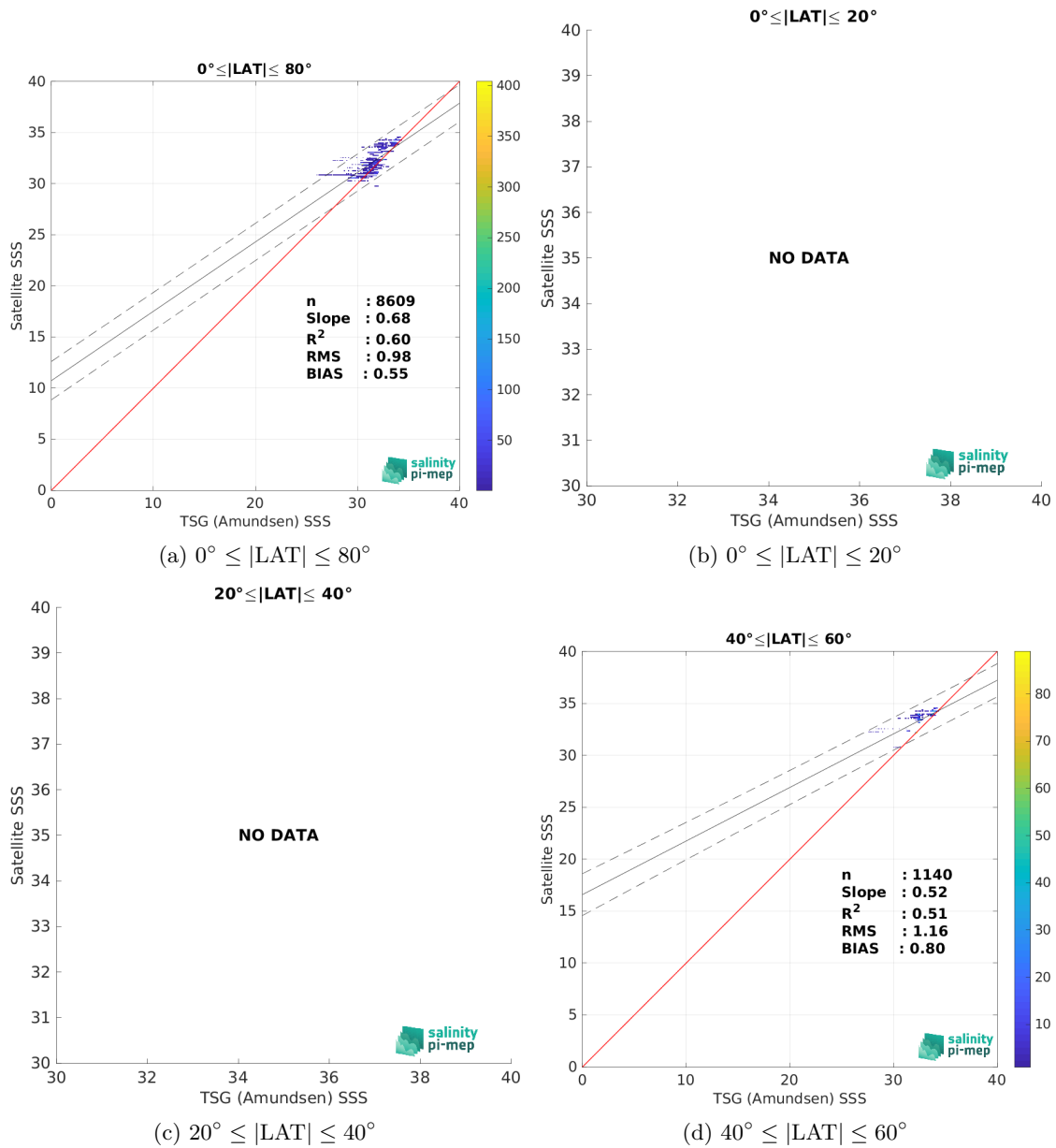
Figure 9: Contour maps of the concentration of Aquarius SSS L3 CAP v5 - Monthly (JPL) SSS (y-axis) versus TSG (Amundsen) SSS (x-axis) at match-up pairs for different latitude bands. For each plot, the red line shows x=y . The black thin and dashed lines indicate a linear fit through the data cloud and the \pm 95\% confidence levels, respectively. The number match-up pairs n , the slope and R^2 coefficient of the linear fit, the root mean square (RMS) and the mean bias between satellite and in situ data are indicated for each latitude band in each plots.
