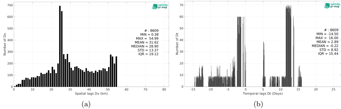
Figure 5: Histograms of the spatial (a) and temporal (b) lags between the location/time of the TSG (Amundsen) measurement and the date of the corresponding Aquarius SSS L3 CAP v5 - Monthly (JPL) SSS pixel.
