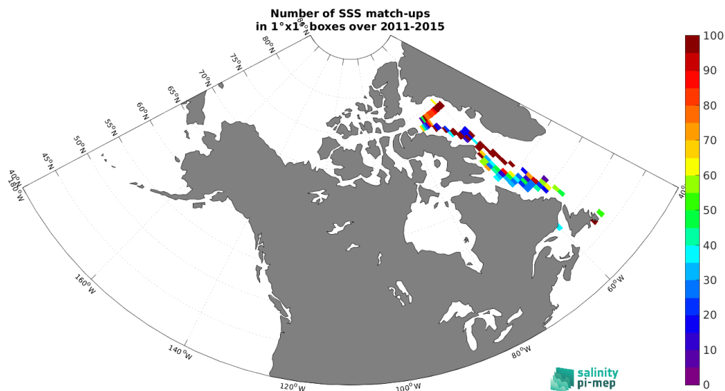
Figure 4: Number of SSS match-ups between TSG (Amundsen) SSS and the Aquarius SSS L3 CAP v5 - Monthly (JPL) SSS product for the Global Ocean Pi-MEP region over 1^\circ \times 1^\circ boxes and for the full satellite product period.
