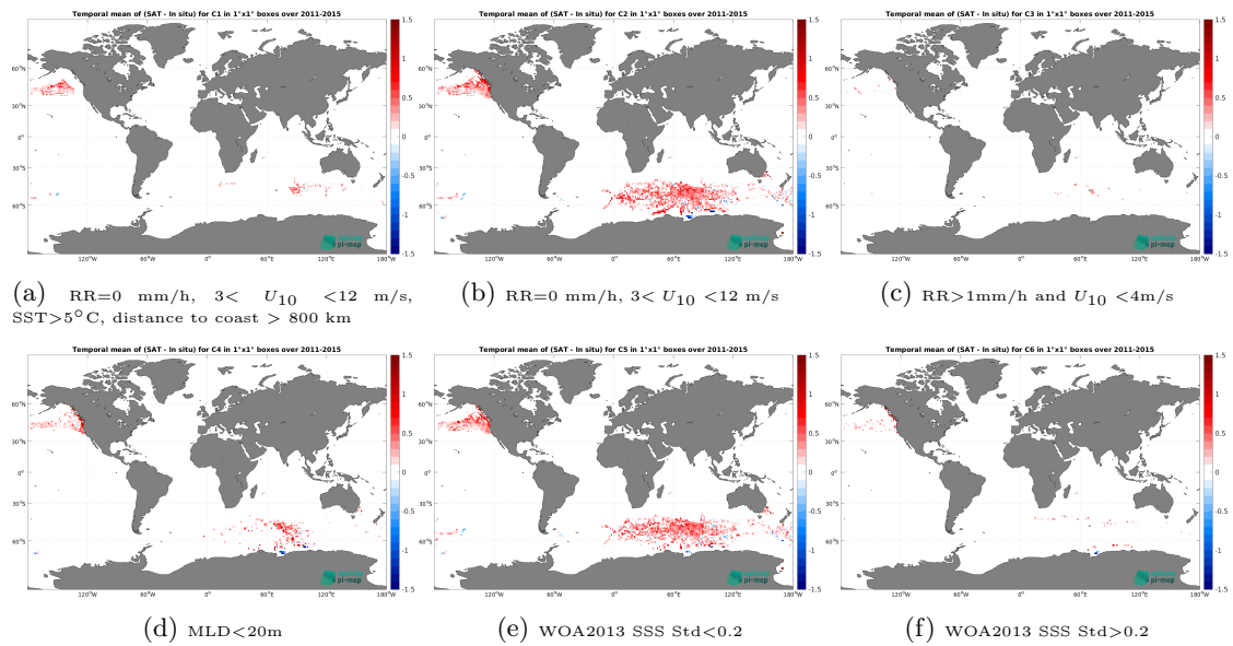
Figure 14: Temporal mean gridded over spatial boxes of size 1^\circ \times 1^\circ of \Delta\text{SSS} (Aquarius SSS L3 CAP v5 - Monthly (JPL) - Marine mammals) for 6 different subdatasets corresponding to:RR=0 mm/h, 3 < U_{10} < 12 m/s, SST>5°C, distance to coast > 800 km (a), RR=0 mm/h, 3 < U_{10} < 12 m/s (b), RR>1mm/h and U_{10} < 4 m/s (c),MLD<20m (d),WOA2013 SSS Std<0.2 (e),WOA2013 SSS Std>0.2 (f).
