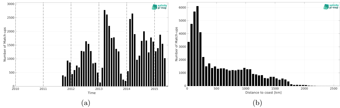
Figure 2: Number of match-ups between Marine mammals and Aquarius SSS L3 CAP v5 - Monthly (JPL) SSS as a function of time (a) and as function of the distance to coast (b) over the Global Ocean Pi-MEP region and for the full satellite product period.
