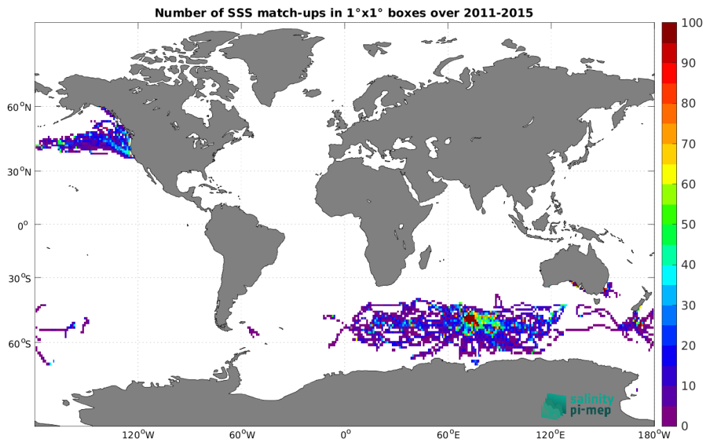
Figure 5: Number of SSS match-ups between Marine mammals SSS and the Aquarius SSS L3 CAP v5 - Monthly (JPL) SSS product for the Global Ocean Pi-MEP region over 1^\circ \times 1^\circ boxes and for the full satellite product period.
