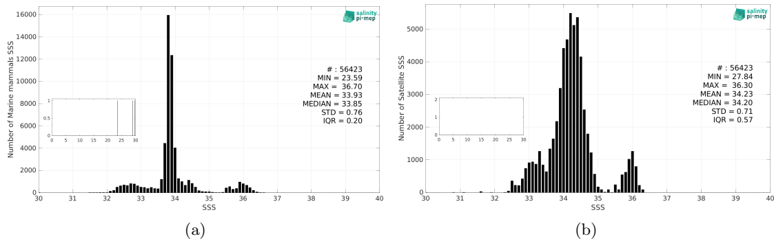
Figure 3: Histograms of SSS from Marine mammals (a) and Aquarius SSS L3 CAP v5 - Monthly (JPL) (b) considering all match-up pairs per bins of 0.1 over the Global Ocean Pi-MEP region and for the full satellite product period.
