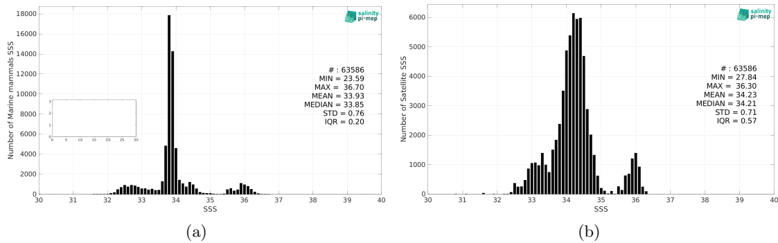
Figure 2: Histograms of SSS from Marine mammals (a) and Aquarius SSS L3 CAP v5 - Monthly (JPL) (b) considering all match-up pairs per bins of 0.1 over the Global Ocean Pi-MEP region and for the full satellite product period.
