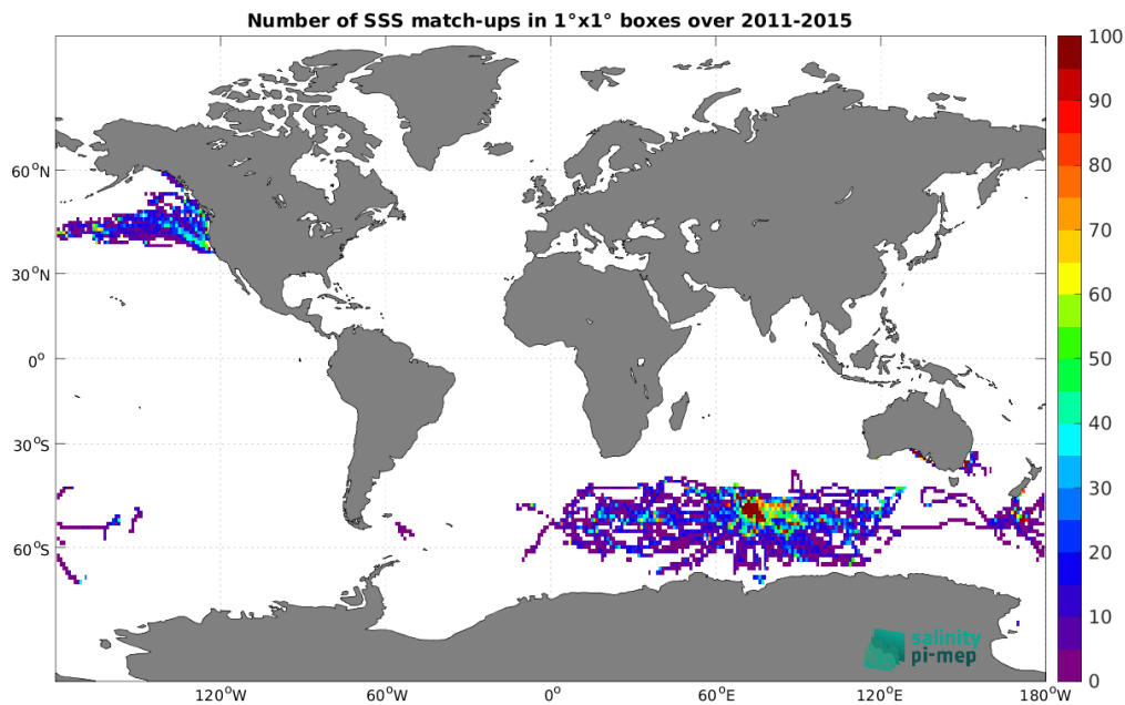
Figure 4: Number of SSS match-ups between Marine mammals SSS and the Aquarius SSS L3 CAP v5 - Monthly (JPL) SSS product for the Global Ocean Pi-MEP region over 1^\circ \times 1^\circ boxes and for the full satellite product period.
