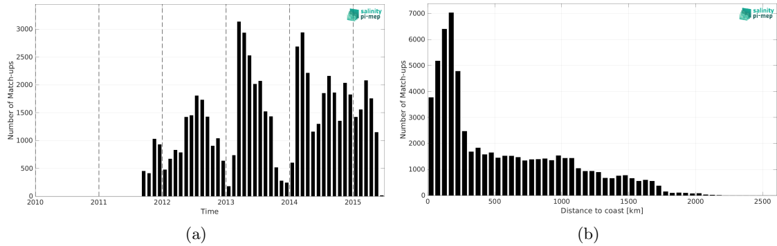
Figure 1: Number of match-ups between Marine mammals and Aquarius SSS L3 CAP v5 - Monthly (JPL) SSS as a function of time (a) and as function of the distance to coast (b) over the Global Ocean Pi-MEP region and for the full satellite product period.
