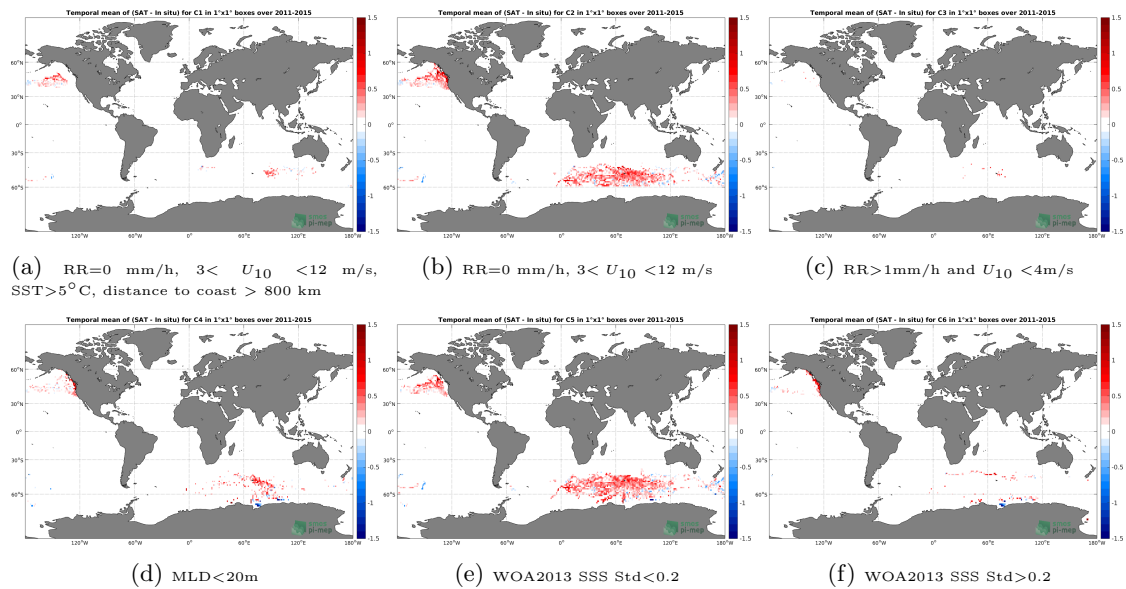
Figure 12: Temporal mean gridded over spatial boxes of size 1^\circ \times 1^\circ of \Delta SSS (Aquarius-L3-JPL-V5-MONTHLY - Sea mammals) for 6 different subdatasets corresponding to:RR=0 mm/h, 3 < U_{10} < 12 m/s, SST >5^\circ C, distance to coast > 800 km (a), RR=0 mm/h, 3 < U_{10} < 12 m/s (b), RR >1 mm/h and U_{10} < 4 m/s (c),MLD <20 m (d),WOA2013 SSS Std <0.2 (e),WOA2013 SSS Std >0.2 (f).
