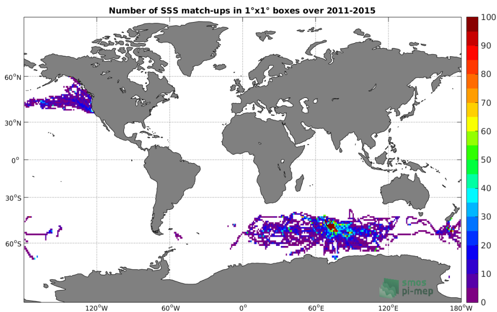
Figure 4: Number of SSS match-ups between Sea mammals SSS and the Aquarius-L3-JPL-V5-MONTHLY SSS product for the Global Ocean Pi-MEP region over 1°x1° boxes and for the full satellite product period.
