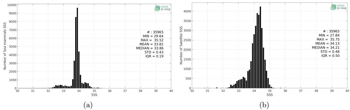
Figure 2: Histograms of SSS from Sea mammals (a) and Aquarius-L3-JPL-V5-MONTHLY (b) considering all match-up pairs per bins of 0.1 over the Global Ocean Pi-MEP region and for the full satellite product period.
