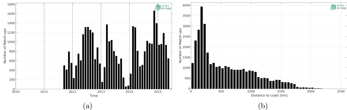
Figure 1: Number of match-ups between Sea mammals and Aquarius-L3-JPL-V5-MONTHLY SSS as a function of time (a) and as function of the distance to coast (b) over the Global Ocean Pi-MEP region and for the full satellite product period.
