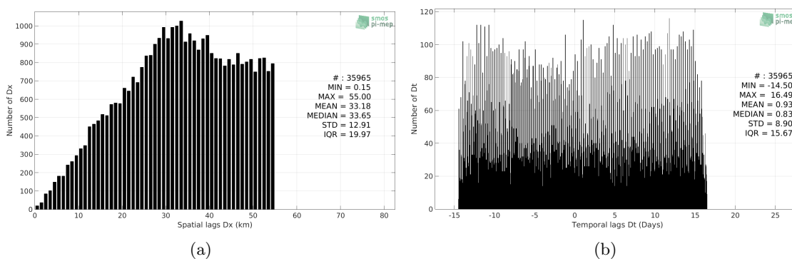
Figure 5: Histograms of the spatial (a) and temporal (b) lags between the time of the Sea mammals measurements and the date of the corresponding Aquarius-L3-JPL-V5-MONTHLY SSS product.
