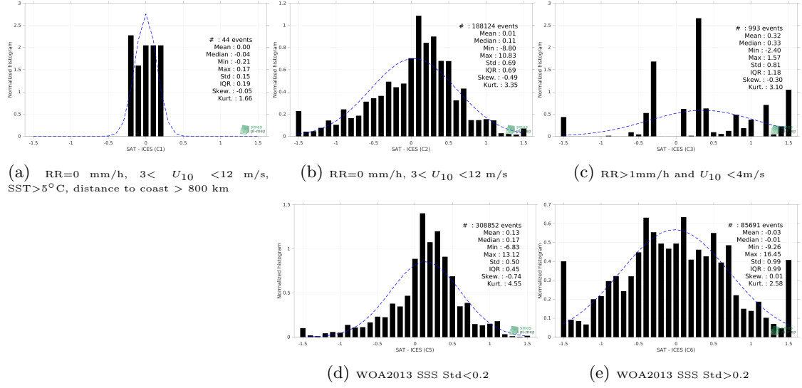
Figure 13: Normalized histogram of \Delta SSS (Aquarius SSS L3 CAP v5 - Monthly (JPL) - ICES) for 5 different subdatasets corresponding to: RR=0 mm/h, 3 < U_{10} < 12 m/s, SST > 5°C, distance to coast > 800 km (a), RR=0 mm/h, 3 < U_{10} < 12 m/s (b), RR > 1mm/h and U_{10} < 4 m/s (c), WOA2013 SSS Std < 0.2 (d), WOA2013 SSS Std > 0.2 (e).
