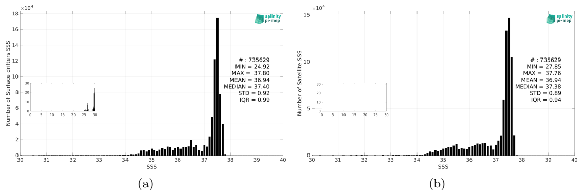
Figure 3: Histograms of SSS from Surface drifters (a) and Aquarius SSS L3 CAP v5 - Monthly (JPL) (b) considering all match-up pairs per bins of 0.1 over the Global Ocean Pi-MEP region and for the full satellite product period.
