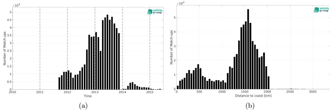
Figure 2: Number of match-ups between Surface drifters and Aquarius SSS L3 CAP v5 - Monthly (JPL) SSS as a function of time (a) and as function of the distance to coast (b) over the Global Ocean Pi-MEP region and for the full satellite product period.
