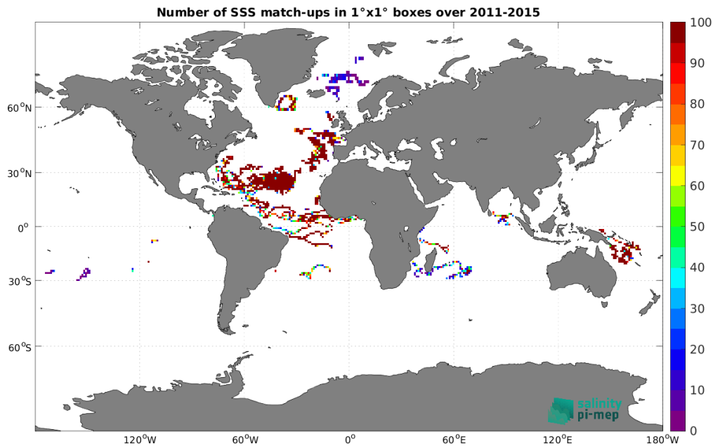
Figure 4: Number of SSS match-ups between Surface drifters SSS and the Aquarius SSS L3 CAP v5 - Monthly (JPL) SSS product for the Global Ocean Pi-MEP region over 1^\circ \times 1^\circ boxes and for the full satellite product period.
