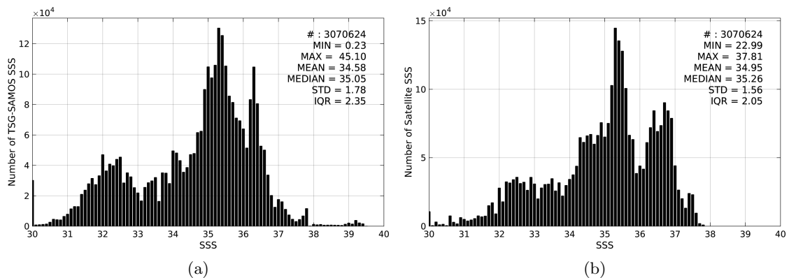
Figure 2: Histograms of SSS from TSG-SAMOS (a) and Aquarius-L3-JPL-V4-7DAY-RUNNING (b) considering all match-up pairs per bins of 0.1 over the Global Ocean Pi-MEP region and for the full satellite product period.
