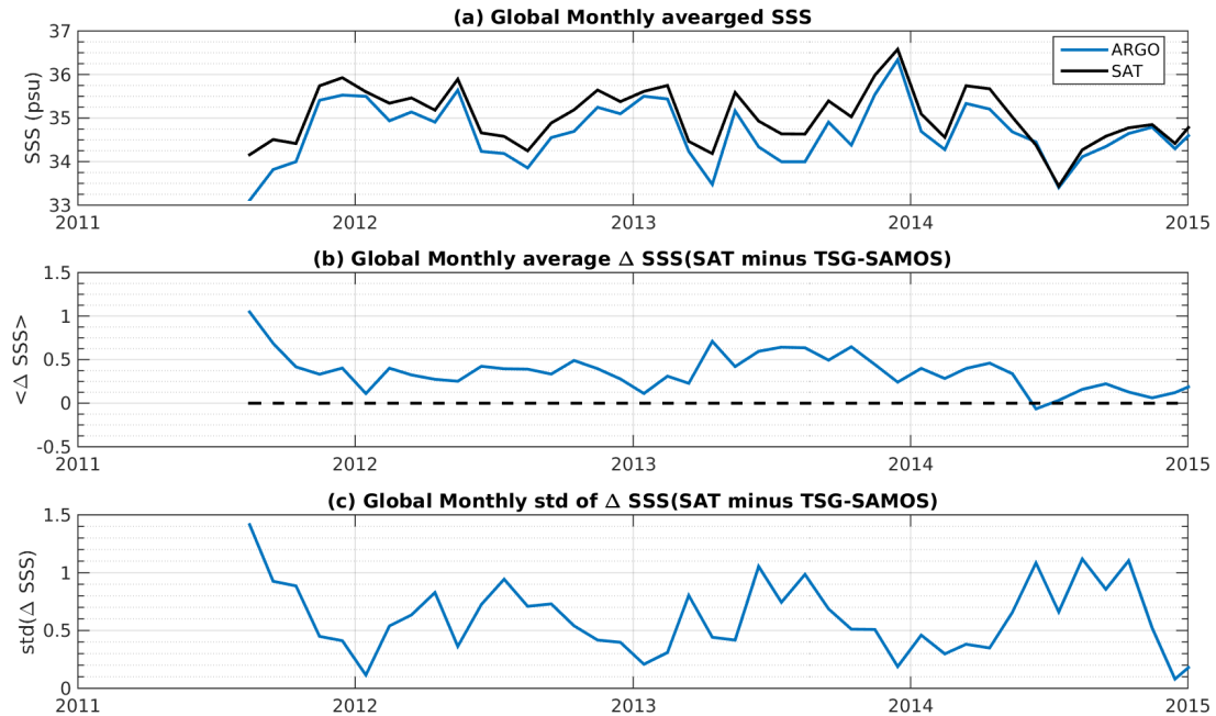
Figure 7: Time series of the monthly averaged mean SSS (top), mean \Delta SSS (Satellite - TSG-SAMOS) and STD of \Delta SSS (Satellite - TSG-SAMOS) over the Global Ocean Pi-MEP region considering all match-ups collected by the Pi-MEP platform.
