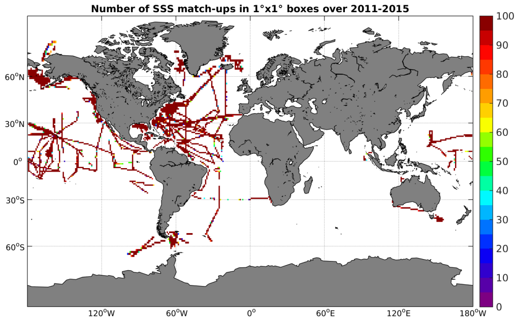
Figure 4: Number of SSS match-ups between TSG-SAMOS SSS and the Aquarius-L3-JPL-V4-7DAY-RUNNING SSS product for the Global Ocean Pi-MEP region over 1^\circ \times 1^\circ boxes and for the full satellite product period.
