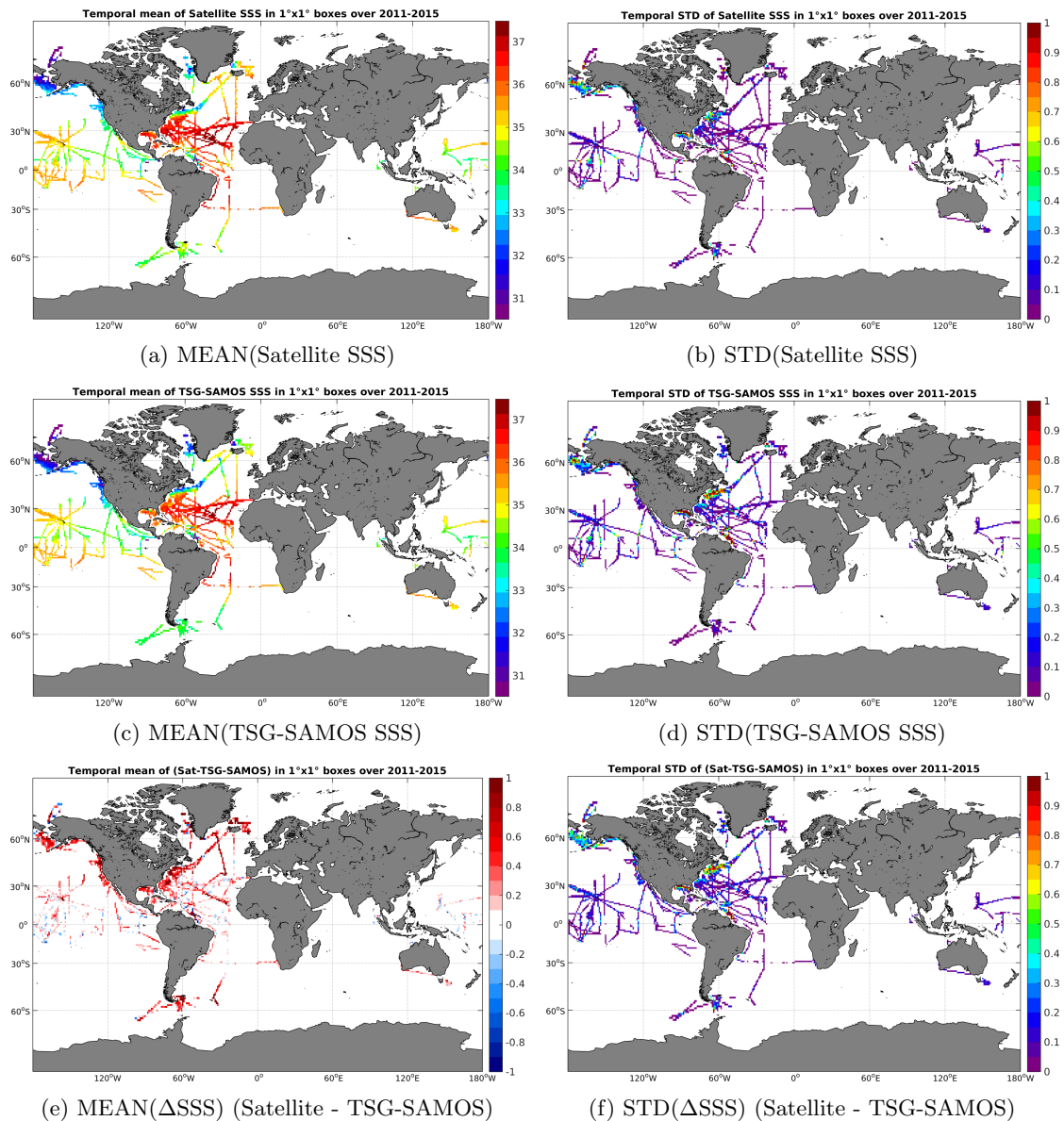
Figure 6: Temporal mean (left) and STD (right) of SSS from Aquarius-L3-JPL-V4-7DAY-RUNNING (top), TSG-SAMOS (middle), and of \Delta SSS (Satellite - TSG-SAMOS). Only match-up pairs are used to generate these maps.
