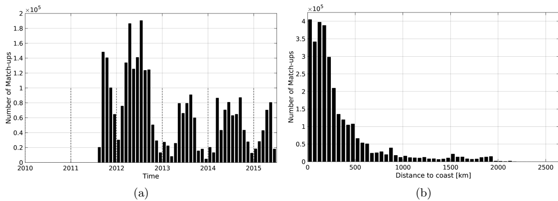
Figure 1: Number of match-ups between TSG-SAMOS and Aquarius-L3-JPL-V4-7DAY-RUNNING SSS as a function of time (a) and as function of the distance to coast (b) over the Global Ocean Pi-MEP region and for the full satellite product period.
