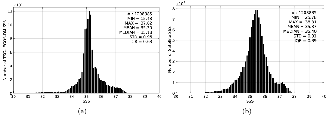
Figure 2: Histograms of SSS from TSG-LEGOS-DM (a) and Aquarius-L3-JPL-V4-7DAY-RUNNING (b) considering all match-up pairs per bins of 0.1 over the Global Ocean Pi-MEP region and for the full satellite product period.
