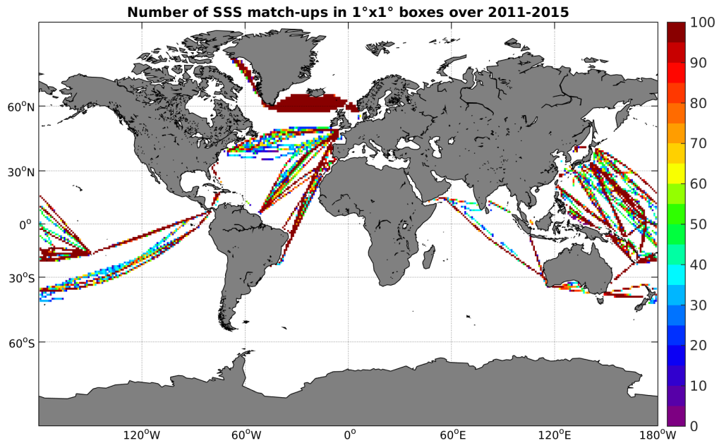
Figure 4: Number of SSS match-ups between TSG-LEGOS-DM SSS and the Aquarius-L3-JPL-V4-7DAY-RUNNING SSS product for the Global Ocean Pi-MEP region over 1^\circ \times 1^\circ boxes and for the full satellite product period.
