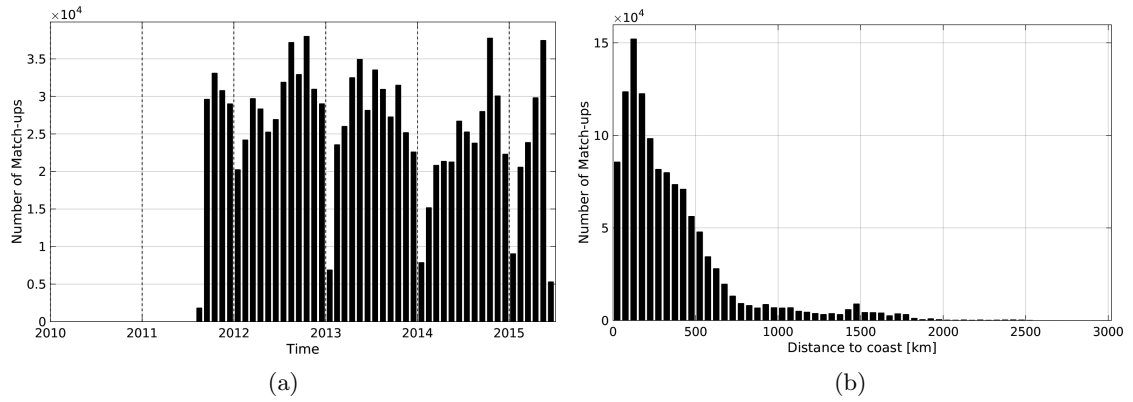
Figure 1: Number of match-ups between TSG-LEGOS-DM and Aquarius-L3-JPL-V4-7DAY-RUNNING SSS as a function of time (a) and as function of the distance to coast (b) over the Global Ocean Pi-MEP region and for the full satellite product period.
