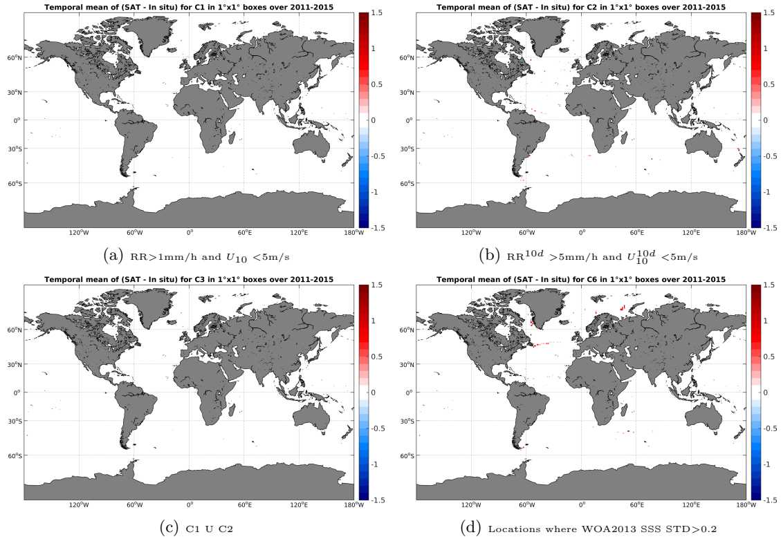
Figure 12: Temporal mean gridded over spatial boxes of size 1^\circ \times 1^\circ of \Delta SSS (Aquarius-L3-JPL-V4-7DAY-RUNNING - TSG-GOSUD-Sailing-ship) for 4 different subdatasets corresponding to: RR > 1mm/h and U_{10} < 5\text{m/s} (a), RR^{10d} > 5\text{mm/h} and U_{10}^{10d} < 5\text{m/s} (b), C1 U C2 (c), Locations where WOA2013 SSS STD > 0.2 (d).
