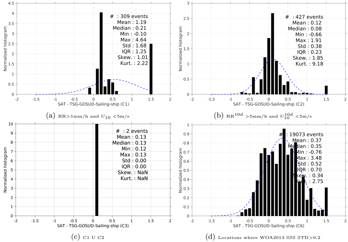
Figure 13: Normalized histogram of \Delta SSS (Aquarius-L3-JPL-V4-7DAY-RUNNING - TSG-GOSUD-Sailing-ship) for 6 different subdatasets corresponding to: RR > 1mm/h and U_{10} < 5 m/s (a), RR^{10d} > 5 mm/h and U_{10}^{10d} < 5 m/s (b), C1 U C2 (c), Locations where WOA2013 SSS STD > 0.2 (d).
