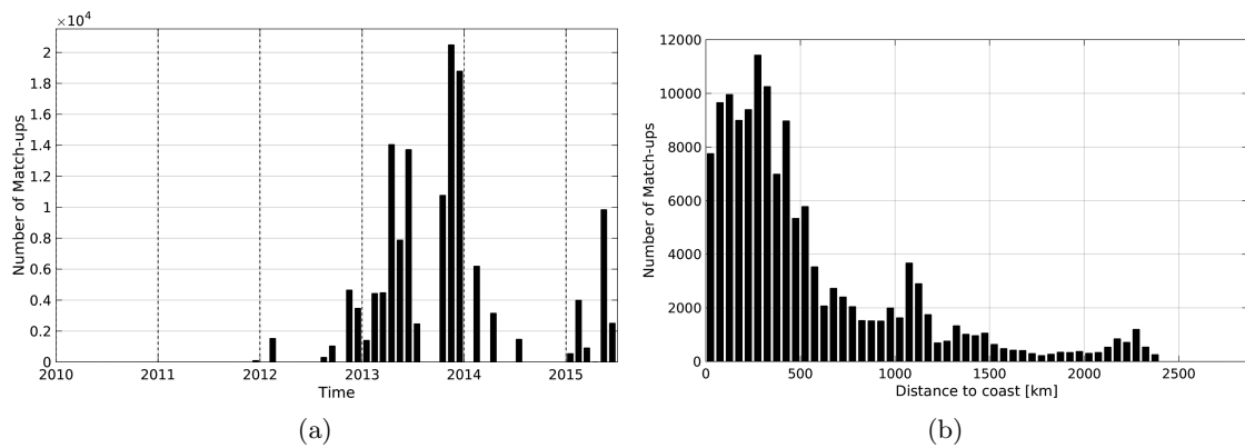
Figure 1: Number of match-ups between TSG-GOSUD-Sailing-ship and Aquarius-L3-JPL-V4-7DAY-RUNNING SSS as a function of time (a) and as function of the distance to coast (b) over the Global Ocean Pi-MEP region and for the full satellite product period.
