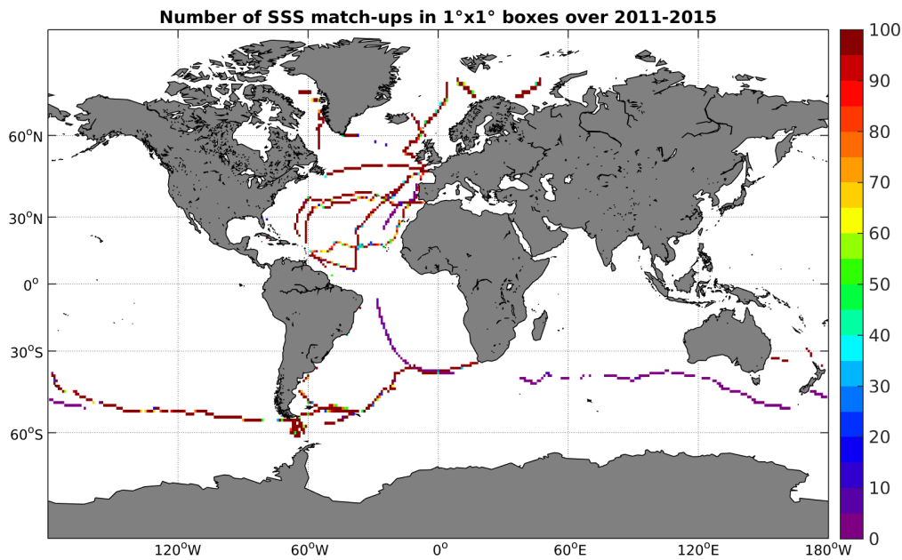
Figure 4: Number of SSS match-ups between TSG-GOSUD-Sailing-ship SSS and the Aquarius-L3-JPL-V4-7DAY-RUNNING SSS product for the Global Ocean Pi-MEP region over 1^\circ \times 1^\circ boxes and for the full satellite product period.
