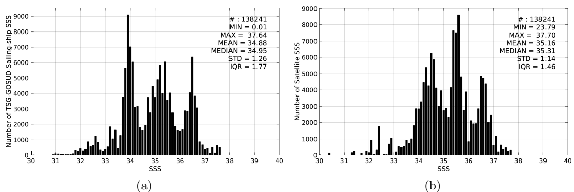
Figure 2: Histograms of SSS from TSG-GOSUD-Sailing-ship (a) and Aquarius-L3-JPL-V4-7DAY-RUNNING (b) considering all match-up pairs per bins of 0.1 over the Global Ocean Pi-MEP region and for the full satellite product period.
