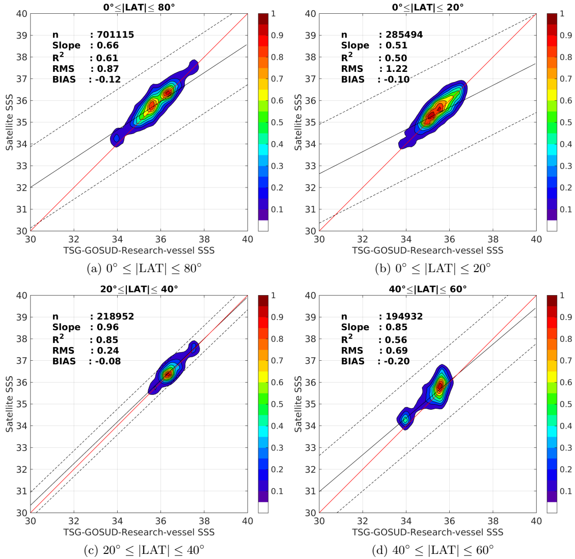
Figure 9: Contour maps of the concentration of Aquarius-L3-JPL-V4-7DAY-RUNNING SSS (y-axis) versus TSG-GOSUD-Research-vessel SSS (x-axis) at match-up pairs for different latitude bands. For each plot, the red line shows x=y . The black thin and dashed lines indicate a linear fit through the data cloud and the \pm 95\% confidence levels, respectively. The number match-up pairs n , the slope and R^2 coefficient of the linear fit, the root mean square (RMS) and the mean bias between satellite and in situ data are indicated for each latitude band in each plots.
