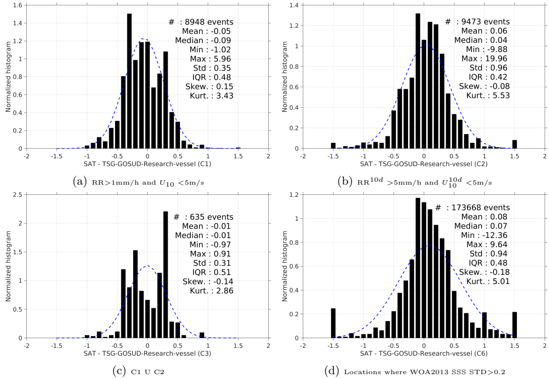
Figure 13: Normalized histogram of \Delta SSS (Aquarius-L3-JPL-V4-7DAY-RUNNING - TSG-GOSUD-Research-vessel) for 6 different subdatasets corresponding to: RR > 1mm/h and U_{10} < 5\text{m/s} (a), RR^{10d} > 5\text{mm/h} and U_{10}^{10d} < 5\text{m/s} (b), C1 U C2 (c), Locations where WOA2013 SSS STD > 0.2 (d).
