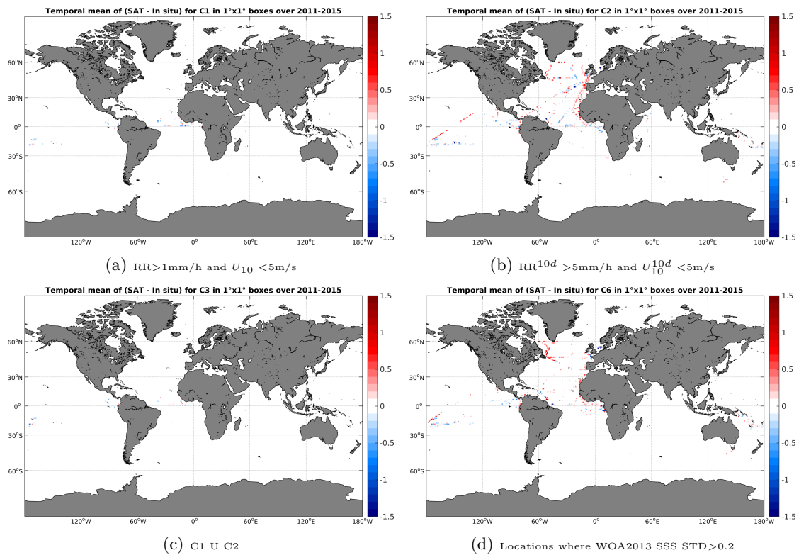
Figure 12: Temporal mean gridded over spatial boxes of size 1^\circ \times 1^\circ of \Delta SSS (Aquarius-L3-JPL-V4-7DAY-RUNNING - TSG-GOSUD-Research-vessel) for 4 different subdatasets corresponding to:RR > 1 mm/h and U_{10} < 5 m/s (a), RR^{10d} > 5 mm/h and U_{10}^{10d} < 5 m/s (b), C1 U C2 (c),Locations where WOA2013 SSS STD > 0.2 (d).
