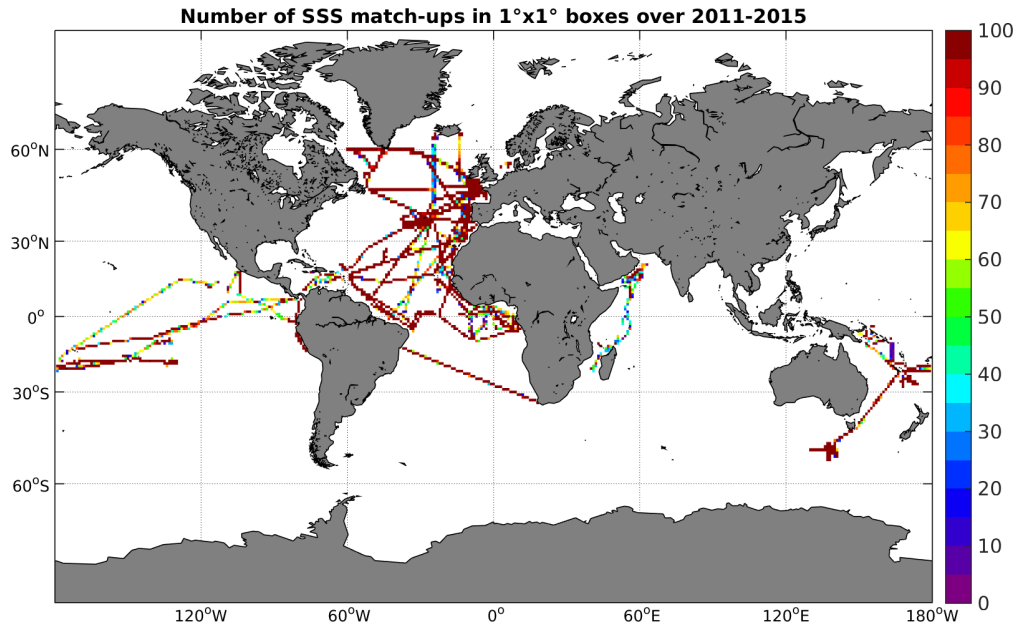
Figure 4: Number of SSS match-ups between TSG-GOSUD-Research-vessel SSS and the Aquarius-L3-JPL-V4-7DAY-RUNNING SSS product for the Global Ocean Pi-MEP region over 1°x1° boxes and for the full satellite product period.
