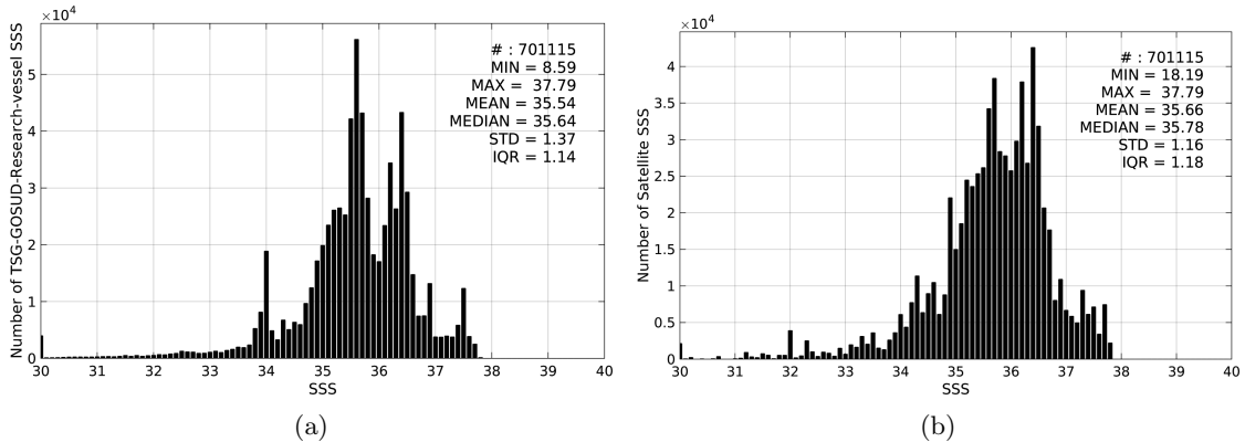
Figure 2: Histograms of SSS from TSG-GOSUD-Research-vessel (a) and Aquarius-L3-JPL-V4-7DAY-RUNNING (b) considering all match-up pairs per bins of 0.1 over the Global Ocean Pi-MEP region and for the full satellite product period.
