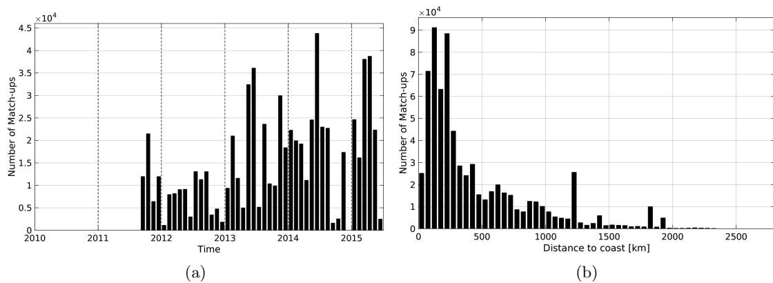
Figure 1: Number of match-ups between TSG-GOSUD-Research-vessel and Aquarius-L3-JPL-V4-7DAY-RUNNING SSS as a function of time (a) and as function of the distance to coast (b) over the Global Ocean Pi-MEP region and for the full satellite product period.
