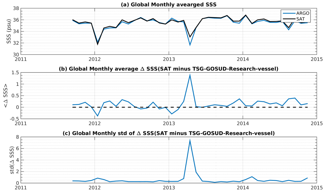
Figure 7: Time series of the monthly averaged mean SSS (top), mean \Delta SSS (Satellite - TSG-GOSUD-Research-vessel) and STD of \Delta SSS (Satellite - TSG-GOSUD-Research-vessel) over the Global Ocean Pi-MEP region considering all match-ups collected by the Pi-MEP platform.
