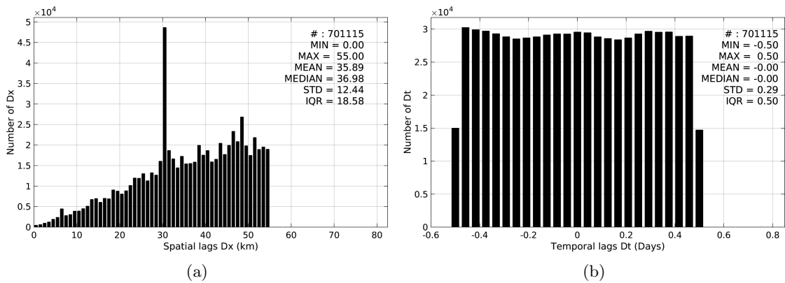
Figure 5: Histograms of the spatial (a) and temporal (b) lags between the time of the TSG-GOSUD-Research-vessel measurements and the date of the corresponding Aquarius-L3-JPL-V4-7DAY-RUNNING SSS product.
