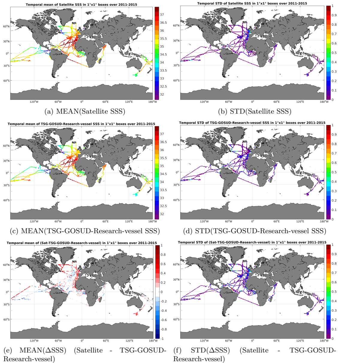
Figure 6: Temporal mean (left) and STD (right) of SSS from Aquarius-L3-JPL-V4-7DAY-RUNNING (top), TSG-GOSUD-Research-vessel (middle), and of \Delta SSS (Satellite - TSG-GOSUD-Research-vessel). Only match-up pairs are used to generate these maps.
