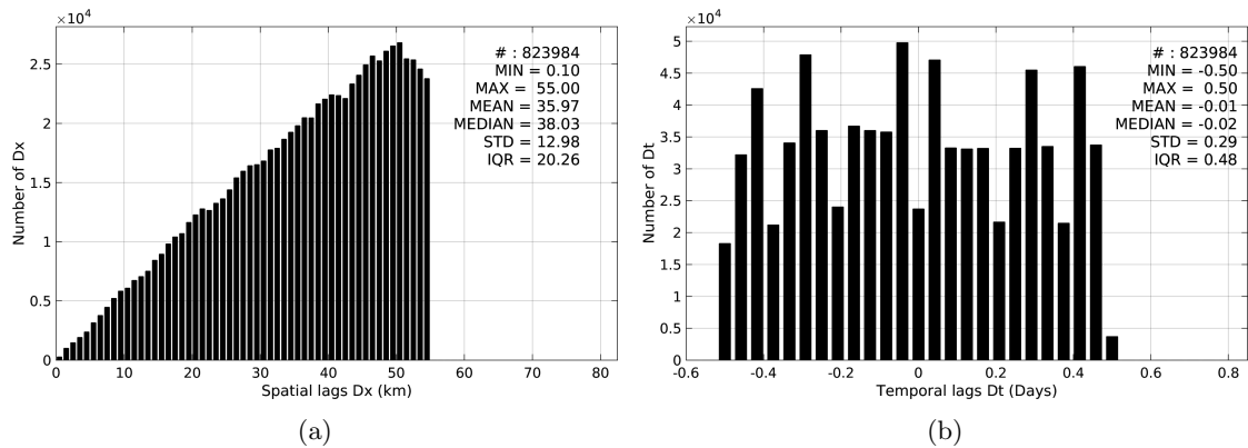
Figure 4: Histograms of the spatial (a) and temporal (b) lags between the time of the Surface drifters measurements and the date of the corresponding Aquarius-L3-JPL-V4-7DAY-RUNNING SSS product.
