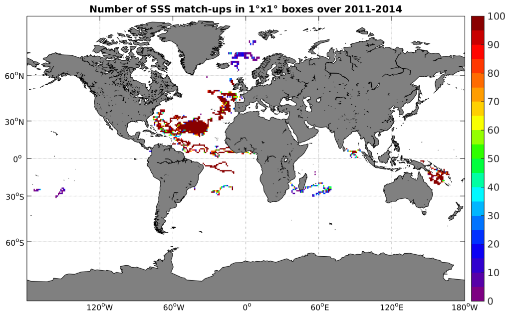
Figure 3: Number of SSS match-ups between Surface drifters SSS and the Aquarius-L3-JPL-V4-7DAY-RUNNING SSS product for the Global Ocean Pi-MEP region over 1^\circ \times 1^\circ boxes and for the full satellite product period.
