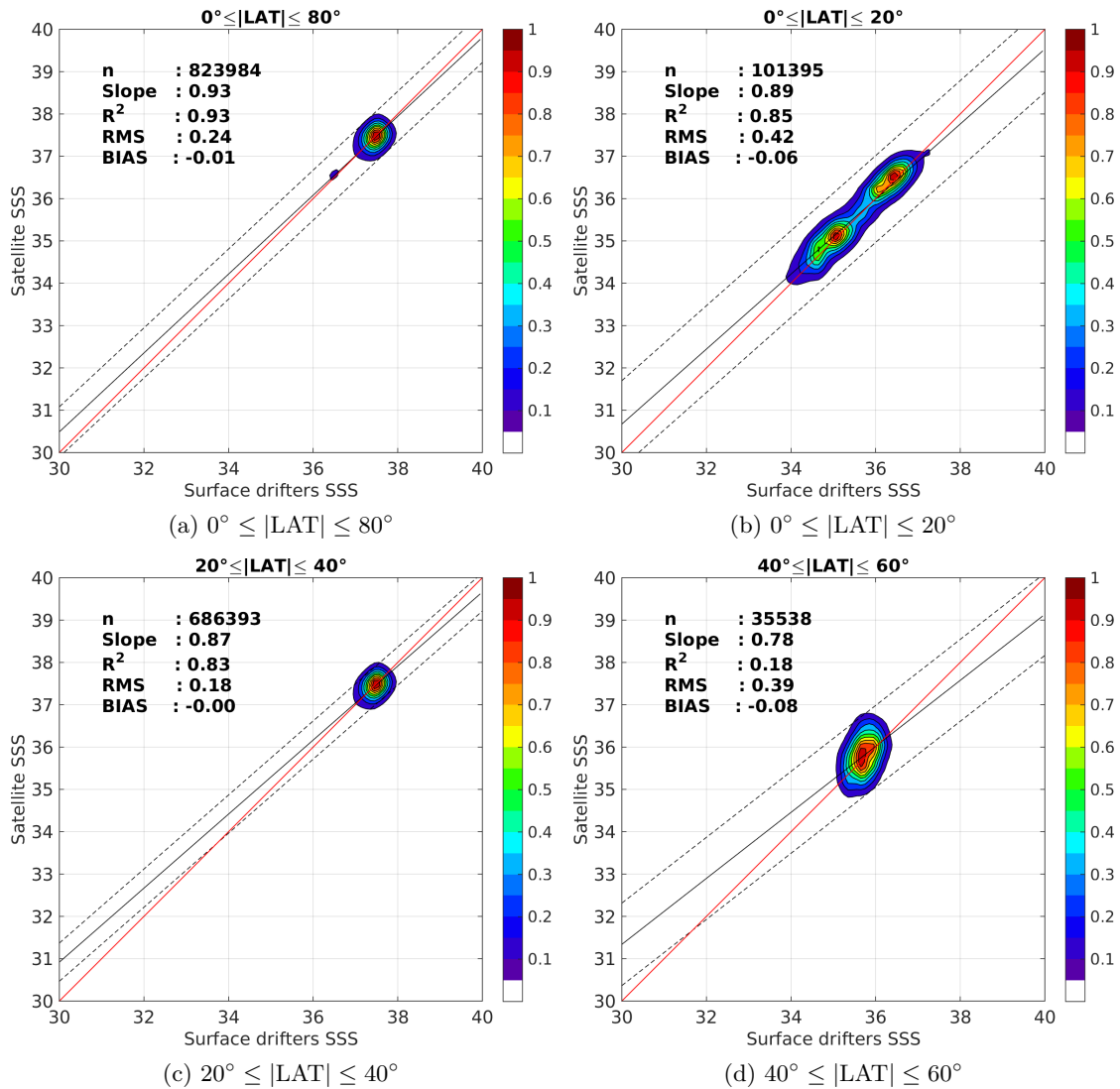
Figure 8: Contour maps of the concentration of Aquarius-L3-JPL-V4-7DAY-RUNNING SSS (y-axis) versus Surface drifters SSS (x-axis) at match-up pairs for different latitude bands. For each plot, the red line shows x=y . The black thin and dashed lines indicate a linear fit through the data cloud and the \pm 95\% confidence levels, respectively. The number match-up pairs n , the slope and R^2 coefficient of the linear fit, the root mean square (RMS) and the mean bias between satellite and in situ data are indicated for each latitude band in each plots.
