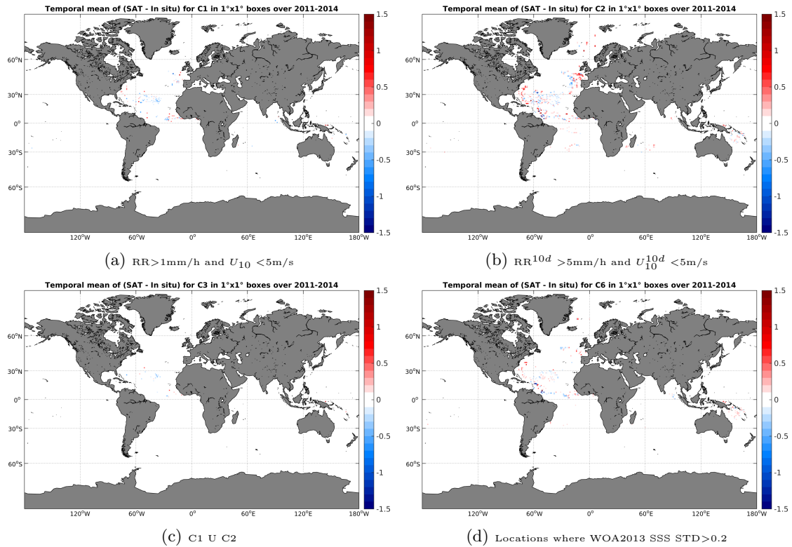
Figure 11: Temporal mean gridded over spatial boxes of size 1^\circ \times 1^\circ of \Delta SSS (Aquarius-L3-JPL-V4-7DAY-RUNNING - Surface drifters) for 4 different subdatasets corresponding to: RR > 1\text{mm/h} and U_{10} < 5\text{m/s} (a), RR^{10d} > 5\text{mm/h} and U_{10}^{10d} < 5\text{m/s} (b), C1 U C2 (c), Locations where WOA2013 SSS STD > 0.2 (d).
