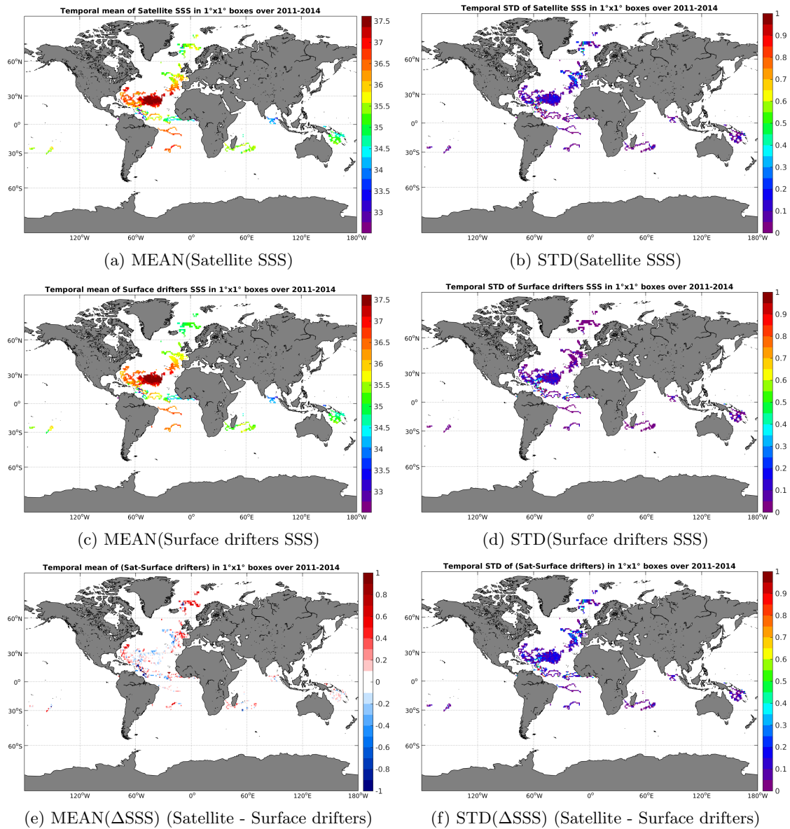
Figure 5: Temporal mean (left) and STD (right) of SSS from Aquarius-L3-JPL-V4-7DAY-RUNNING (top), Surface drifters (middle), and of \Delta SSS (Satellite - Surface drifters). Only match-up pairs are used to generate these maps.
