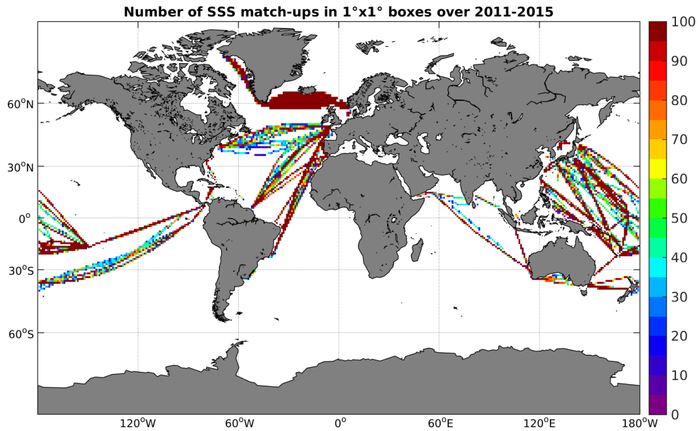
Figure 4: Number of SSS match-ups between TSG-LEGOS-DM SSS and the Aquarius-L3-JPL-V4-MONTHLY SSS product for the Global Ocean Pi-MEP region over 1^\circ \times 1^\circ boxes and for the full satellite product period.
