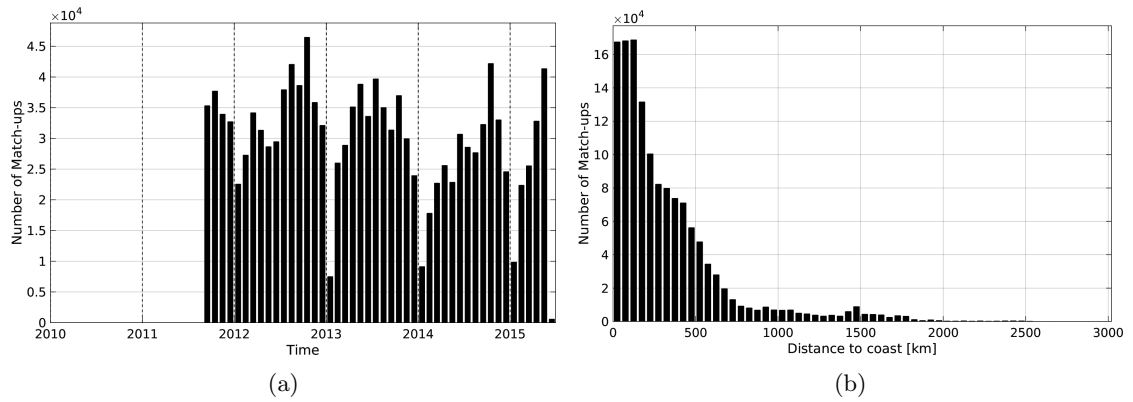
Figure 1: Number of match-ups between TSG-LEGOS-DM and Aquarius-L3-JPL-V4-MONTHLY SSS as a function of time (a) and as function of the distance to coast (b) over the Global Ocean Pi-MEP region and for the full satellite product period.
