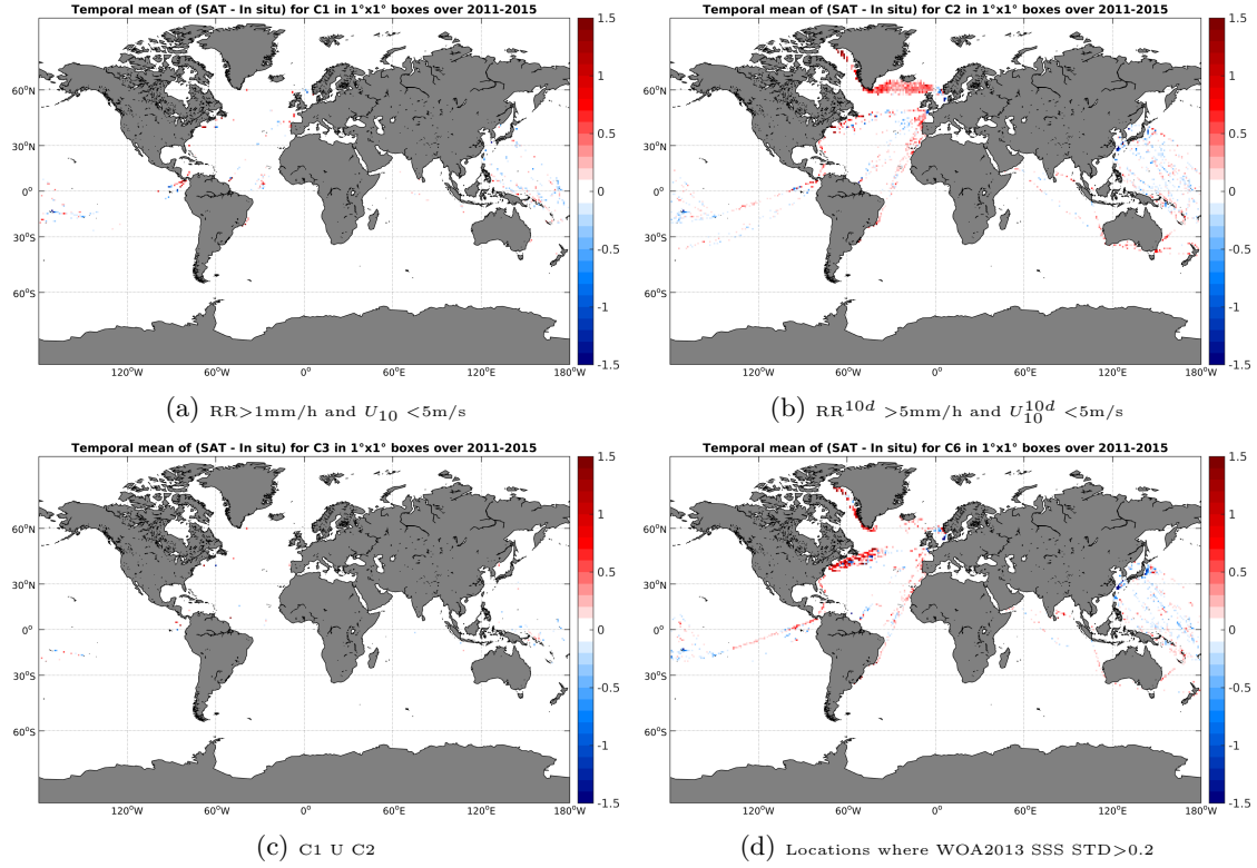
Figure 12: Temporal mean gridded over spatial boxes of size 1^\circ \times 1^\circ of \Delta SSS (Aquarius-L3-JPL-V4-MONTHLY - TSG-LEGOS-DM) for 4 different subdatasets corresponding to: RR > 1\text{mm/h} and U_{10} < 5\text{m/s} (a), RR^{10d} > 5\text{mm/h} and U_{10}^{10d} < 5\text{m/s} (b), C1 U C2 (c), Locations where WOA2013 SSS STD > 0.2 (d).
