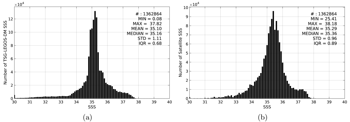
Figure 2: Histograms of SSS from TSG-LEGOS-DM (a) and Aquarius-L3-JPL-V4-MONTHLY (b) considering all match-up pairs per bins of 0.1 over the Global Ocean Pi-MEP region and for the full satellite product period.
