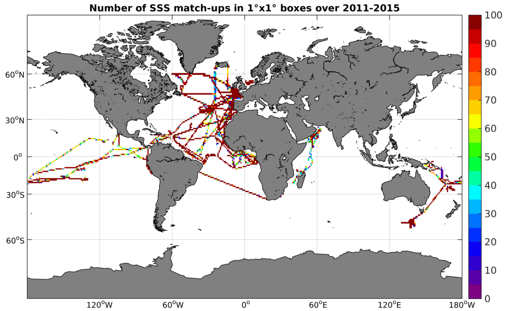
Figure 4: Number of SSS match-ups between TSG-GOSUD-Research-vessel SSS and the Aquarius-L3-JPL-V4-MONTHLY SSS product for the Global Ocean Pi-MEP region over 1^\circ \times 1^\circ boxes and for the full satellite product period.
