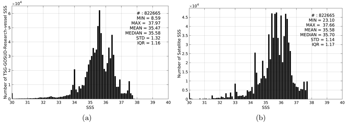
Figure 2: Histograms of SSS from TSG-GOSUD-Research-vessel (a) and Aquarius-L3-JPL-V4-MONTHLY (b) considering all match-up pairs per bins of 0.1 over the Global Ocean Pi-MEP region and for the full satellite product period.
