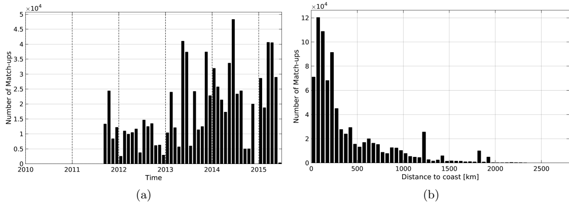
Figure 1: Number of match-ups between TSG-GOSUD-Research-vessel and Aquarius-L3-JPL-V4-MONTHLY SSS as a function of time (a) and as function of the distance to coast (b) over the Global Ocean Pi-MEP region and for the full satellite product period.
