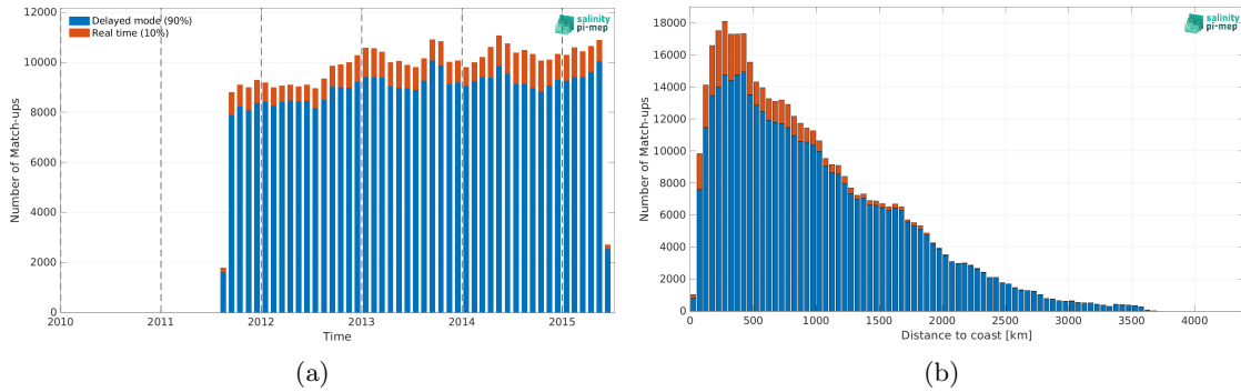
Figure 1: Number of match-ups between Argo and Aquarius SSS L2-AVERAGED OR v5 (NASA-GSFC) SSS as a function of time (a) and as function of the distance to coast (b) over the Global Ocean Pi-MEP region and for the full satellite product period.
