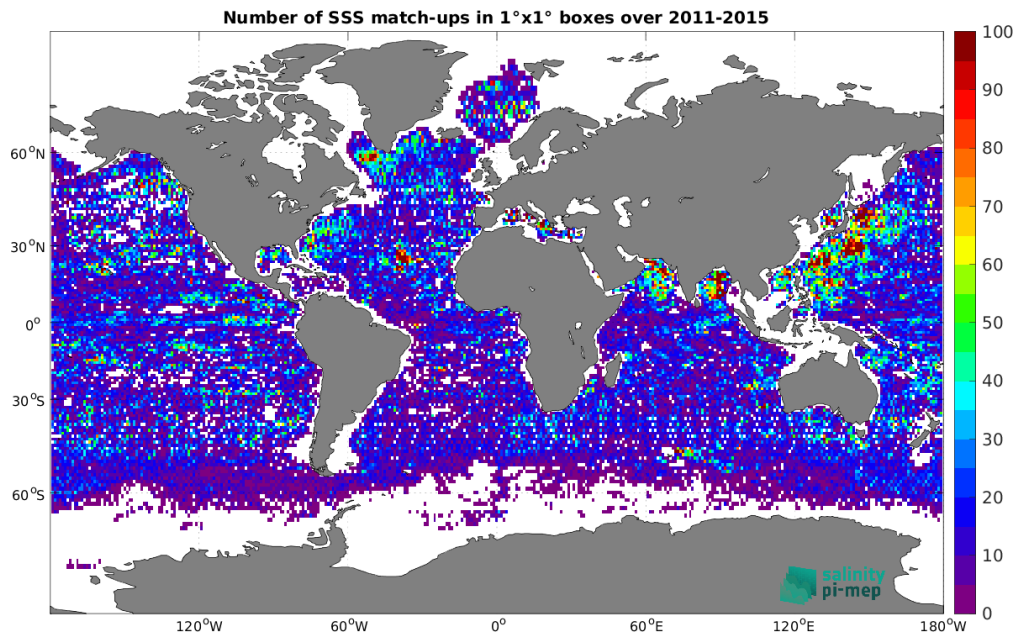
Figure 4: Number of SSS match-ups between Argo SSS and the Aquarius SSS L2-AVERAGED OR v5 (NASA-GSFC) SSS product for the Global Ocean Pi-MEP region over 1^\circ \times 1^\circ boxes and for the full satellite product period.
