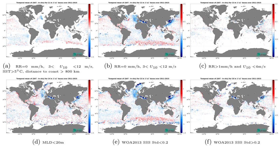
Figure 12: Temporal mean gridded over spatial boxes of size 1^\circ \times 1^\circ of \Delta SSS (Aquarius SSS L2-AVERAGED OR v5 (NASA-GSFC) - Argo) for 6 different subdatasets corresponding to:RR=0 mm/h, 3 < U_{10} < 12 m/s, SST >5^\circ C, distance to coast > 800 km (a), RR=0 mm/h, 3 < U_{10} < 12 m/s (b), RR >1 mm/h and U_{10} < 4 m/s (c),MLD <20 m (d),WOA2013 SSS Std <0.2 (e),WOA2013 SSS Std >0.2 (f).
