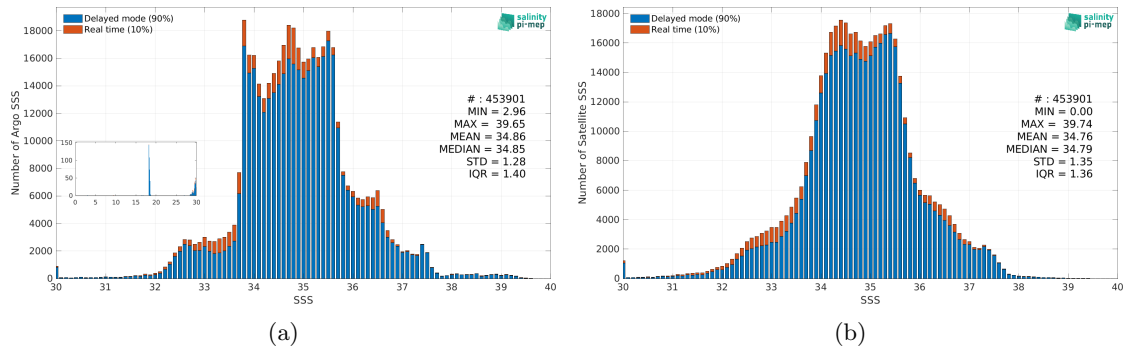
Figure 2: Histograms of SSS from Argo (a) and Aquarius SSS L2-AVERAGED OR v5 (NASA-GSFC) (b) considering all match-up pairs per bins of 0.1 over the Global Ocean Pi-MEP region and for the full satellite product period.
