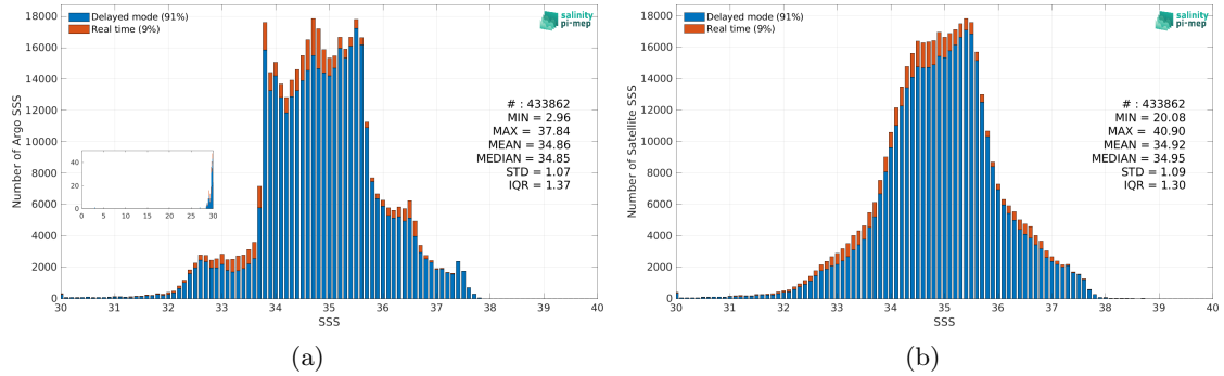
Figure 2: Histograms of SSS from Argo (a) and Aquarius SSS L2-AVERAGED CAP v5 (JPL) (b) considering all match-up pairs per bins of 0.1 over the Global Ocean Pi-MEP region and for the full satellite product period.
