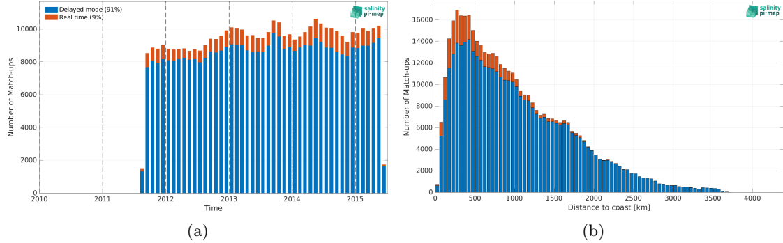
Figure 1: Number of match-ups between Argo and Aquarius SSS L2-AVERAGED CAP v5 (JPL) SSS as a function of time (a) and as function of the distance to coast (b) over the Global Ocean Pi-MEP region and for the full satellite product period.
