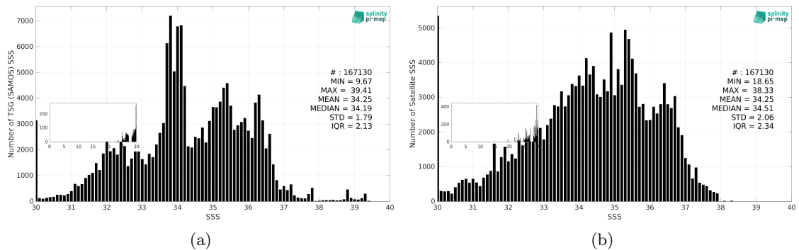
Figure 3: Histograms of SSS from TSG (SAMOS) (a) and Aquarius SSS L2 OR v5 (NASA-GSFC) (b) considering all match-up pairs per bins of 0.1 over the Global Ocean Pi-MEP region and for the full satellite product period.
