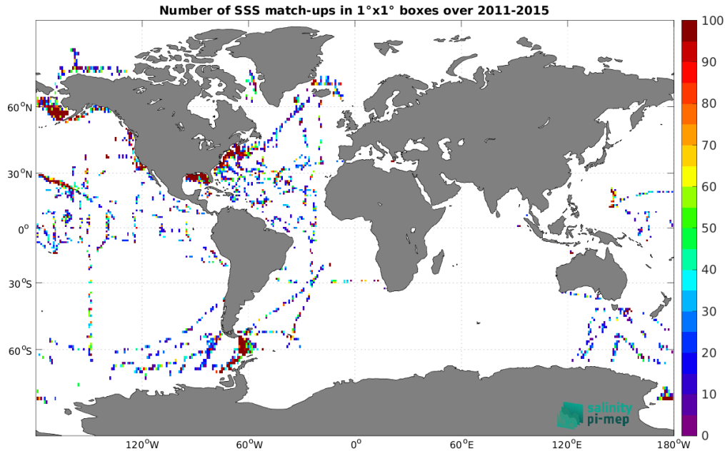
Figure 5: Number of SSS match-ups between TSG (SAMOS) SSS and the Aquarius SSS L2 OR v5 (NASA-GSFC) SSS product for the Global Ocean Pi-MEP region over 1^\circ \times 1^\circ boxes and for the full satellite product period.
