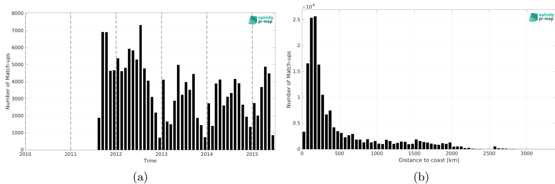
Figure 2: Number of match-ups between TSG (SAMOS) and Aquarius SSS L2 OR v5 (NASA-GSFC) SSS as a function of time (a) and as function of the distance to coast (b) over the Global Ocean Pi-MEP region and for the full satellite product period.
