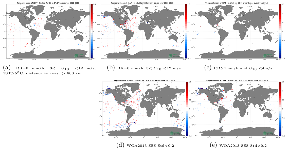
Figure 12: Temporal mean gridded over spatial boxes of size 1^\circ \times 1^\circ of \Delta\text{SSS} (Aquarius SSS L2 OR v5 (NASA-GSFC) - TSG (SAMOS)) for 5 different subdatasets corresponding to:RR=0 mm/h, 3 < U_{10} < 12 m/s, SST > 5^\circ\text{C} , distance to coast > 800 km (a), RR=0 mm/h, 3 < U_{10} < 12 m/s (b), RR > 1 mm/h and U_{10} < 4 m/s (c), WOA2013 SSS Std < 0.2 (d), WOA2013 SSS Std > 0.2 (e).
