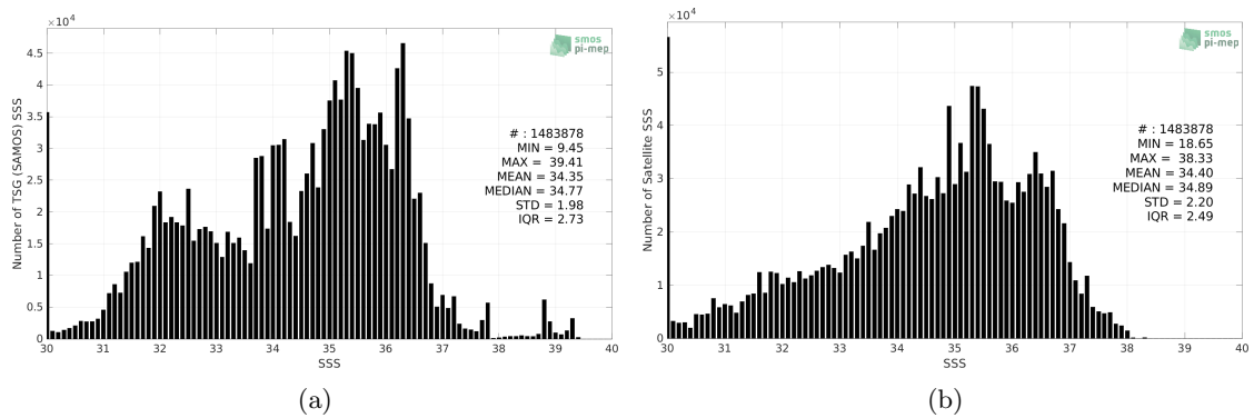
Figure 2: Histograms of SSS from TSG (SAMOS) (a) and Aquarius SSS L2 OR v5 (NASA-GSFC) (b) considering all match-up pairs per bins of 0.1 over the Global Ocean Pi-MEP region and for the full satellite product period.
