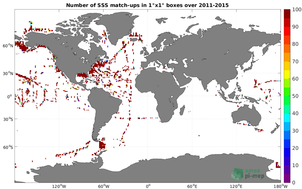
Figure 4: Number of SSS match-ups between TSG (SAMOS) SSS and the Aquarius SSS L2 OR v5 (NASA-GSFC) SSS product for the Global Ocean Pi-MEP region over 1^\circ \times 1^\circ boxes and for the full satellite product period.
