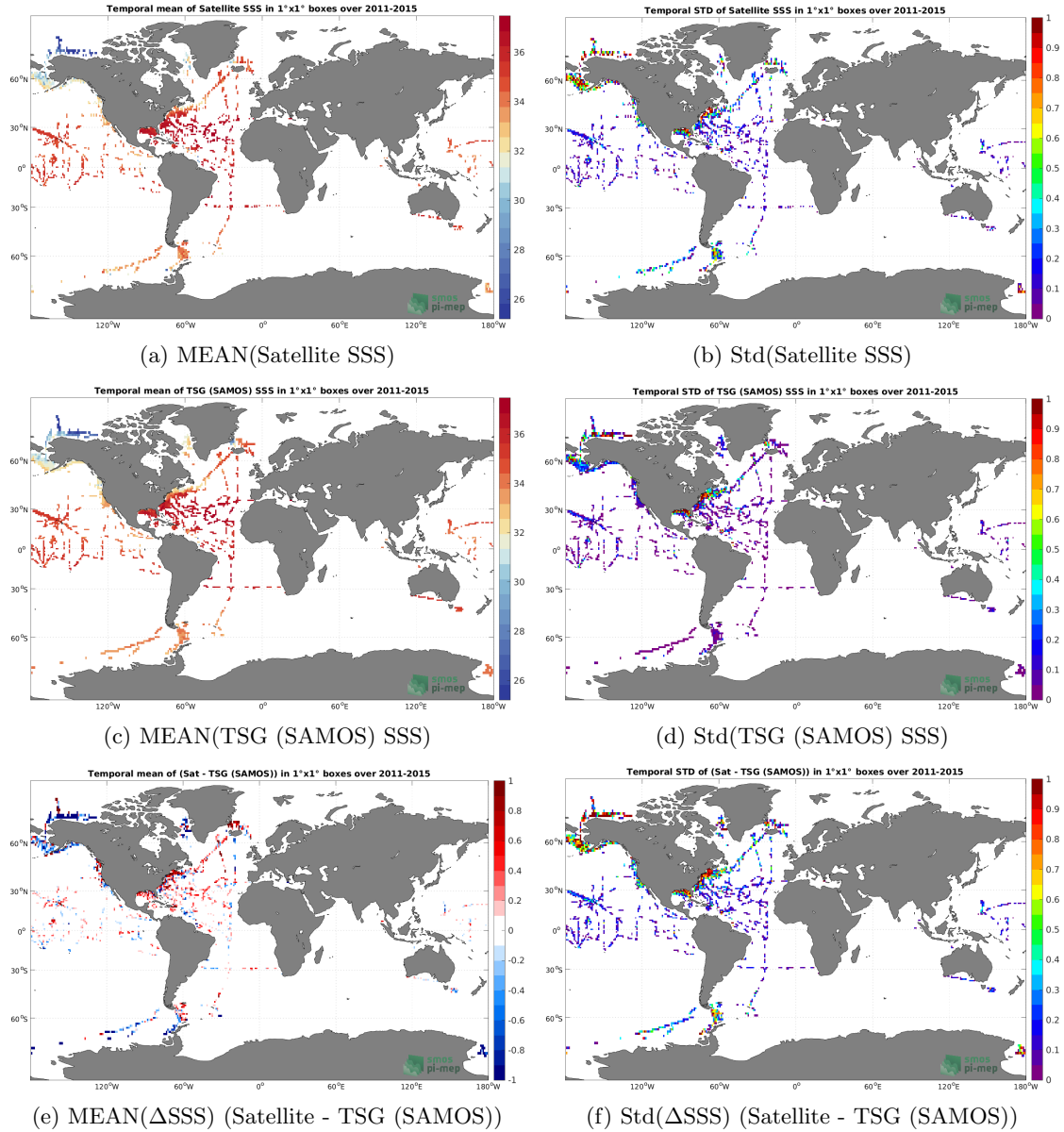
Figure 6: Temporal mean (left) and Std (right) of SSS from Aquarius SSS L2 OR v5 (NASA-GSFC) (top), TSG (SAMOS) (middle), and of \Delta SSS (Satellite - TSG (SAMOS)). Only match-up pairs are used to generate these maps.
