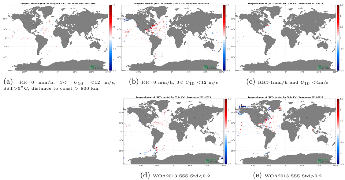
Figure 12: Temporal mean gridded over spatial boxes of size 1^\circ \times 1^\circ of \Delta SSS (Aquarius SSS L2 OR v5 (NASA-GSFC) - TSG (SAMOS)) for 5 different subdatasets corresponding to:RR=0 mm/h, 3 < U_{10} < 12 m/s, SST > 5^\circ\text{C} , distance to coast > 800 km (a), RR=0 mm/h, 3 < U_{10} < 12 m/s (b), RR > 1 mm/h and U_{10} < 4 m/s (c), WOA2013 SSS Std < 0.2 (d), WOA2013 SSS Std > 0.2 (e).
