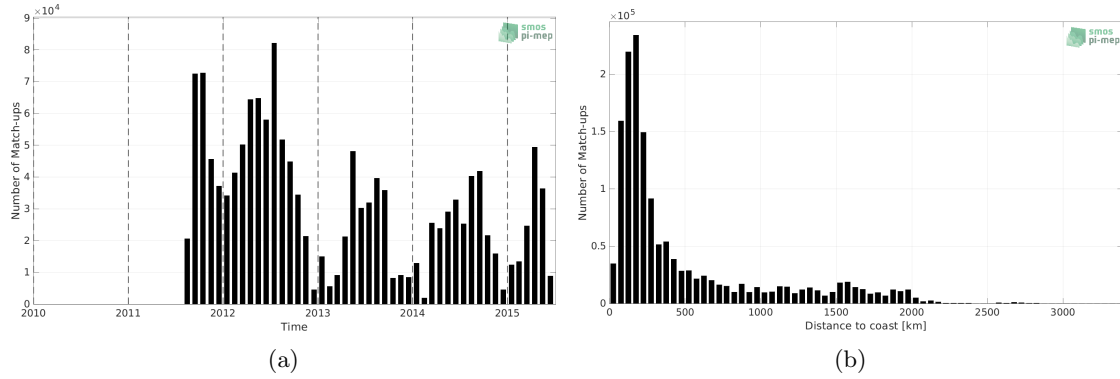
Figure 1: Number of match-ups between TSG (SAMOS) and Aquarius SSS L2 OR v5 (NASA-GSFC) SSS as a function of time (a) and as function of the distance to coast (b) over the Global Ocean Pi-MEP region and for the full satellite product period.
