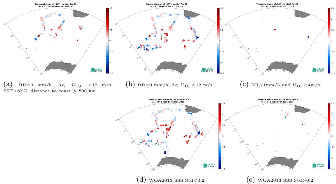
Figure 12: Temporal mean gridded over spatial boxes of size 1^\circ \times 1^\circ of \Delta SSS (Aquarius SSS L2 OR v5 (NASA-GSFC) - TSG (NCEI-0170743)) for 5 different subdatasets corresponding to:RR=0 mm/h, 3 < U_{10} < 12 m/s, SST >5^\circ C, distance to coast > 800 km (a), RR=0 mm/h, 3 < U_{10} < 12 m/s (b), RR >1 mm/h and U_{10} < 4 m/s (c), WOA2013 SSS Std <0.2 (d), WOA2013 SSS Std >0.2 (e).
