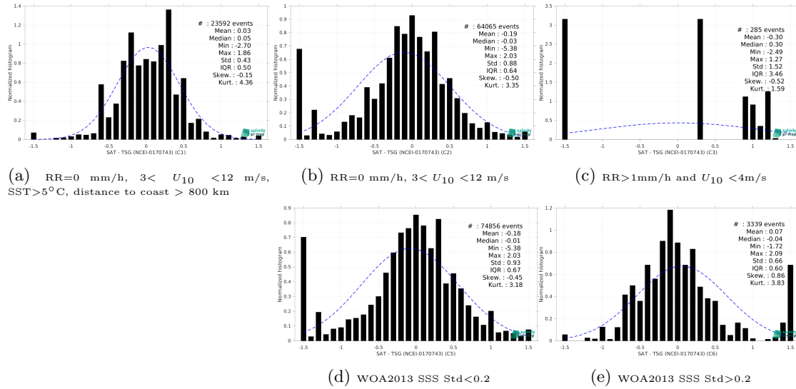
Figure 13: Normalized histogram of \Delta SSS (Aquarius SSS L2 OR v5 (NASA-GSFC) - TSG (NCEI-0170743)) for 5 different subdatasets corresponding to: RR=0 mm/h, 3 < U_{10} < 12 m/s, SST>5°C, distance to coast > 800 km (a), RR=0 mm/h, 3 < U_{10} < 12 m/s (b), RR>1mm/h and U_{10} < 4 m/s (c), WOA2013 SSS Std<0.2 (d), WOA2013 SSS Std>0.2 (e).
