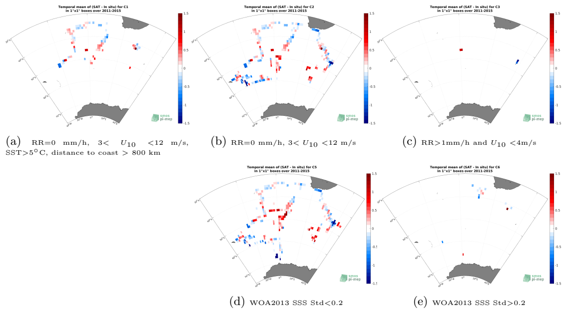
Figure 12: Temporal mean gridded over spatial boxes of size 1^\circ \times 1^\circ of \Delta SSS (Aquarius SSS L2 OR v5 (NASA-GSFC) - TSG (NCEI-0170743)) for 5 different subdatasets corresponding to: RR=0 mm/h, 3 < U_{10} < 12 m/s, SST >5^\circ\text{C} , distance to coast > 800 km (a), RR=0 mm/h, 3 < U_{10} < 12 m/s (b), RR >1 mm/h and U_{10} < 4 m/s (c), WOA2013 SSS Std <0.2 (d), WOA2013 SSS Std >0.2 (e).
