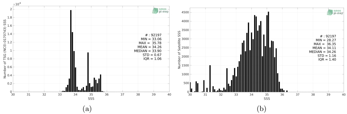
Figure 2: Histograms of SSS from TSG (NCEI-0170743) (a) and Aquarius SSS L2 OR v5 (NASA-GSFC) (b) considering all match-up pairs per bins of 0.1 over the Global Ocean Pi-MEP region and for the full satellite product period.
