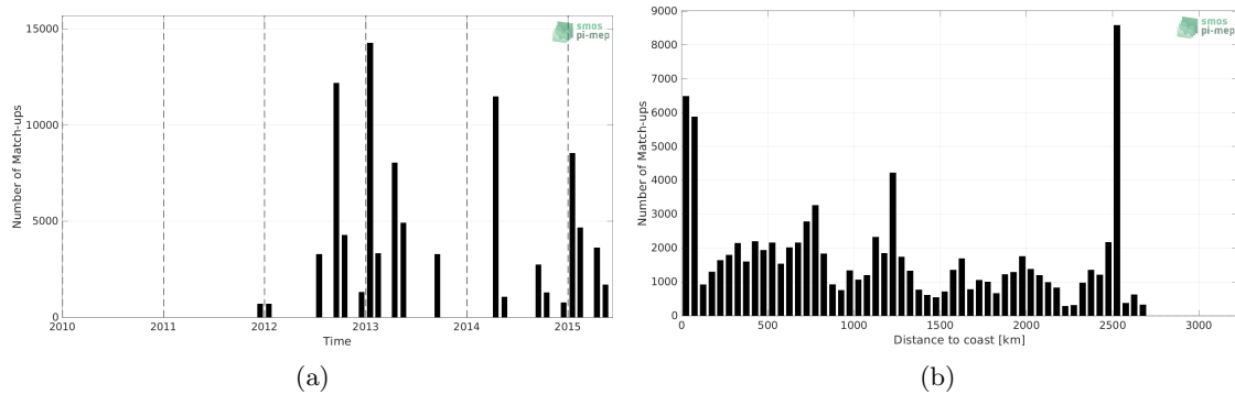
Figure 1: Number of match-ups between TSG (NCEI-0170743) and Aquarius SSS L2 OR v5 (NASA-GSFC) SSS as a function of time (a) and as function of the distance to coast (b) over the Global Ocean Pi-MEP region and for the full satellite product period.
