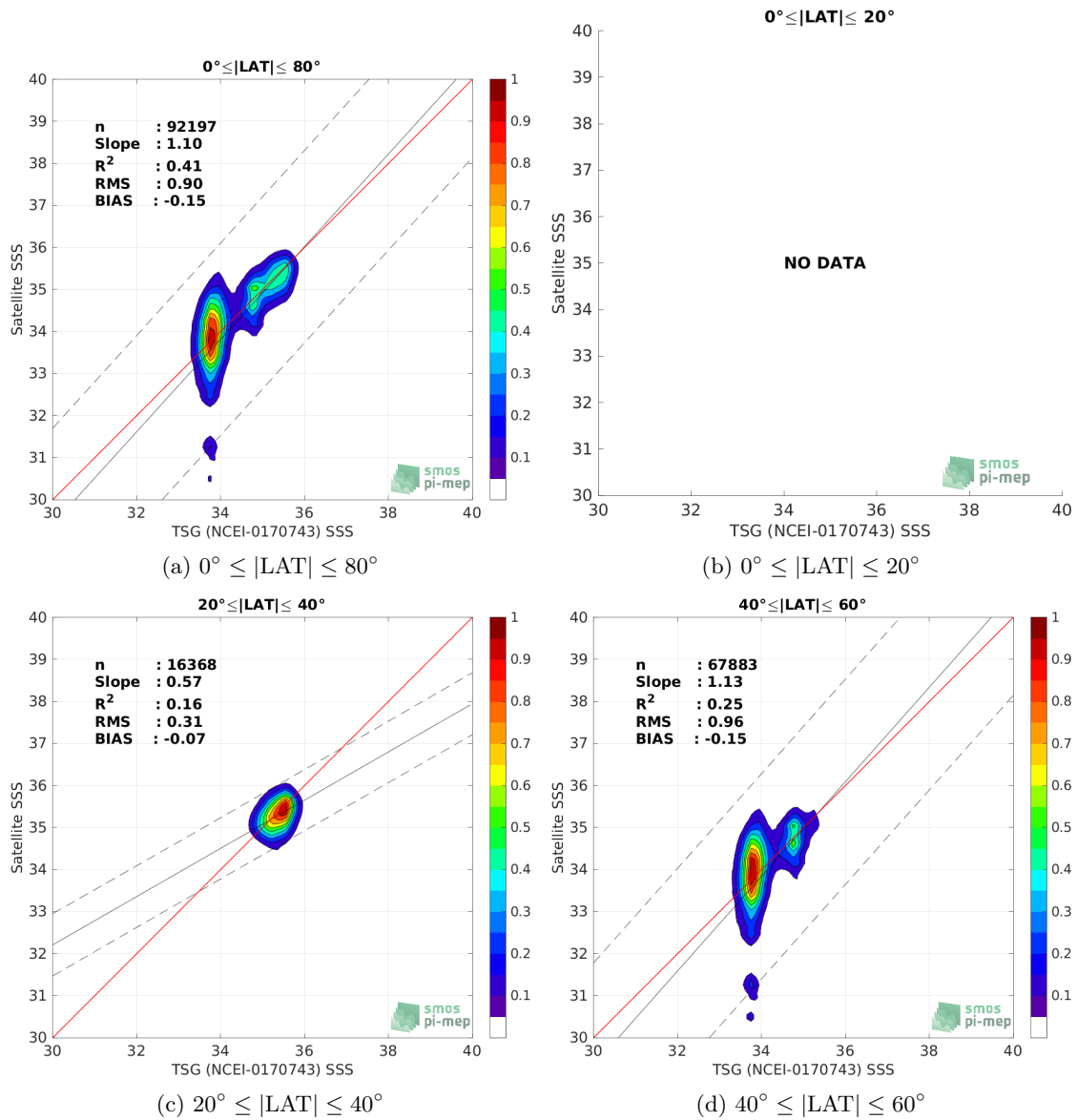
Figure 9: Contour maps of the concentration of Aquarius SSS L2 OR v5 (NASA-GSFC) SSS (y-axis) versus TSG (NCEI-0170743) SSS (x-axis) at match-up pairs for different latitude bands. For each plot, the red line shows x=y . The black thin and dashed lines indicate a linear fit through the data cloud and the \pm 95\% confidence levels, respectively. The number match-up pairs n , the slope and R^2 coefficient of the linear fit, the root mean square (RMS) and the mean bias between satellite and in situ data are indicated for each latitude band in each plots.
