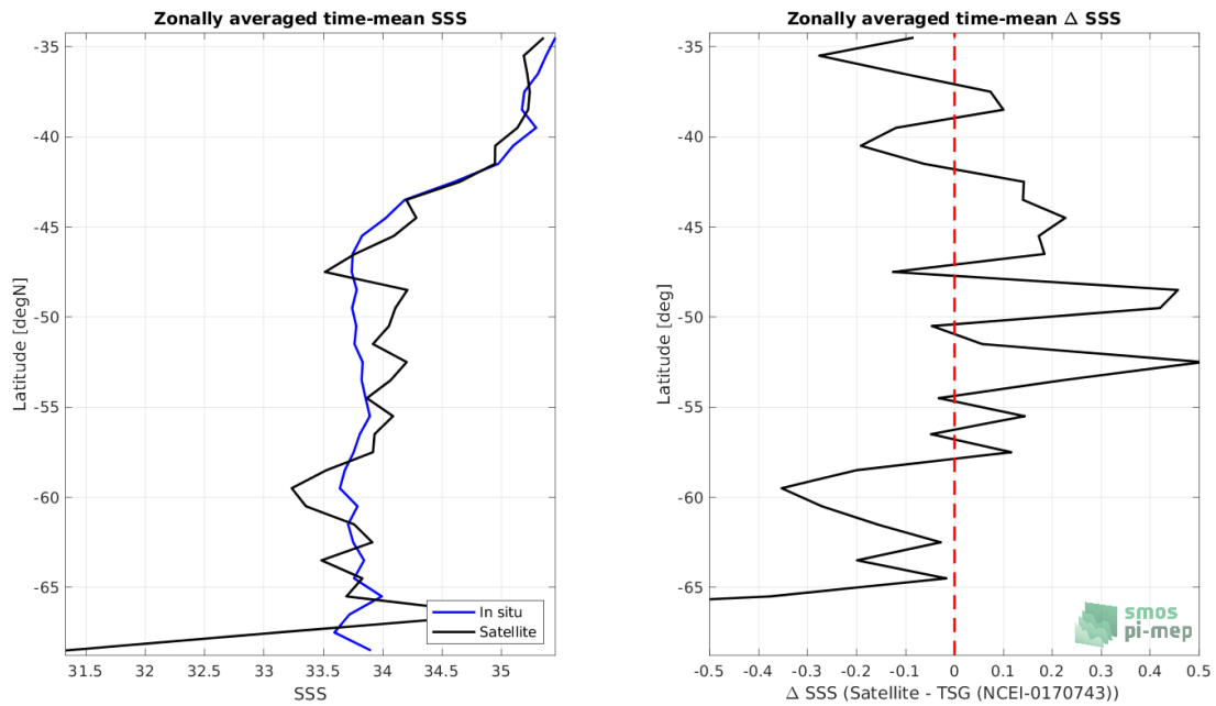
Figure 8: Left panel: Zonal mean SSS from Aquarius SSS L2 OR v5 (NASA-GSFC) satellite product (black) and from TSG (NCEI-0170743) (blue). Right panel: Zonal mean of \Delta SSS (Satellite - TSG (NCEI-0170743)) for all the collected Pi-MEP match-up pairs estimated over the full satellite product period.
