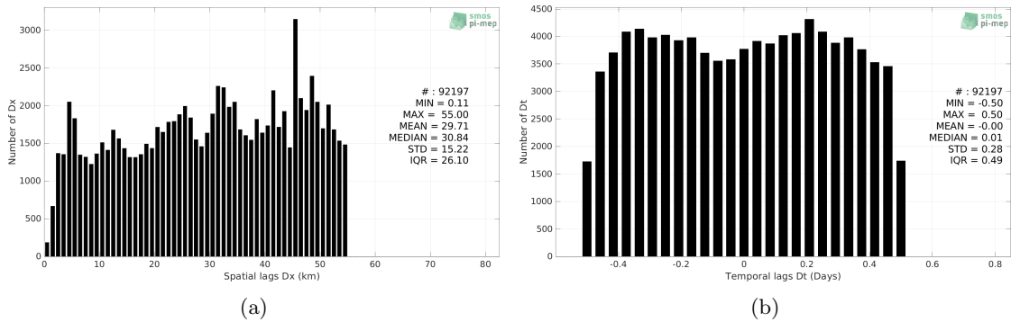
Figure 5: Histograms of the spatial (a) and temporal (b) lags between the location/time of the TSG (NCEI-0170743) measurement and the date of the corresponding Aquarius SSS L2 OR v5 (NASA-GSFC) SSS pixel.
