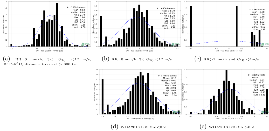
Figure 13: Normalized histogram of \Delta SSS (Aquarius SSS L2 OR v5 (NASA-GSFC) - TSG (NCEI-0170743)) for 5 different subdatasets corresponding to: RR=0 mm/h, 3 < U_{10} < 12 m/s, SST > 5°C, distance to coast > 800 km (a), RR=0 mm/h, 3 < U_{10} < 12 m/s (b), RR > 1mm/h and U_{10} < 4 m/s (c), WOA2013 SSS Std < 0.2 (d), WOA2013 SSS Std > 0.2 (e).
