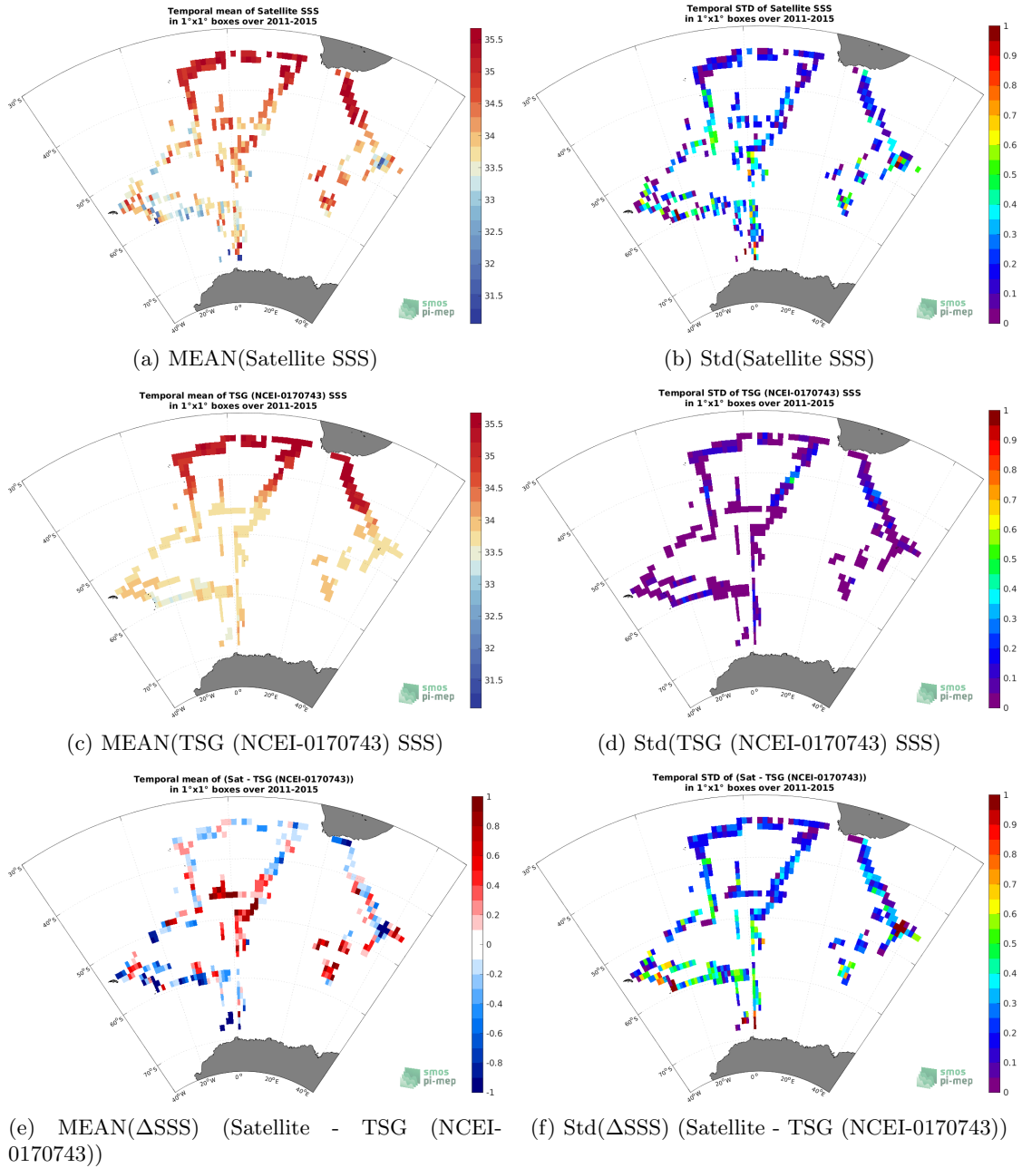
Figure 6: Temporal mean (left) and Std (right) of SSS from Aquarius SSS L2 OR v5 (NASA-GSFC) (top), TSG (NCEI-0170743) (middle), and of \Delta SSS (Satellite - TSG (NCEI-0170743)). Only match-up pairs are used to generate these maps.
