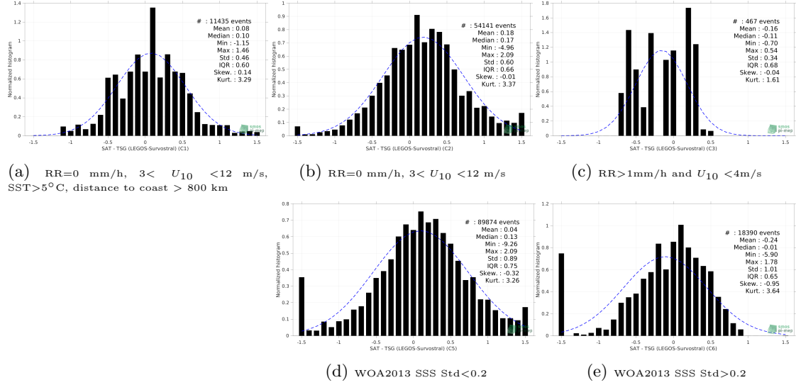
Figure 13: Normalized histogram of \Delta SSS (Aquarius SSS L2 OR v5 (NASA-GSFC) - TSG (LEGOS-Survostral)) for 5 different subdatasets corresponding to: RR=0 mm/h, 3 < U_{10} < 12 m/s, SST > 5°C, distance to coast > 800 km (a), RR=0 mm/h, 3 < U_{10} < 12 m/s (b), RR > 1mm/h and U_{10} < 4 m/s (c), WOA2013 SSS Std < 0.2 (d), WOA2013 SSS Std > 0.2 (e).
