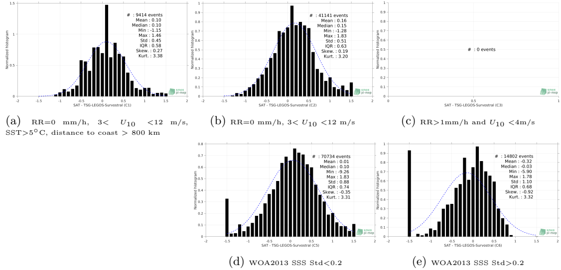
Figure 13: Normalized histogram of \Delta SSS (Aquarius-L2-OR-V5 - TSG-LEGOS-Survostral) for 5 different subdatasets corresponding to: RR=0 mm/h, 3 < U_{10} < 12 m/s, SST>5°C, distance to coast > 800 km (a), RR=0 mm/h, 3 < U_{10} < 12 m/s (b), RR>1mm/h and U_{10} < 4 m/s (c), WOA2013 SSS Std<0.2 (d), WOA2013 SSS Std>0.2 (e).
