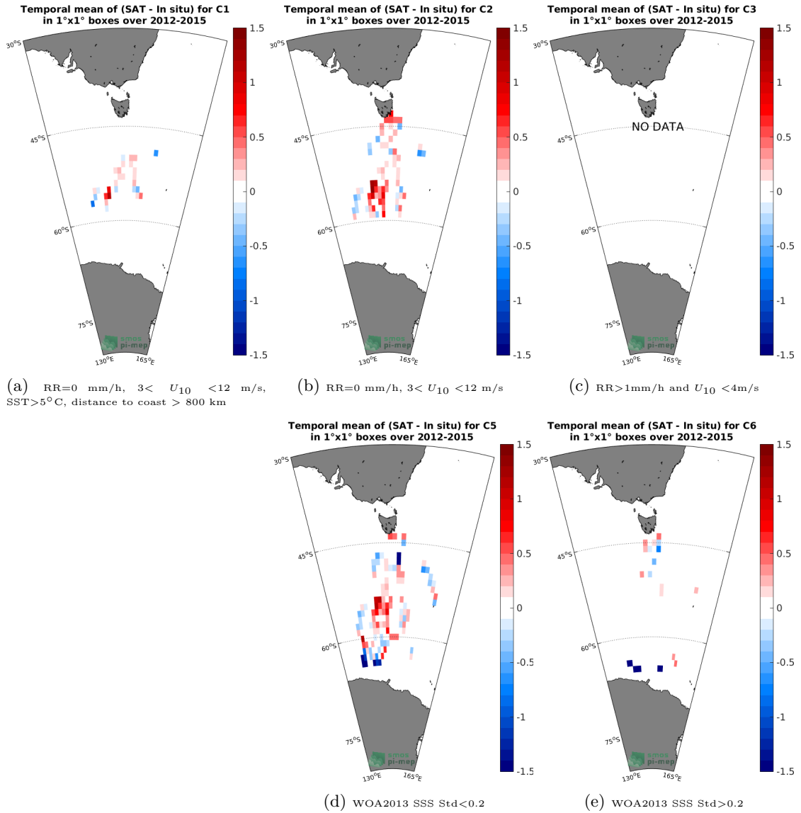
Figure 12: Temporal mean gridded over spatial boxes of size 1°x1° of \Delta SSS (Aquarius-L2-OR-V5 - TSG-LEGOS-Survostral) for 5 different subdatasets corresponding to: RR=0 mm/h, 3 < U_{10} < 12 m/s, SST > 5°C, distance to coast > 800 km (a), RR=0 mm/h, 3 < U_{10} < 12 m/s (b), RR > 1mm/h and U_{10} < 4 m/s (c), WOA2013 SSS Std < 0.2 (d), WOA2013 SSS Std > 0.2 (e).
