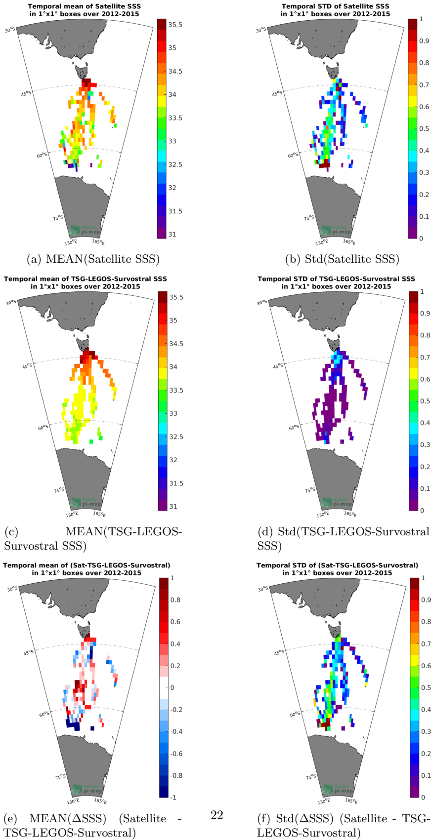
Figure 6: Temporal mean (left) and Std (right) of SSS from Aquarius-L2-OR-V5 (top), TSG-LEGOS-Survostral (middle), and of \Delta SSS (Satellite - TSG-LEGOS-Survostral). Only match-up pairs are used to generate these maps.
