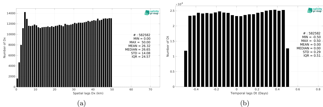
Figure 6: Histograms of the spatial (a) and temporal (b) lags between the location/time of the TSG (LEGOS-DM) measurement and the date of the corresponding Aquarius SSS L2 OR v5 (NASA-GSFC) SSS pixel.
