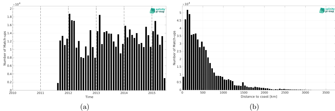
Figure 2: Number of match-ups between TSG (LEGOS-DM) and Aquarius SSS L2 OR v5 (NASA-GSFC) SSS as a function of time (a) and as function of the distance to coast (b) over the Global Ocean Pi-MEP region and for the full satellite product period.
