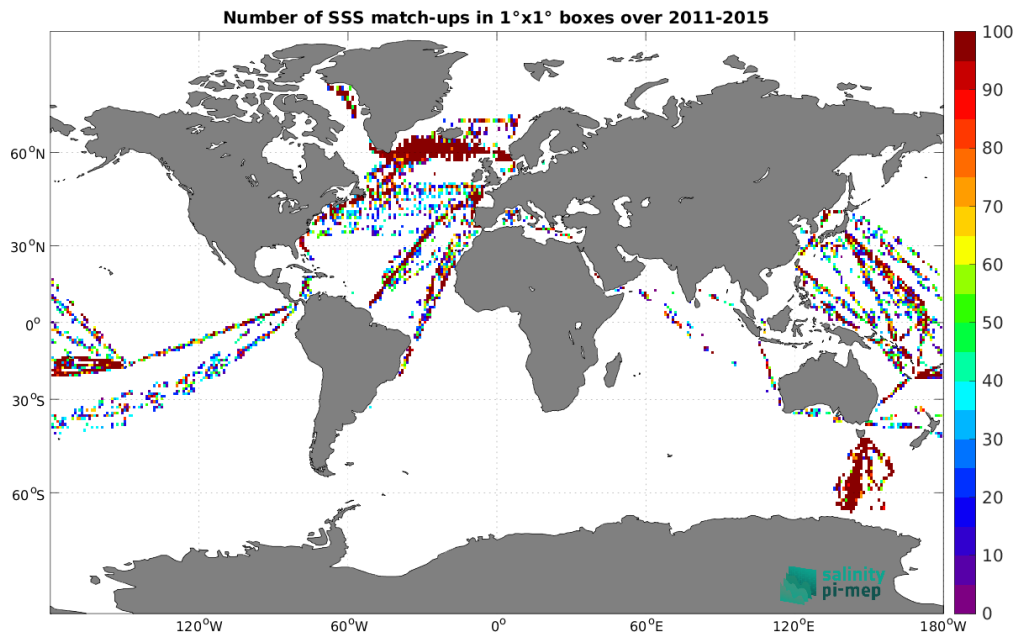
Figure 5: Number of SSS match-ups between TSG (LEGOS-DM) SSS and the Aquarius SSS L2 OR v5 (NASA-GSFC) SSS product for the Global Ocean Pi-MEP region over 1^\circ \times 1^\circ boxes and for the full satellite product period.
