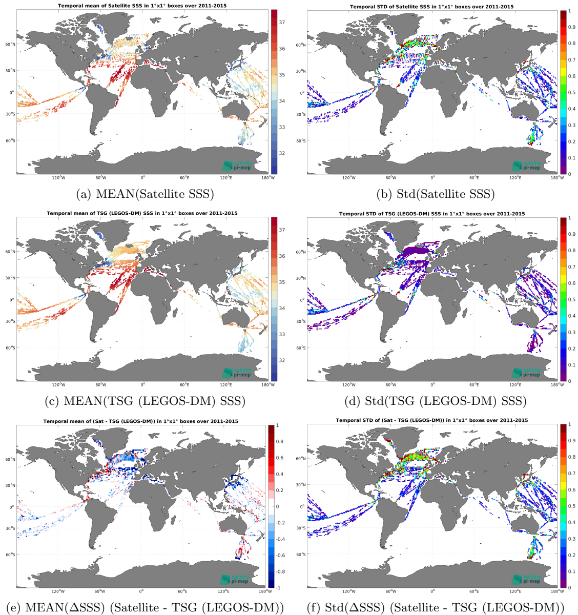
Figure 7: Temporal mean (left) and Std (right) of SSS from Aquarius SSS L2 OR v5 (NASA-GSFC) (top), TSG (LEGOS-DM) (middle), and of \Delta SSS (Satellite - TSG (LEGOS-DM)). Only match-up pairs are used to generate these maps.
