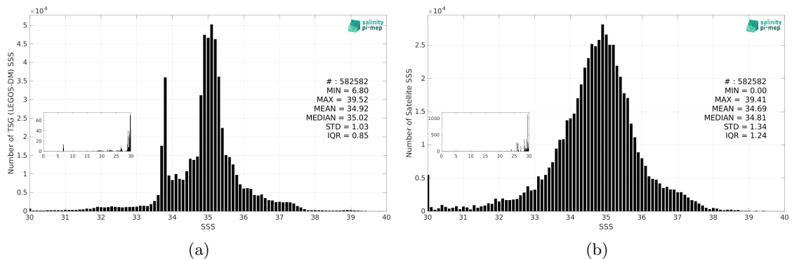
Figure 3: Histograms of SSS from TSG (LEGOS-DM) (a) and Aquarius SSS L2 OR v5 (NASA-GSFC) (b) considering all match-up pairs per bins of 0.1 over the Global Ocean Pi-MEP region and for the full satellite product period.
