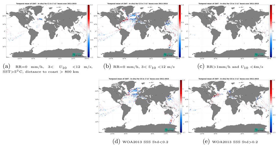
Figure 14: Temporal mean gridded over spatial boxes of size 1^\circ \times 1^\circ of \Delta SSS (Aquarius SSS L2 OR v5 (NASA-GSFC) - TSG (LEGOS-DM)) for 5 different subdatasets corresponding to:RR=0 mm/h, 3 < U_{10} < 12 m/s, SST > 5^\circ\text{C} , distance to coast > 800 km (a), RR=0 mm/h, 3 < U_{10} < 12 m/s (b), RR > 1 mm/h and U_{10} < 4 m/s (c), WOA2013 SSS Std < 0.2 (d), WOA2013 SSS Std > 0.2 (e).
