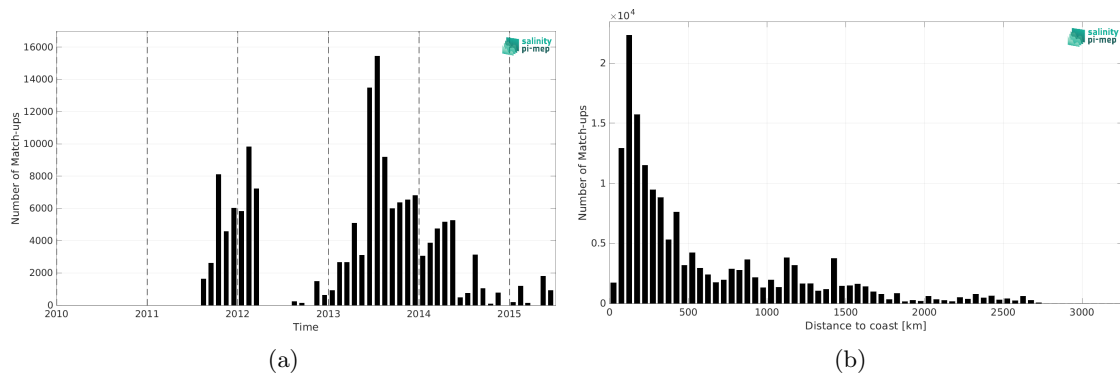
Figure 2: Number of match-ups between TSG (GOSUD-Sailing-ship) and Aquarius SSS L2 OR v5 (NASA-GSFC) SSS as a function of time (a) and as function of the distance to coast (b) over the Global Ocean Pi-MEP region and for the full satellite product period.
