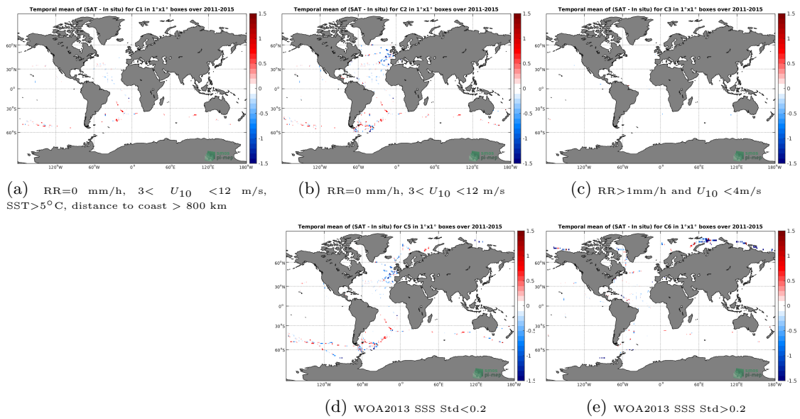
Figure 12: Temporal mean gridded over spatial boxes of size 1^\circ \times 1^\circ of \Delta SSS (Aquarius-L2-OR-V5 - TSG-GOSUD-Sailing-ship) for 5 different subdatasets corresponding to:RR=0 mm/h, 3 < U_{10} < 12 m/s, SST > 5°C, distance to coast > 800 km (a), RR=0 mm/h, 3 < U_{10} < 12 m/s (b), RR > 1mm/h and U_{10} < 4 m/s (c), WOA2013 SSS Std < 0.2 (d), WOA2013 SSS Std > 0.2 (e).
