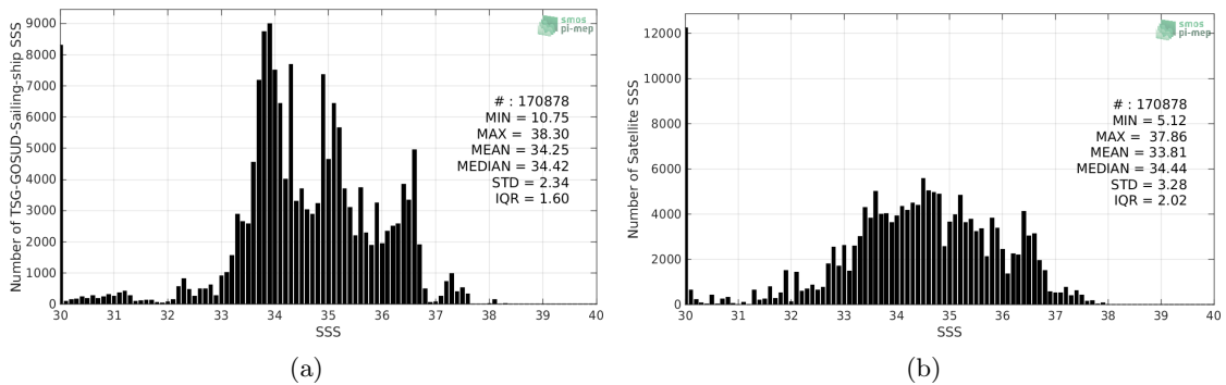
Figure 2: Histograms of SSS from TSG-GOSUD-Sailing-ship (a) and Aquarius-L2-OR-V5 (b) considering all match-up pairs per bins of 0.1 over the Global Ocean Pi-MEP region and for the full satellite product period.
