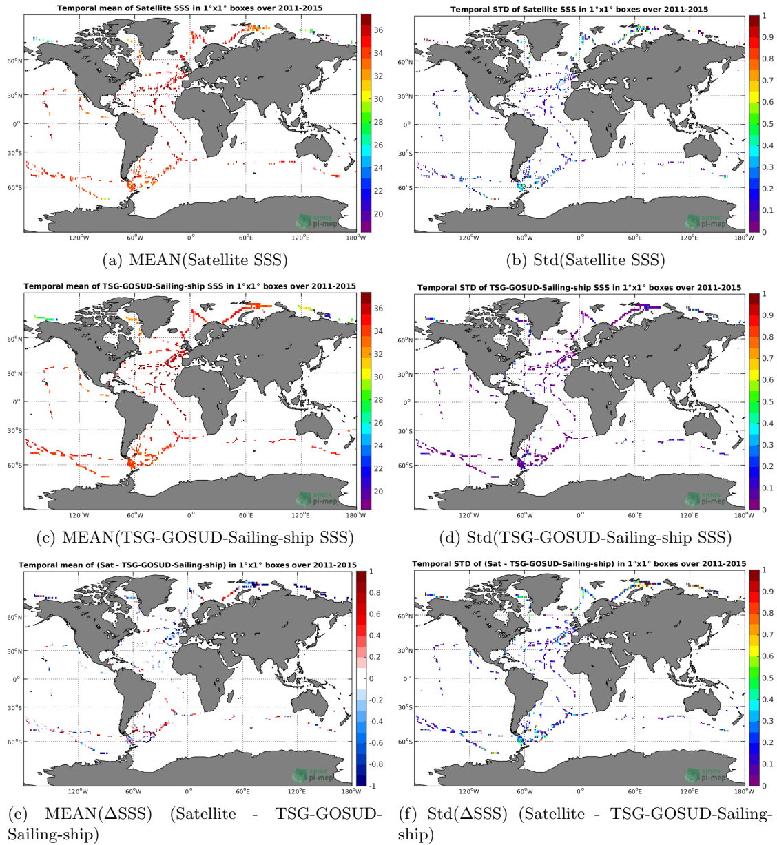
Figure 6: Temporal mean (left) and Std (right) of SSS from Aquarius-L2-OR-V5 (top), TSG-GOSUD-Sailing-ship (middle), and of \Delta SSS (Satellite - TSG-GOSUD-Sailing-ship). Only match-up pairs are used to generate these maps.
