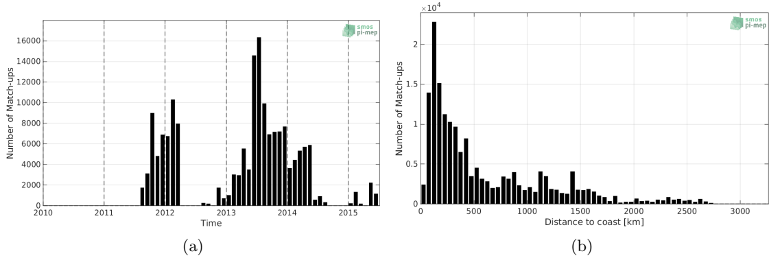
Figure 1: Number of match-ups between TSG-GOSUD-Sailing-ship and Aquarius-L2-OR-V5 SSS as a function of time (a) and as function of the distance to coast (b) over the Global Ocean Pi-MEP region and for the full satellite product period.
