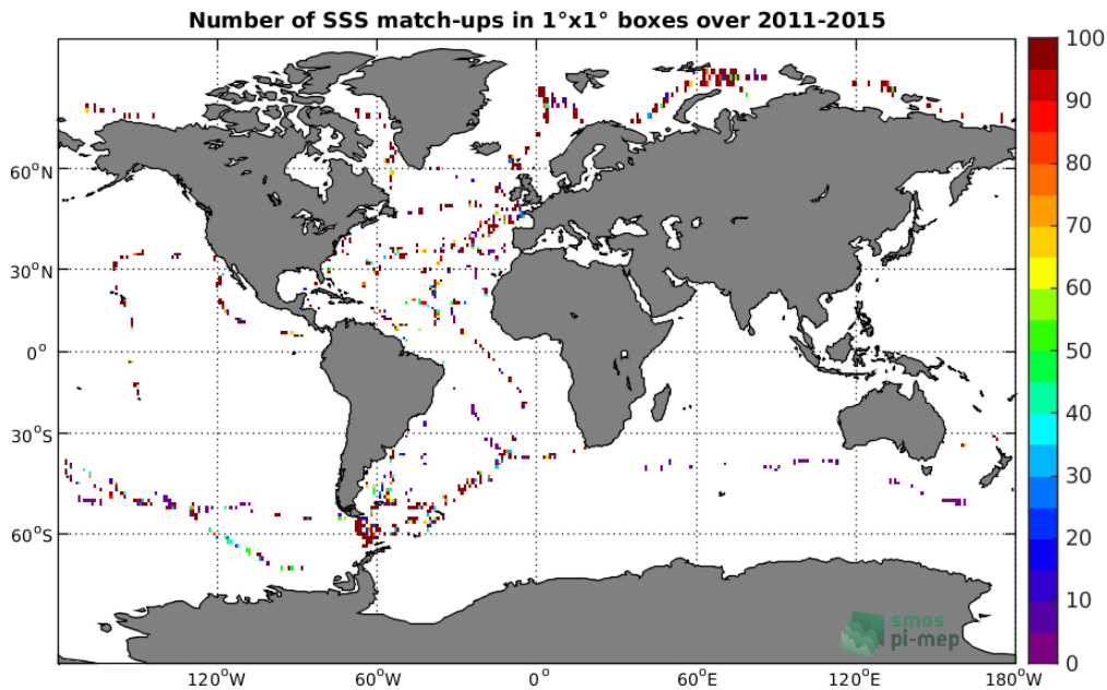
Figure 4: Number of SSS match-ups between TSG-GOSUD-Sailing-ship SSS and the Aquarius-L2-OR-V5 SSS product for the Global Ocean Pi-MEP region over 1^\circ \times 1^\circ boxes and for the full satellite product period.
