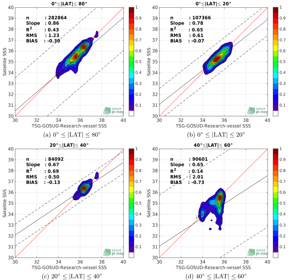
Figure 9: Contour maps of the concentration of Aquarius-L2-OR-V5 SSS (y-axis) versus TSG-GOSUD-Research-vessel SSS (x-axis) at match-up pairs for different latitude bands. For each plot, the red line shows x=y . The black thin and dashed lines indicate a linear fit through the data cloud and the \pm 95\% confidence levels, respectively. The number match-up pairs n , the slope and R^2 coefficient of the linear fit, the root mean square (RMS) and the mean bias between satellite and in situ data are indicated for each latitude band in each plots.
