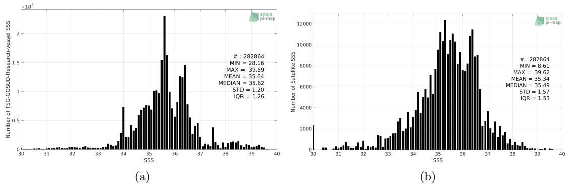
Figure 2: Histograms of SSS from TSG-GOSUD-Research-vessel (a) and Aquarius-L2-OR-V5 (b) considering all match-up pairs per bins of 0.1 over the Global Ocean Pi-MEP region and for the full satellite product period.
