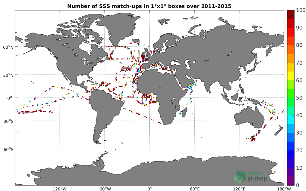
Figure 4: Number of SSS match-ups between TSG-GOSUD-Research-vessel SSS and the Aquarius-L2-OR-V5 SSS product for the Global Ocean Pi-MEP region over 1^\circ \times 1^\circ boxes and for the full satellite product period.
