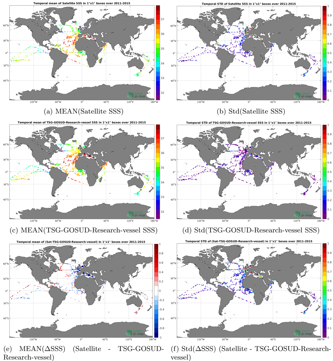
Figure 6: Temporal mean (left) and Std (right) of SSS from Aquarius-L2-OR-V5 (top), TSG-GOSUD-Research-vessel (middle), and of \Delta SSS (Satellite - TSG-GOSUD-Research-vessel). Only match-up pairs are used to generate these maps.
