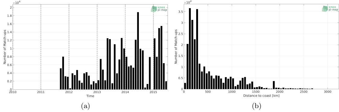
Figure 1: Number of match-ups between TSG-GOSUD-Research-vessel and Aquarius-L2-OR-V5 SSS as a function of time (a) and as function of the distance to coast (b) over the Global Ocean Pi-MEP region and for the full satellite product period.
