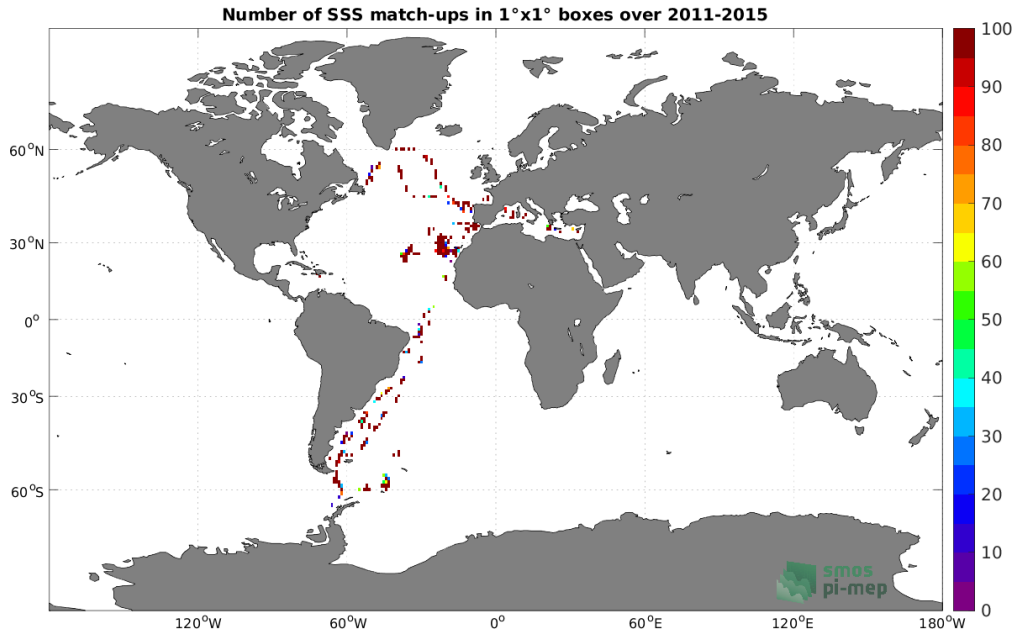
Figure 4: Number of SSS match-ups between TSG (CSIC-UTM) SSS and the Aquarius SSS L2 OR v5 (NASA-GSFC) SSS product for the Global Ocean Pi-MEP region over 1^\circ \times 1^\circ boxes and for the full satellite product period.
