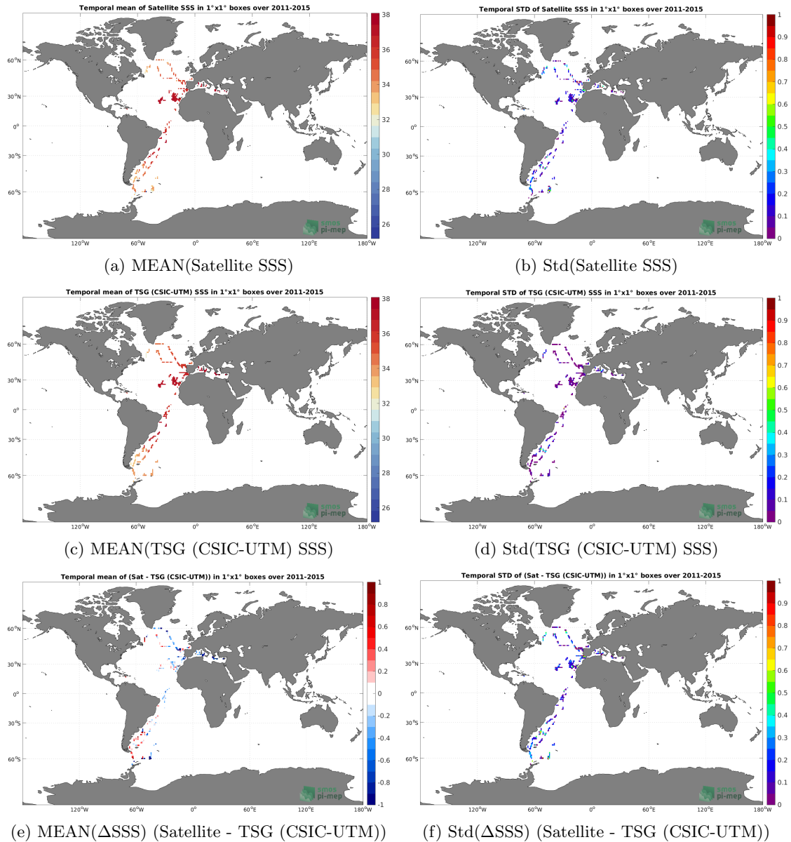
Figure 6: Temporal mean (left) and Std (right) of SSS from Aquarius SSS L2 OR v5 (NASA-GSFC) (top), TSG (CSIC-UTM) (middle), and of \Delta SSS (Satellite - TSG (CSIC-UTM)). Only match-up pairs are used to generate these maps.
