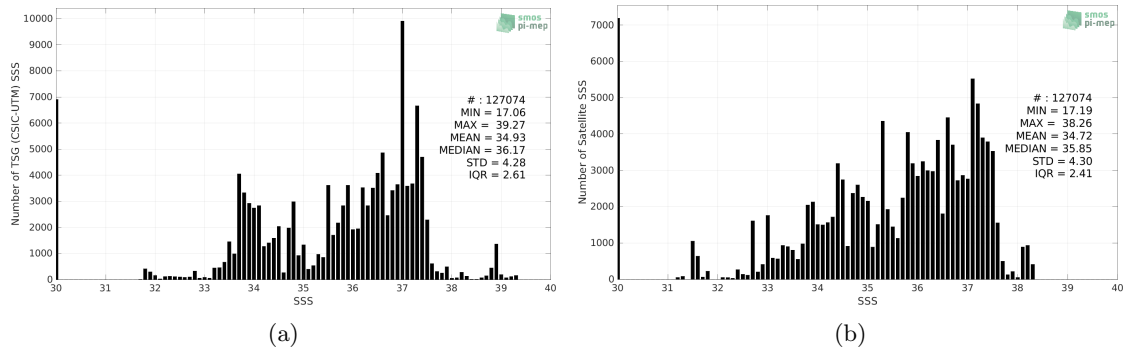
Figure 2: Histograms of SSS from TSG (CSIC-UTM) (a) and Aquarius SSS L2 OR v5 (NASA-GSFC) (b) considering all match-up pairs per bins of 0.1 over the Global Ocean Pi-MEP region and for the full satellite product period.
