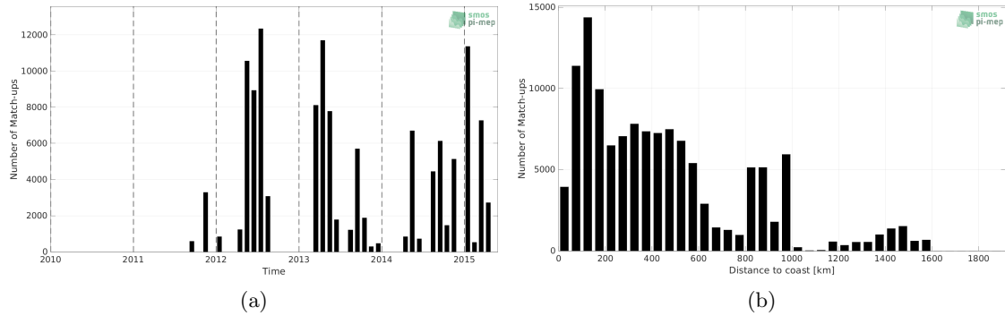
Figure 1: Number of match-ups between TSG (CSIC-UTM) and Aquarius SSS L2 OR v5 (NASA-GSFC) SSS as a function of time (a) and as function of the distance to coast (b) over the Global Ocean Pi-MEP region and for the full satellite product period.
