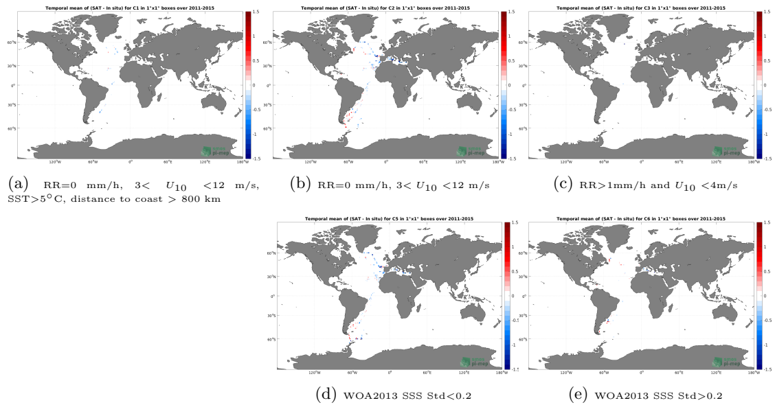
Figure 12: Temporal mean gridded over spatial boxes of size 1^\circ \times 1^\circ of \Delta SSS (Aquarius SSS L2 OR v5 (NASA-GSFC) - TSG (CSIC-UTM)) for 5 different subdatasets corresponding to:RR=0 mm/h, 3 < U_{10} < 12 m/s, SST > 5^\circ\text{C} , distance to coast > 800 km (a), RR=0 mm/h, 3 < U_{10} < 12 m/s (b), RR > 1 mm/h and U_{10} < 4 m/s (c), WOA2013 SSS Std < 0.2 (d), WOA2013 SSS Std > 0.2 (e).
